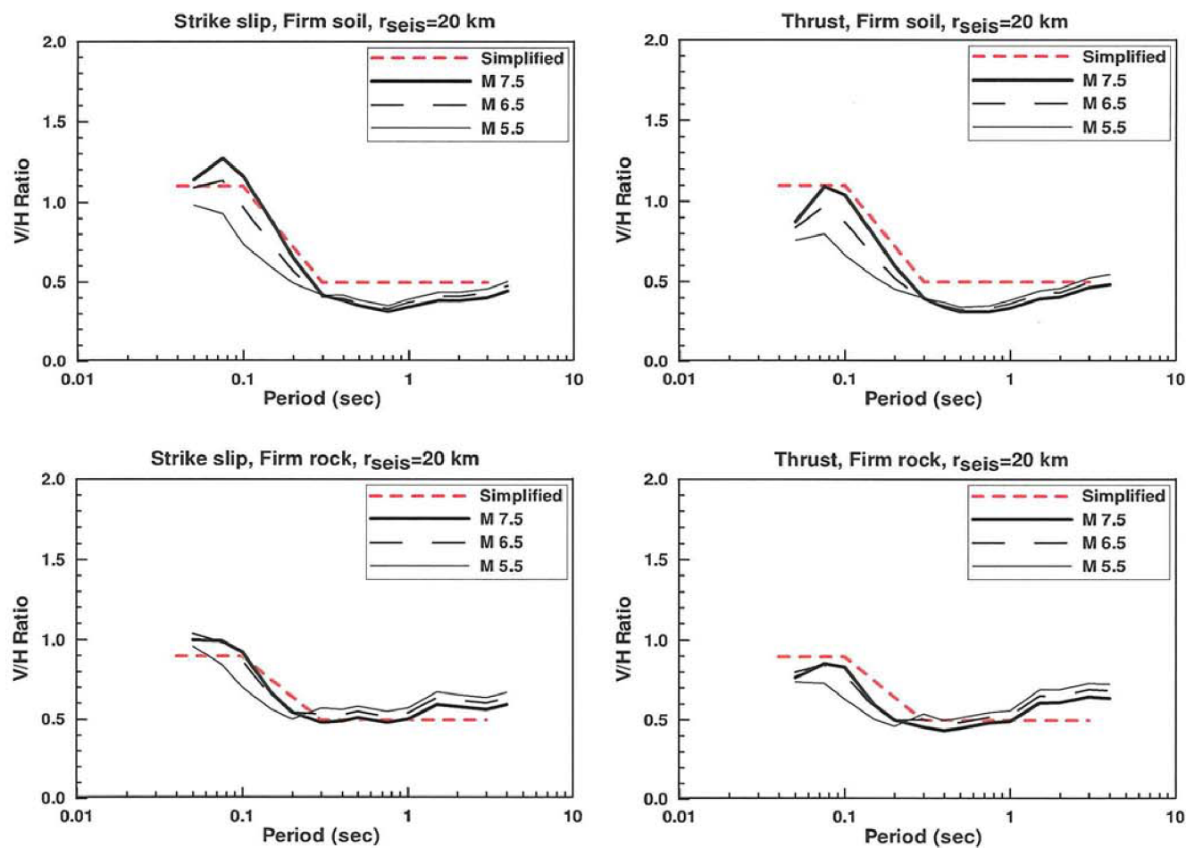
Fig. 9. Comparison of the simplified and predicted V/H response spectral ratios developed in this study for r_{\text{seis}} = 20 km and selected values of magnitude and local soil conditions.
