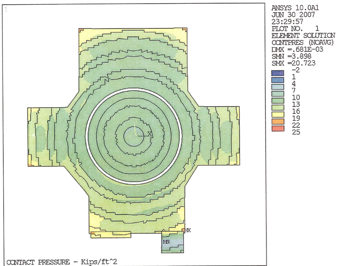
Figure 03.08.05-5-1—Static Bearing Pressure for Soil Condition 2sn4u
