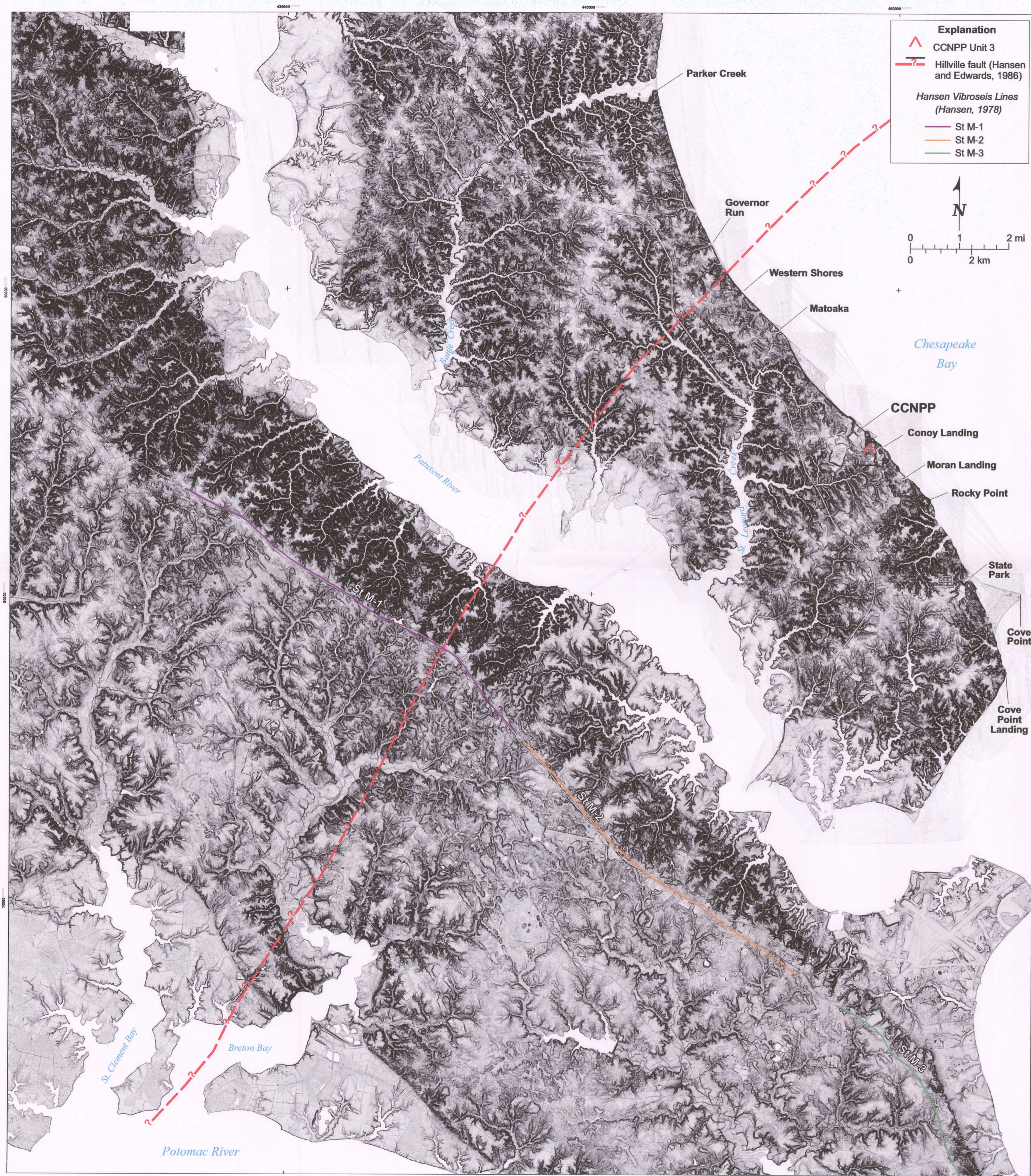
Figure 2. Slope Map of LIDAR data covering the extent of the Hillville fault, Calvert and St. Mary's Counties, Maryland.
