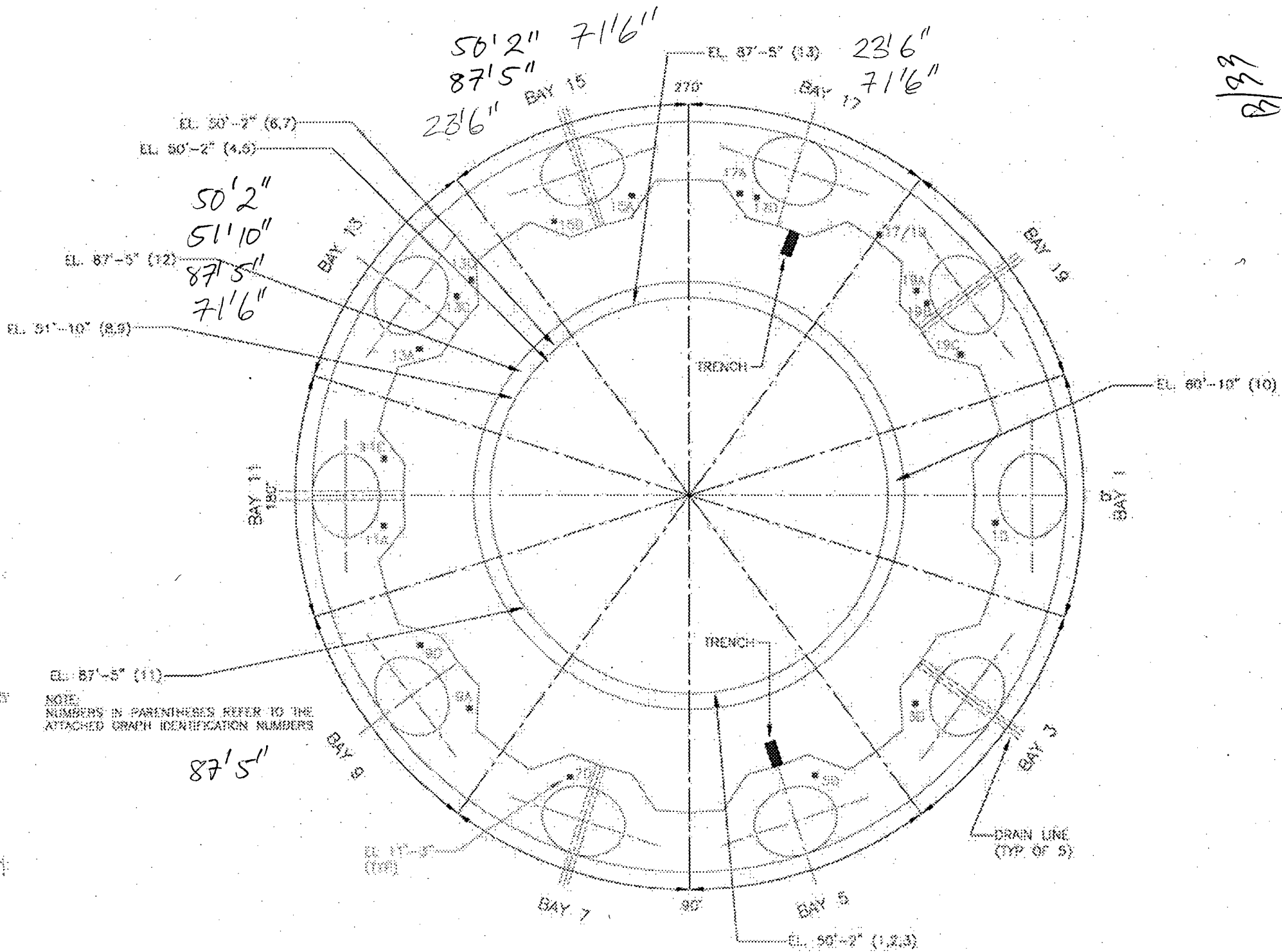
KEY PLAN
