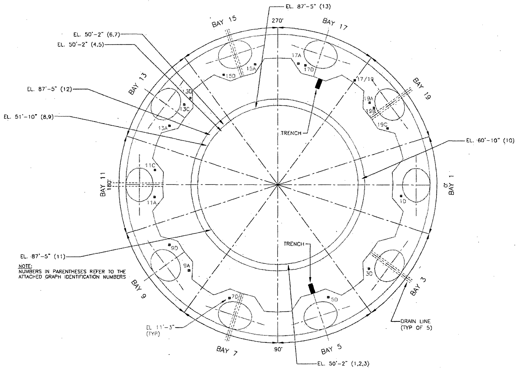
KEY PLAN
