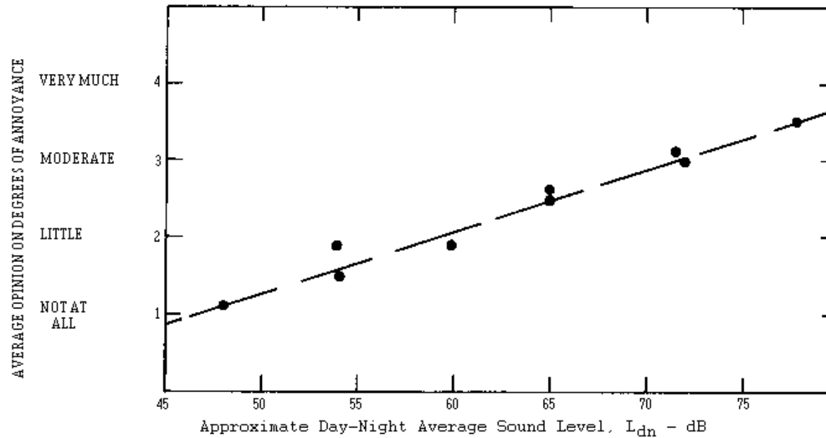
Level - Results of First London Heathrow Survey D-39 from D-6
