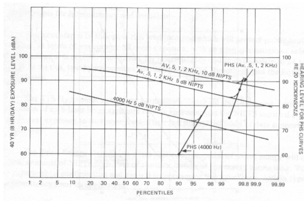
Figure C-4. Exposure Level and Hearing Level as a Function of Population Percent Showing Merging of
