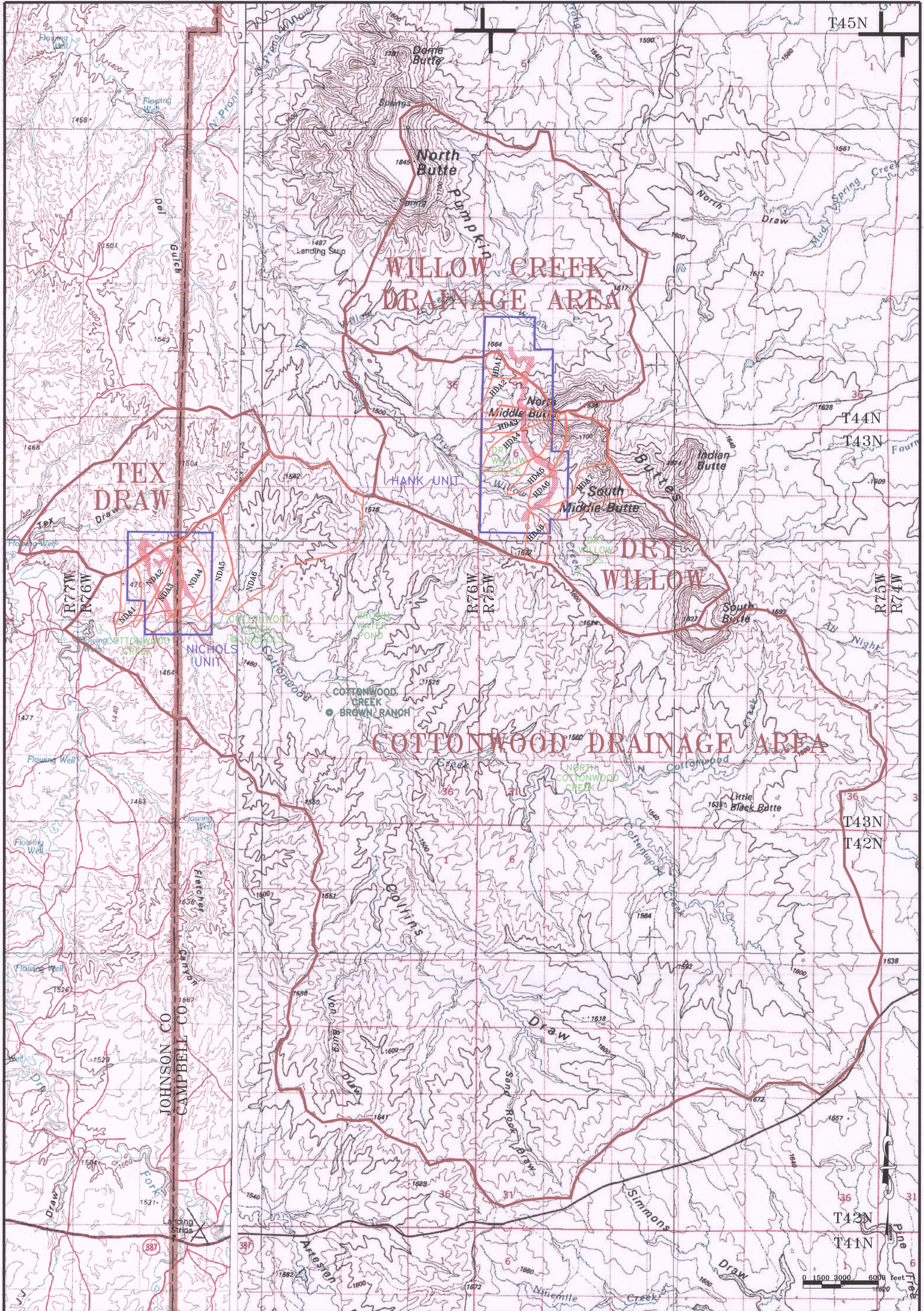
FIGURE D6-1. SURFACE DRAINAGE AREAS
