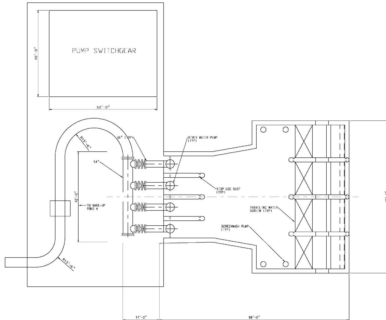
PLAN
