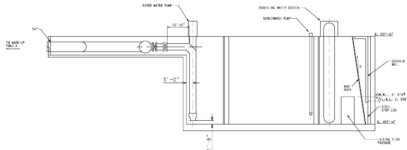
PROFILE
