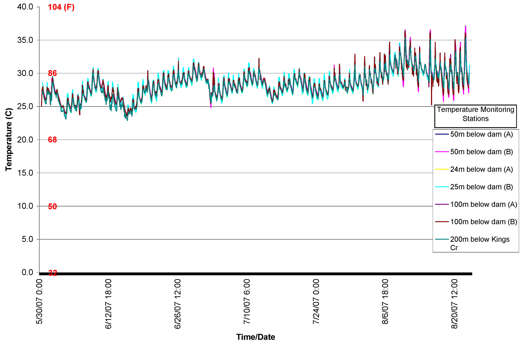
WILLIAM STATES LEE III NUCLEAR STATION UNITS 1 & 2 Ninety-Nine Islands Dam Discharge Water Temperature Hourly Readings for 2007 FIGURE 2.3-26 Rev 1
