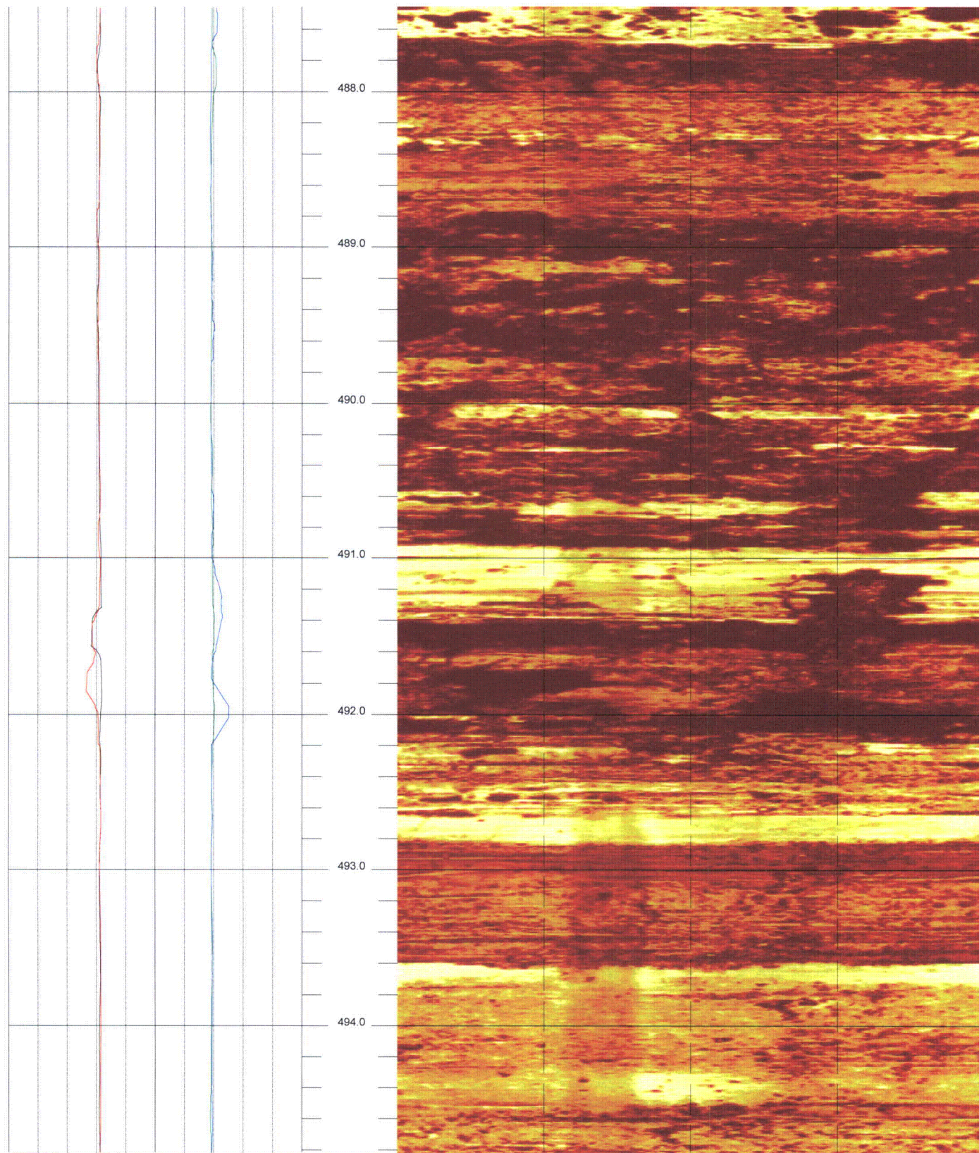
PEF - LNP COLA Boring AD-4 Acoustic Televiewer based Caliper rev 1 Sheet 39 of 40
