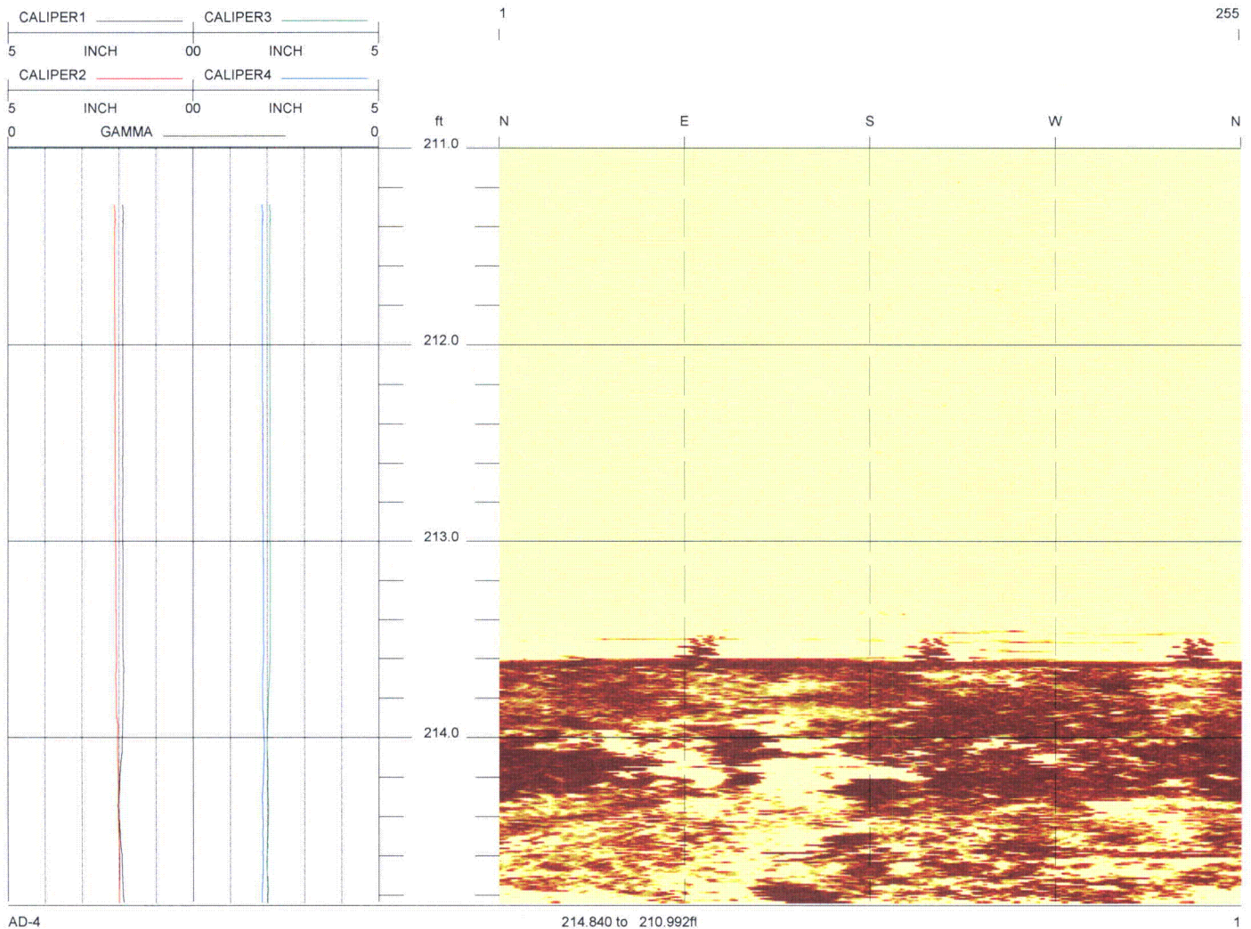
PEF - LNP COLA Boring AD-4 Acoustic Televiwer based Caliper rev 1 Sheet 1 of 40
