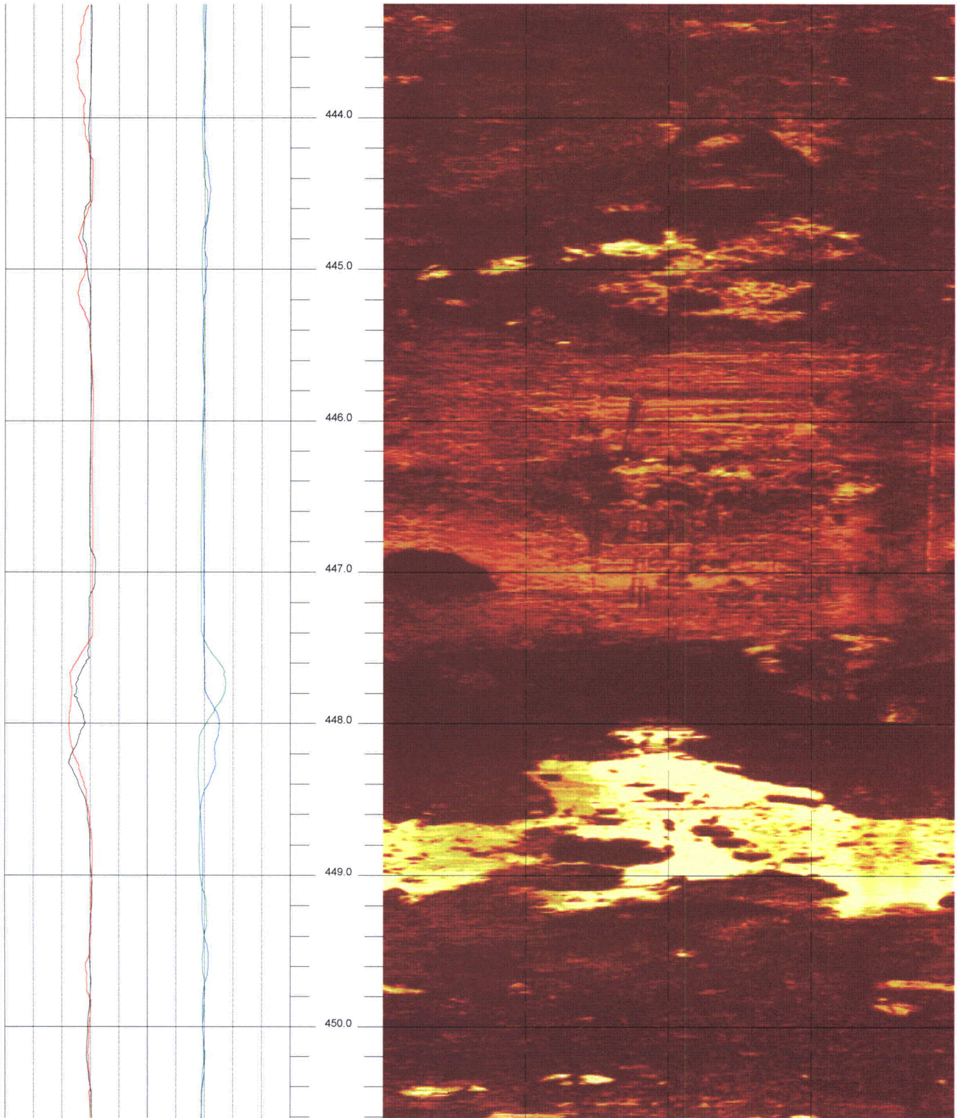
PEF - LNP COLA Boring AD-4 Acoustic Televiewer based Caliper rev 1 Sheet 33 of 40
