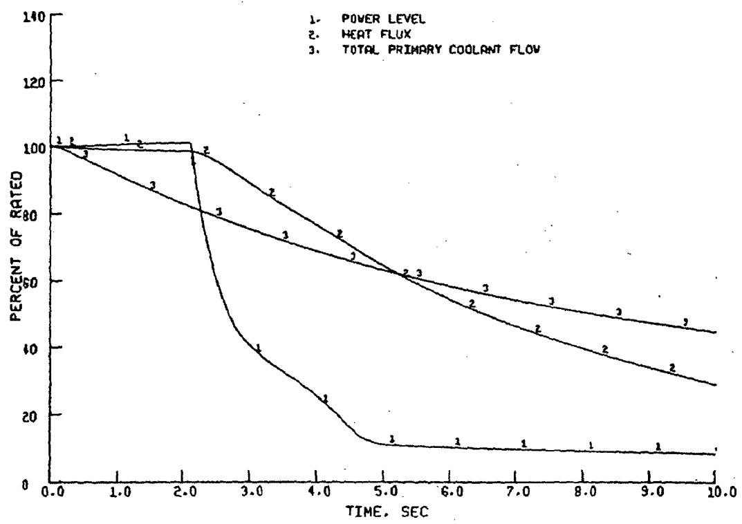
Figure 15.2.5-1 St. Lucie Unit 1 - Power, Heat Flux and Flow - Loss Of Coolant Flow
