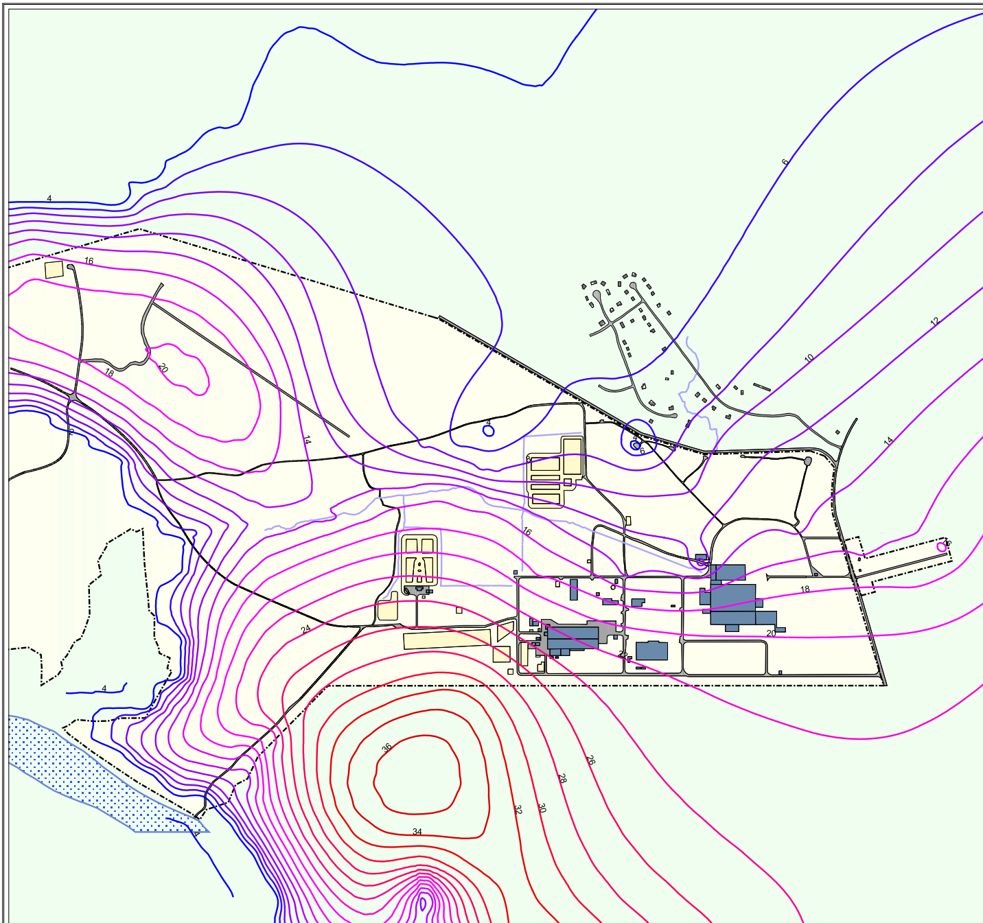
Figure P-18 Calibrated Groundwater Elevations – Site Area Nov 1998
