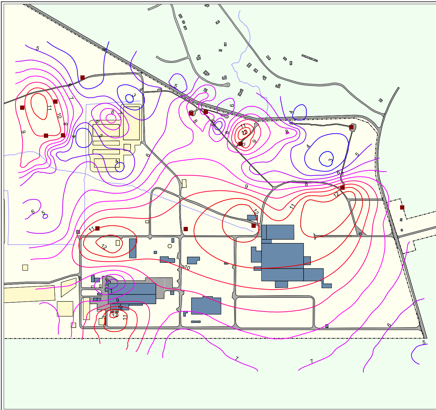
Figure P-6 Estimated Semiconfining- Layer Thickness
