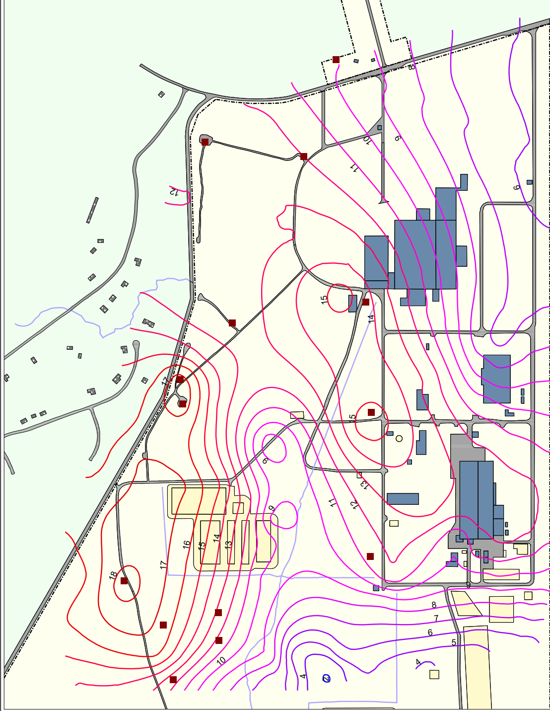
Figure P-5 Piezometric Head Difference Between the Surficial and Principal Aquifers (9/12/00)
