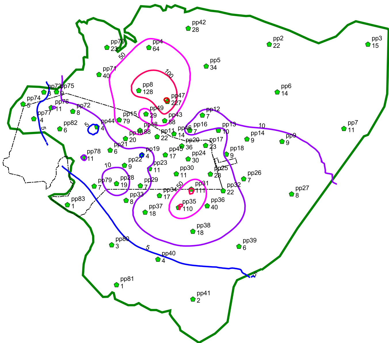
Figure P-13 Model Hydraulic Conductivity Distribution and Pilot Points Wilmington Site
