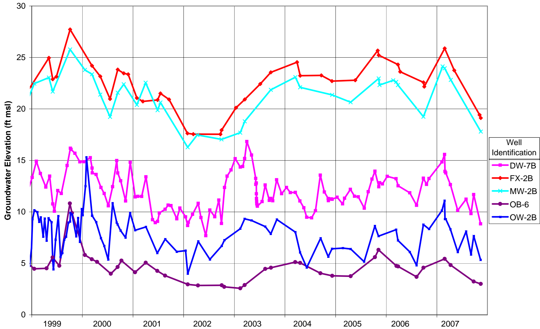
Figure 3.4-11. Example Principal Aquifer hydrographs.
