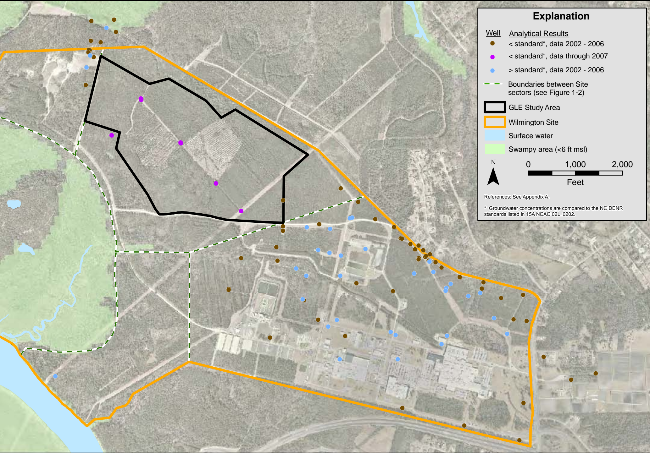
Figure 3.4-15. Summary of groundwater quality data – organic constituents.
