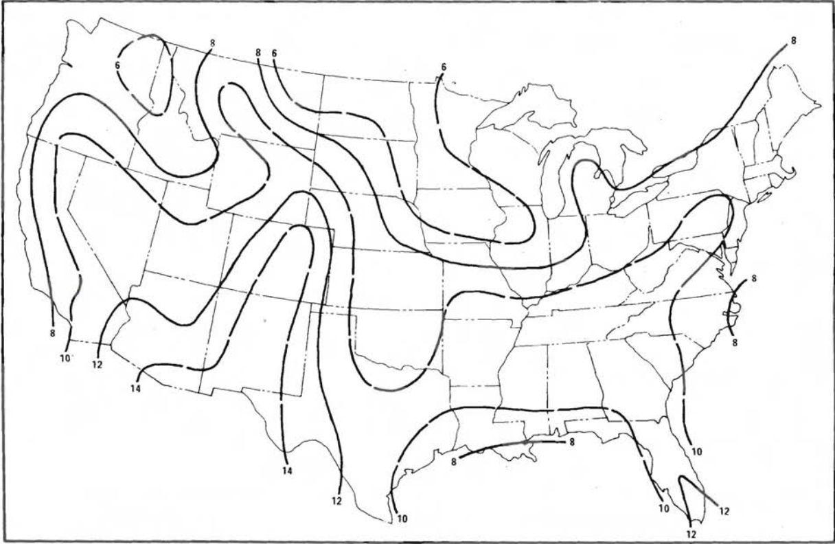
Figure 3.6-28. Mean afternoon mixing heights in winter for the continental United States ( m \times 10^2 ).
