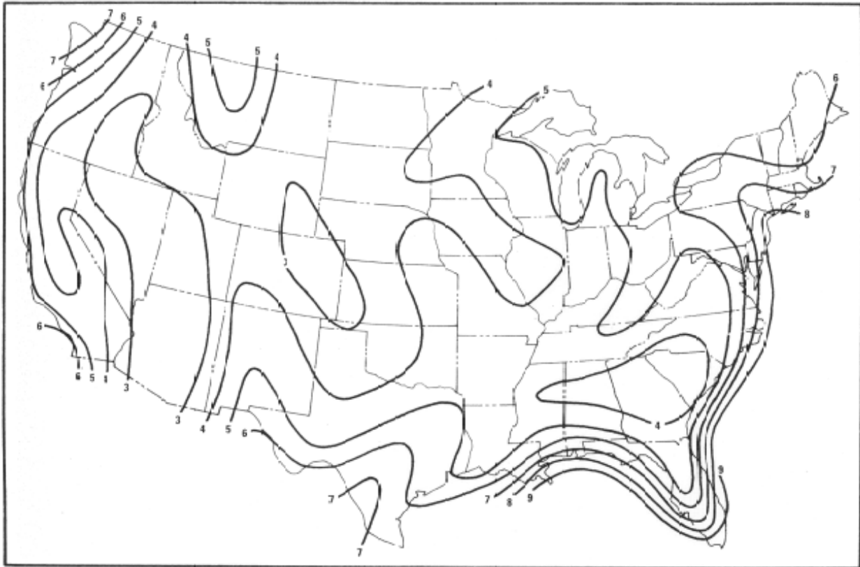
Figure 3.6-22. Mean annual morning mixing heights for the continental United States ( m \times 10^2 ).
