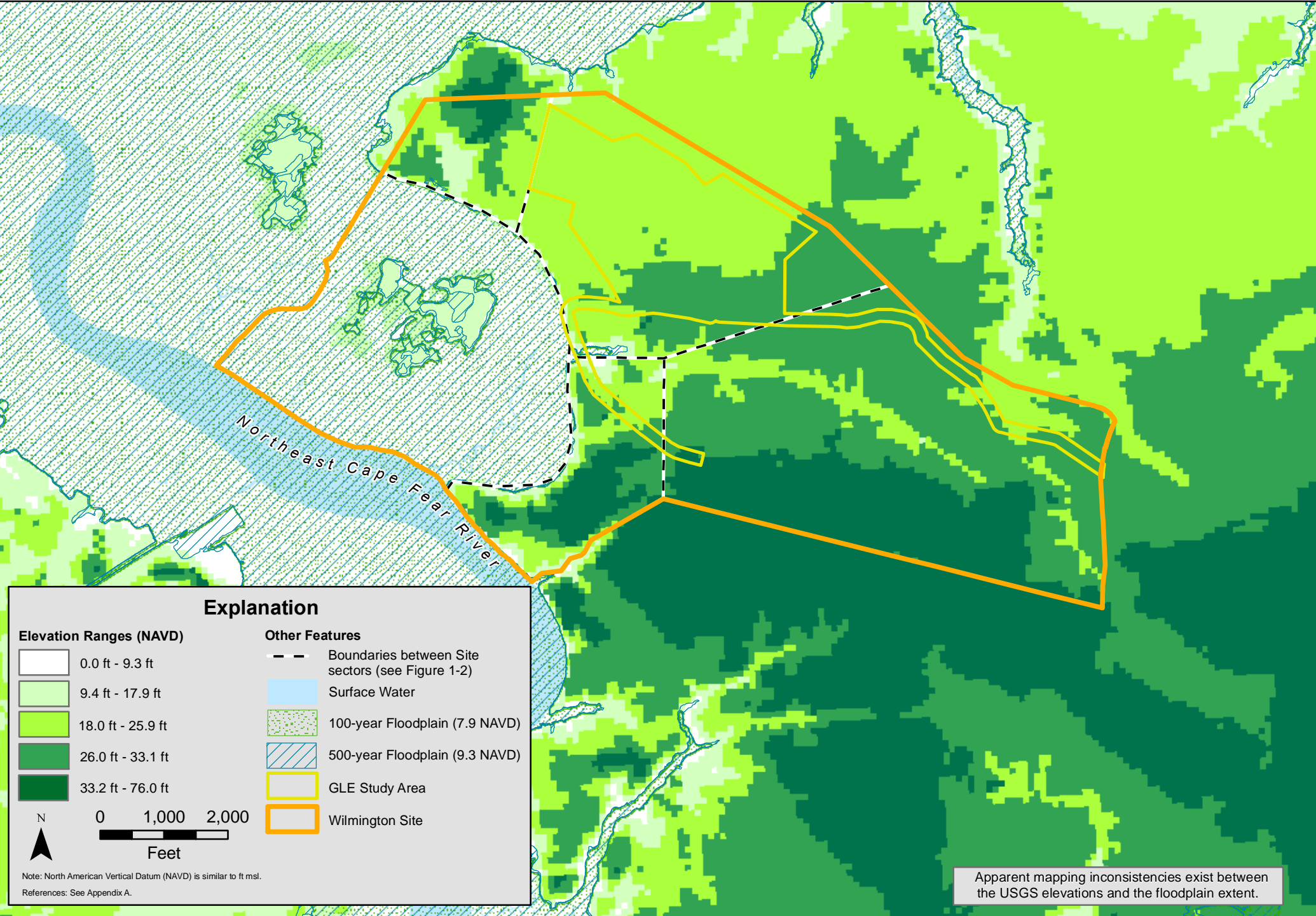
Figure 3.4-25. Floodplain and elevation distribution in the area of the Proposed GLE Facility.
