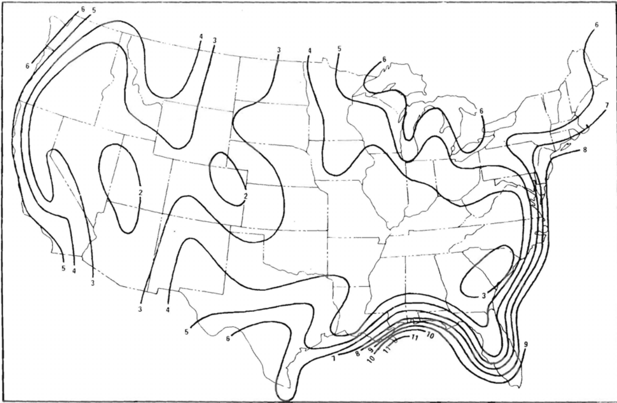
Figure 3.6-26. Mean morning mixing heights in autumn for the continental United States ( m \times 10^2 ).
