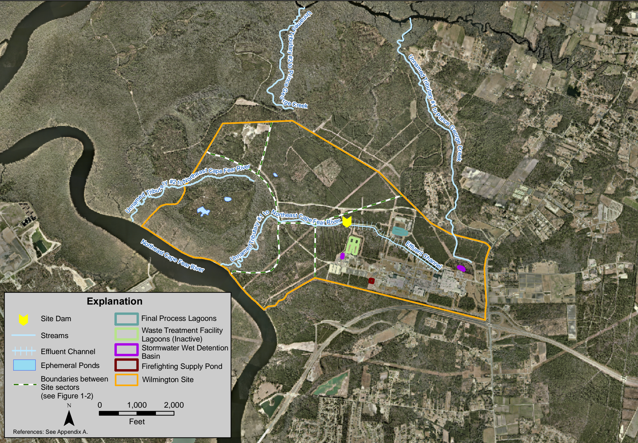
Figure 3.4-19. Wilmington Site surface waters.
