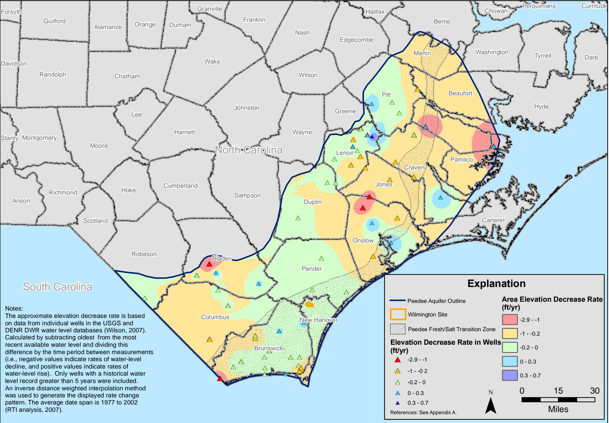
Figure 3.4-29. Approximate rate of groundwater elevation decrease in the Peedee Aquifer.
