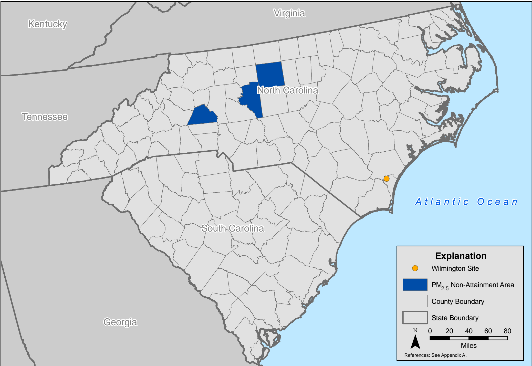
Figure 3.6-38. Wilmington Site location relative to PM 2.5 non-attainment areas.
