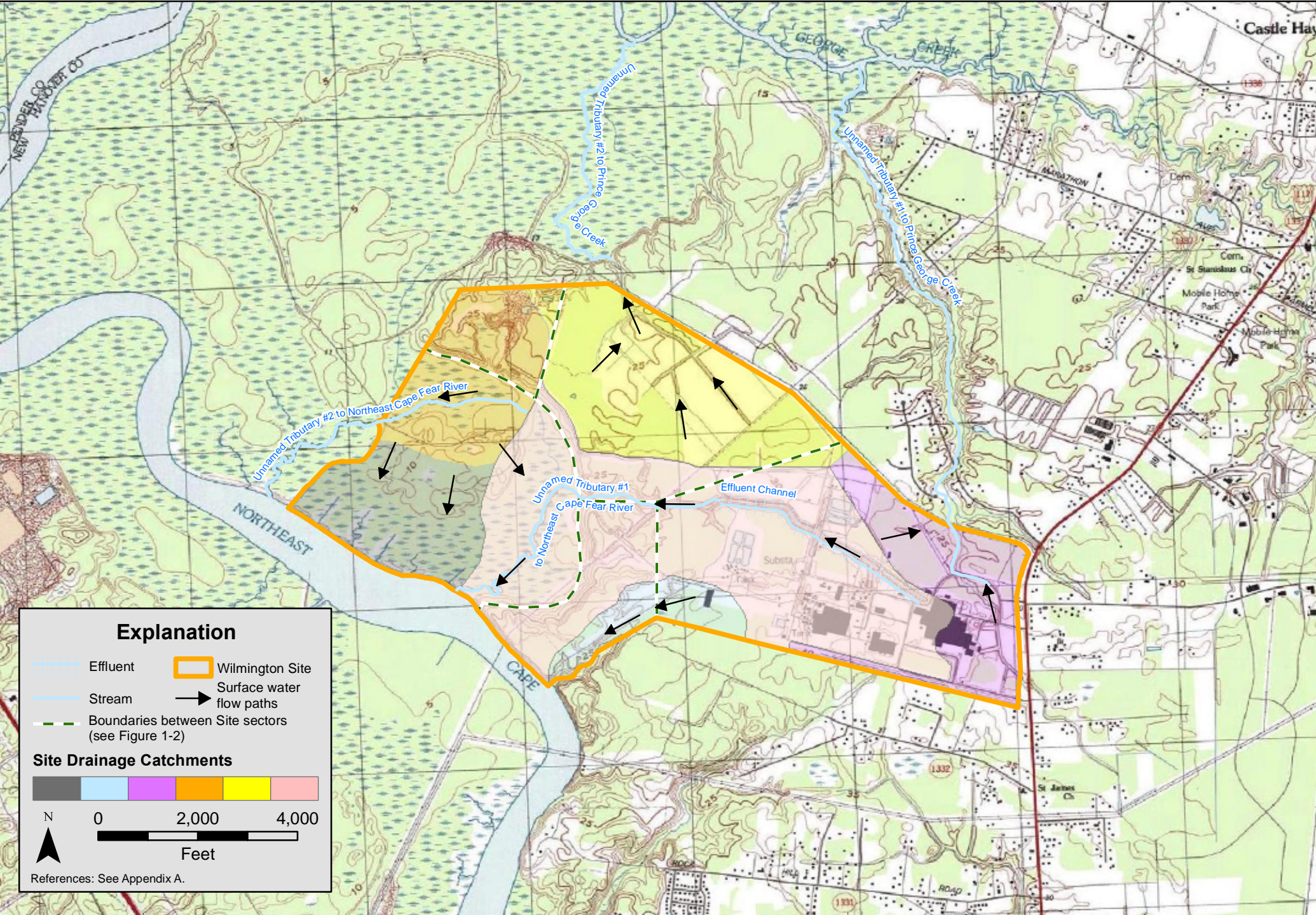
Figure 3.4-23. Current Wilmington Site drainage.
