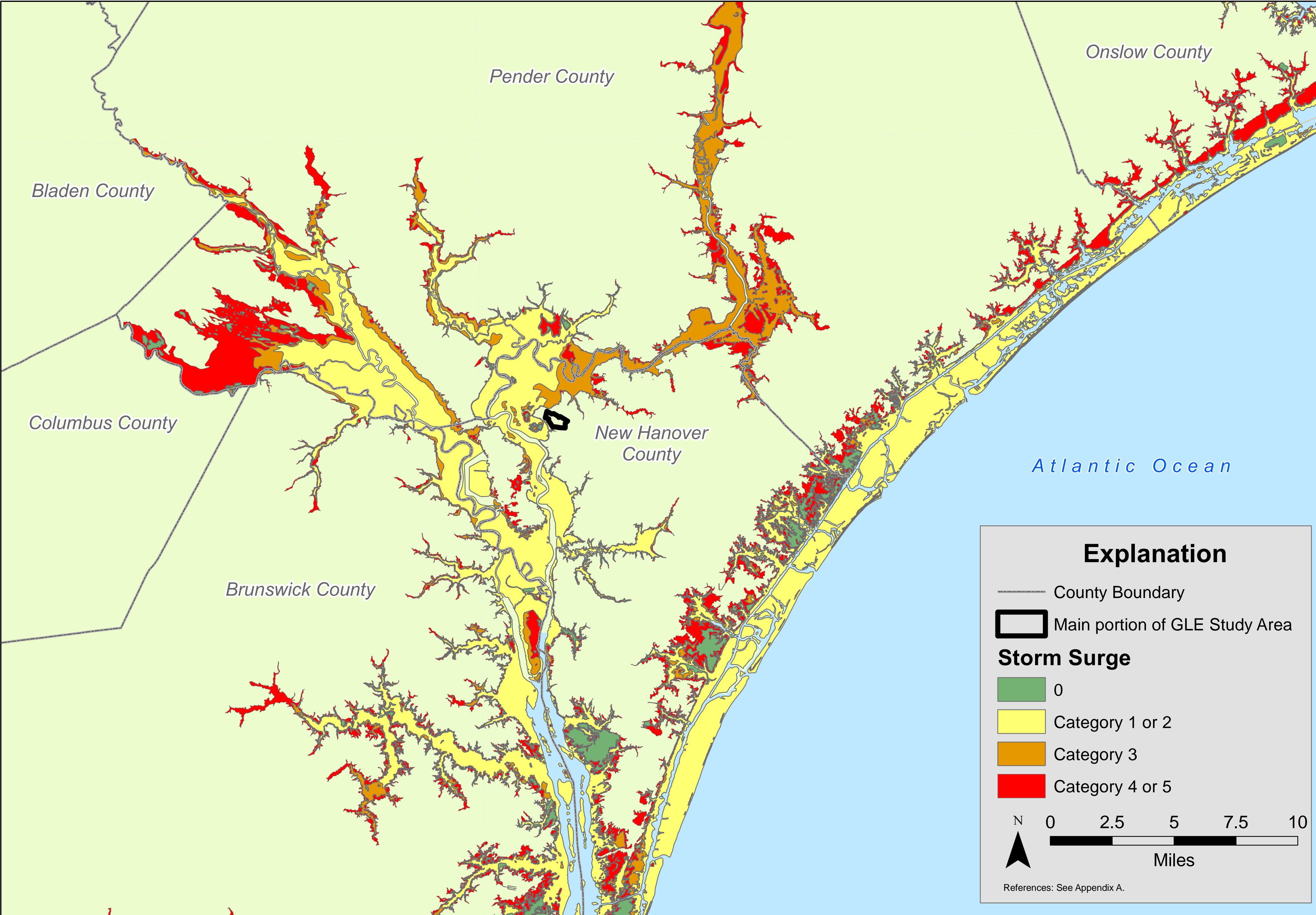
Figure 3.6-35. Hurricane storm surge areas.
