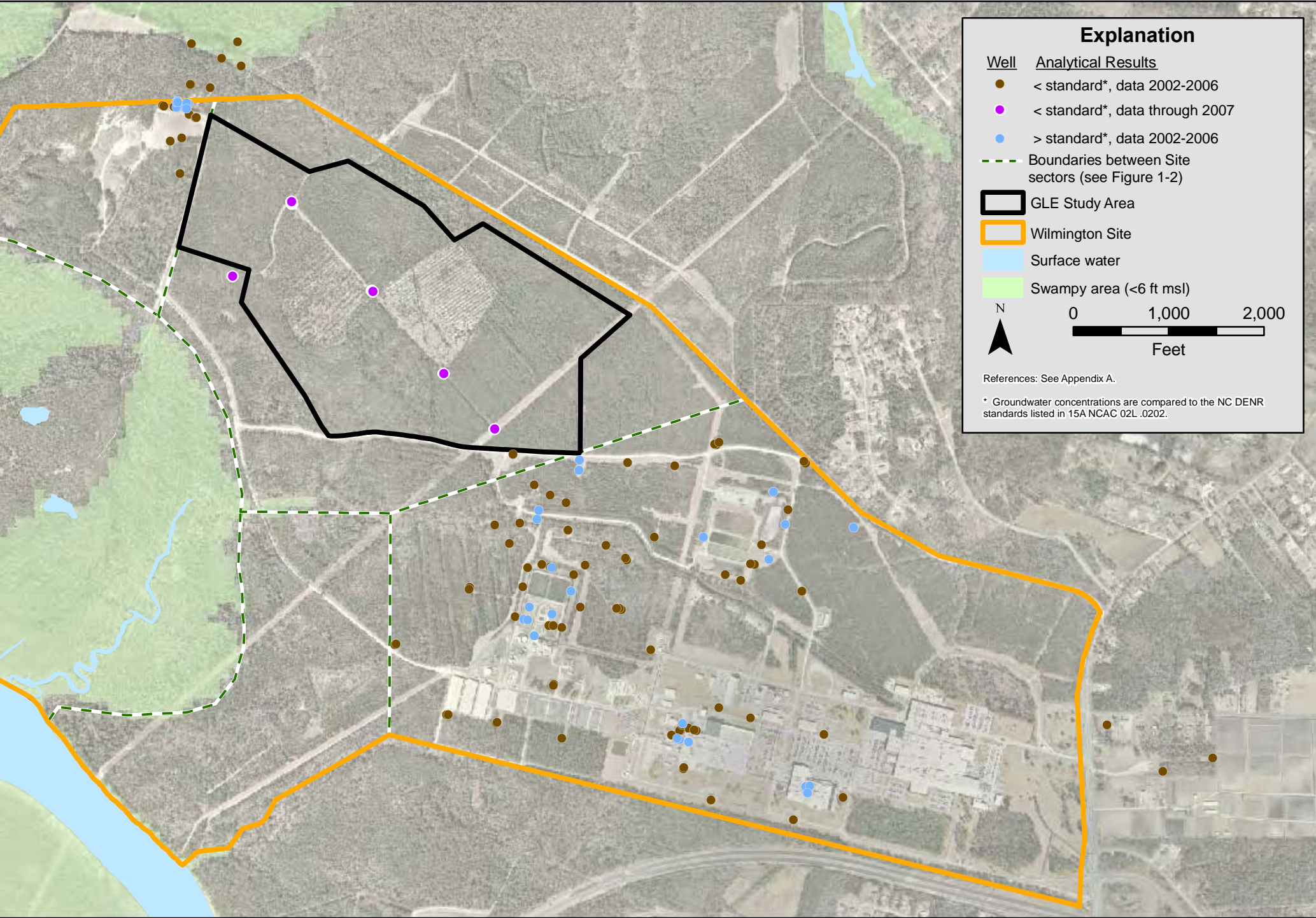
Figure 3.4-16. Summary of groundwater quality data - inorganic and physical constituents.
