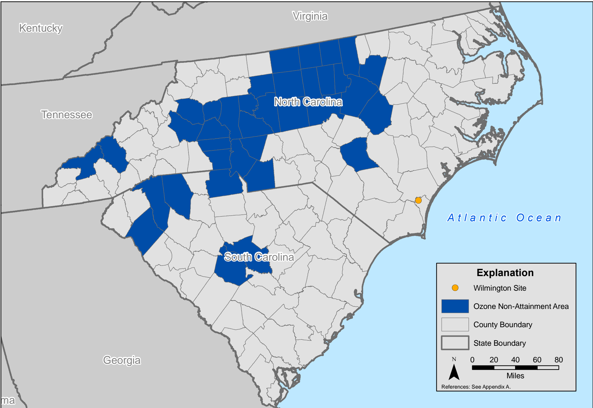
Figure 3.6-37. Wilmington Site location relative to ozone non-attainment areas.
