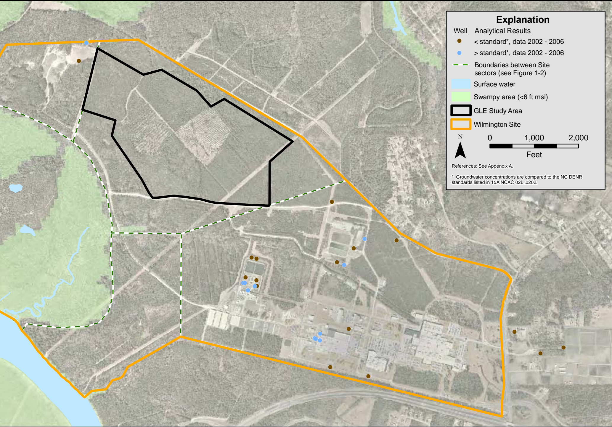
Figure 3.4-17. Summary of groundwater quality data - gross alpha activity.
