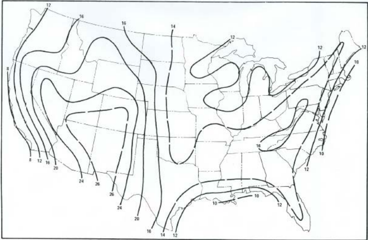
Figure 3.6-27. Mean annual afternoon mixing heights for the continental United States ( m \times 10^2 ).
