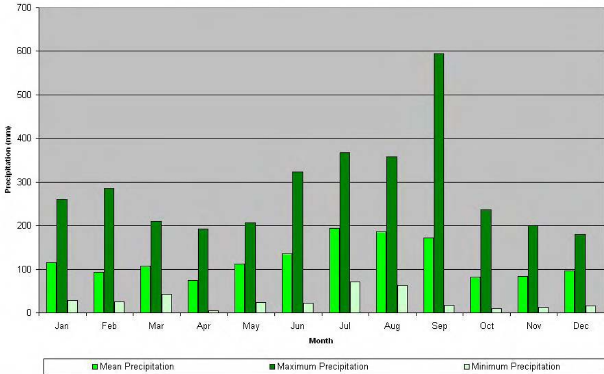
Monthly Precipitation Amount at ILM Airport
