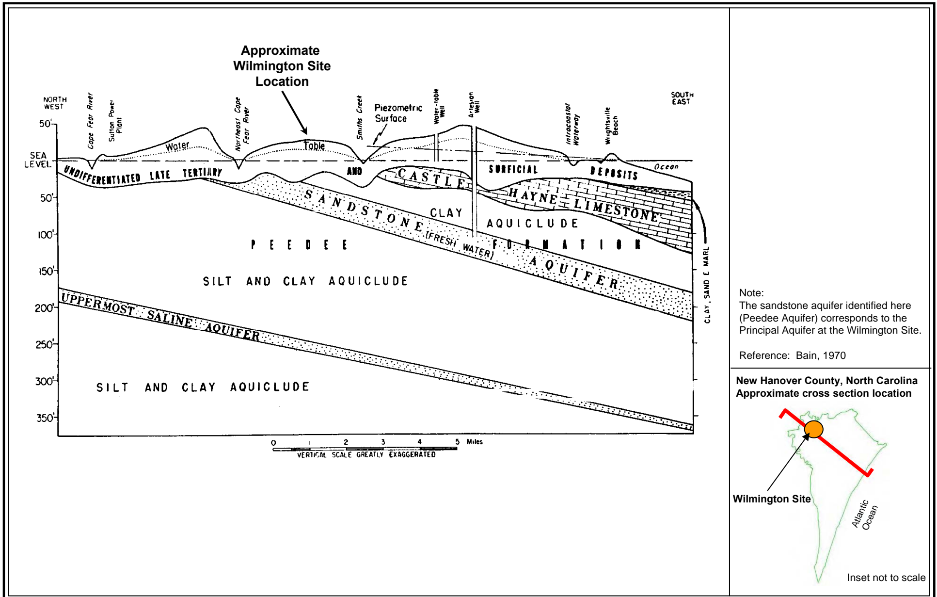
Figure 3.4-9. Hydrogeologic cross section through New Hanover County, NC.
