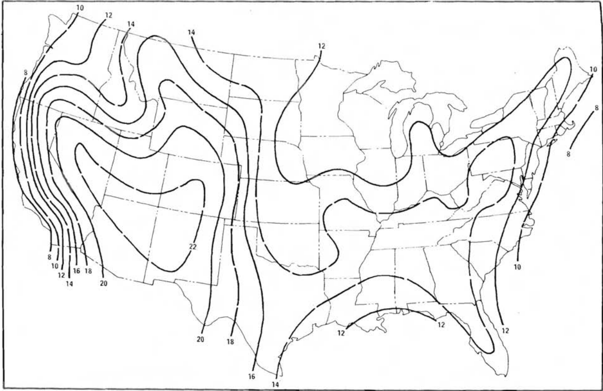
Figure 3.6-31. Mean afternoon mixing heights in autumn for the continental United States ( m \times 10^2 ).
