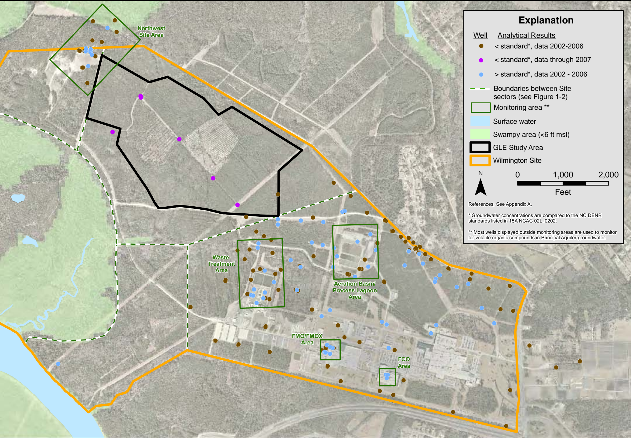
Figure 3.4-14. Summary of groundwater quality data – all monitored constituents.
