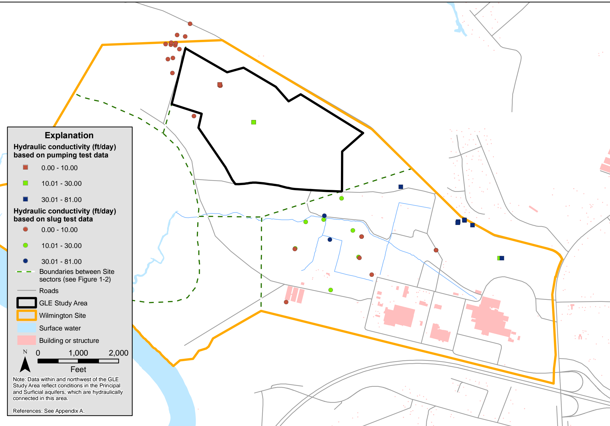
Figure 3.4-12. Measured Principal Aquifer hydraulic conductivity (ft/day).
