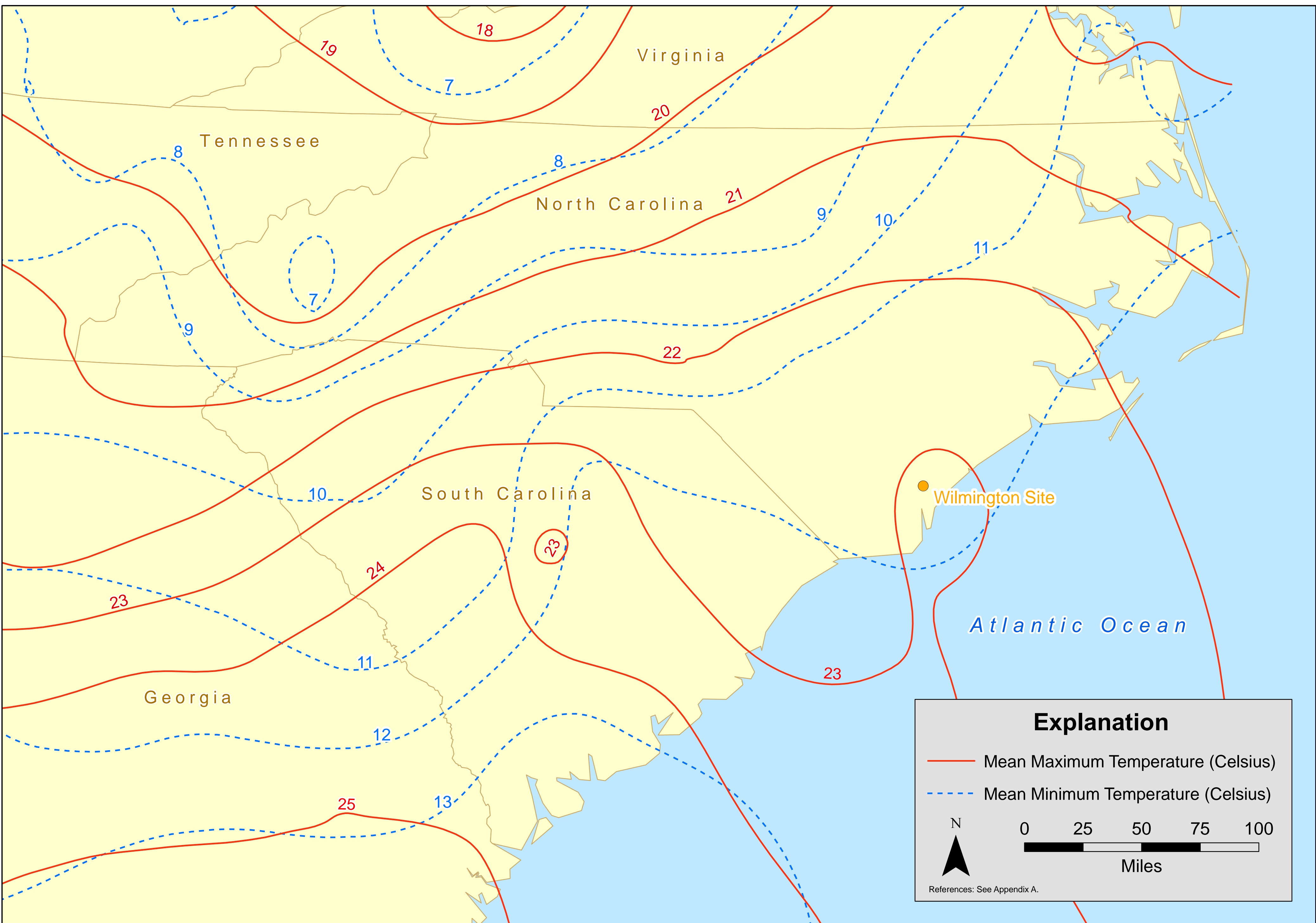
Figure 3.6-2. Mean annual maximum and minimum temperatures for North Carolina.
