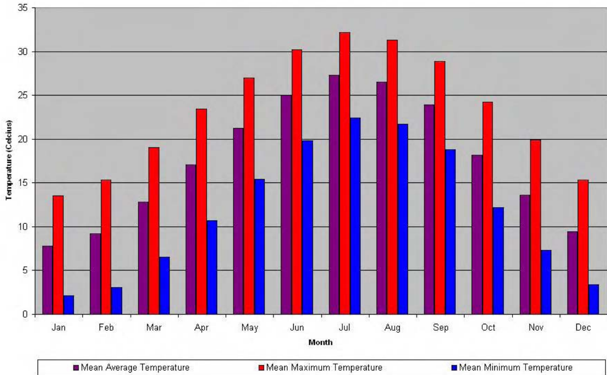
Mean Temperatures at ILM Airport
