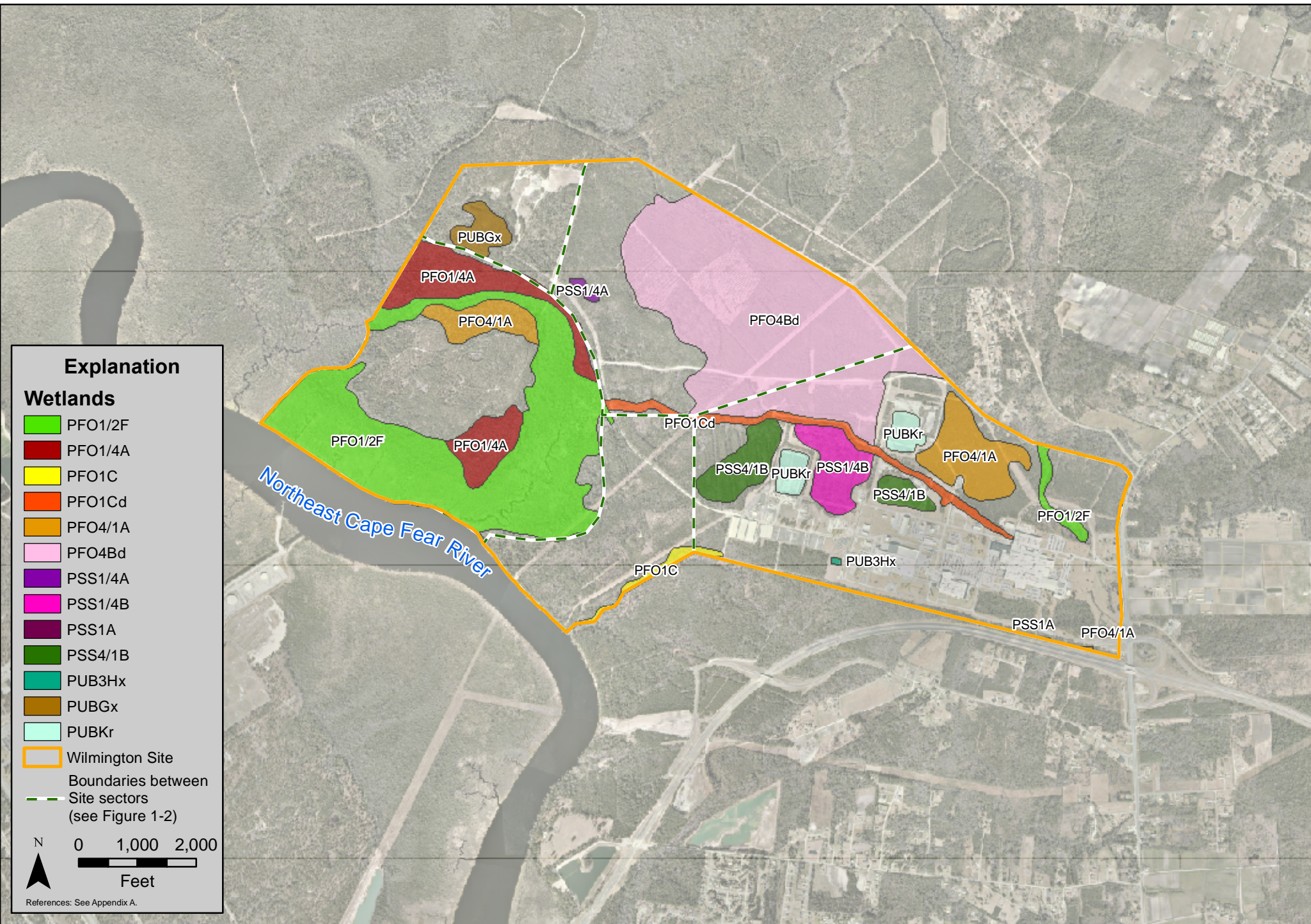
Figure 3.4-26. Wilmington Site wetlands as classified by the National Wetlands Inventory.
