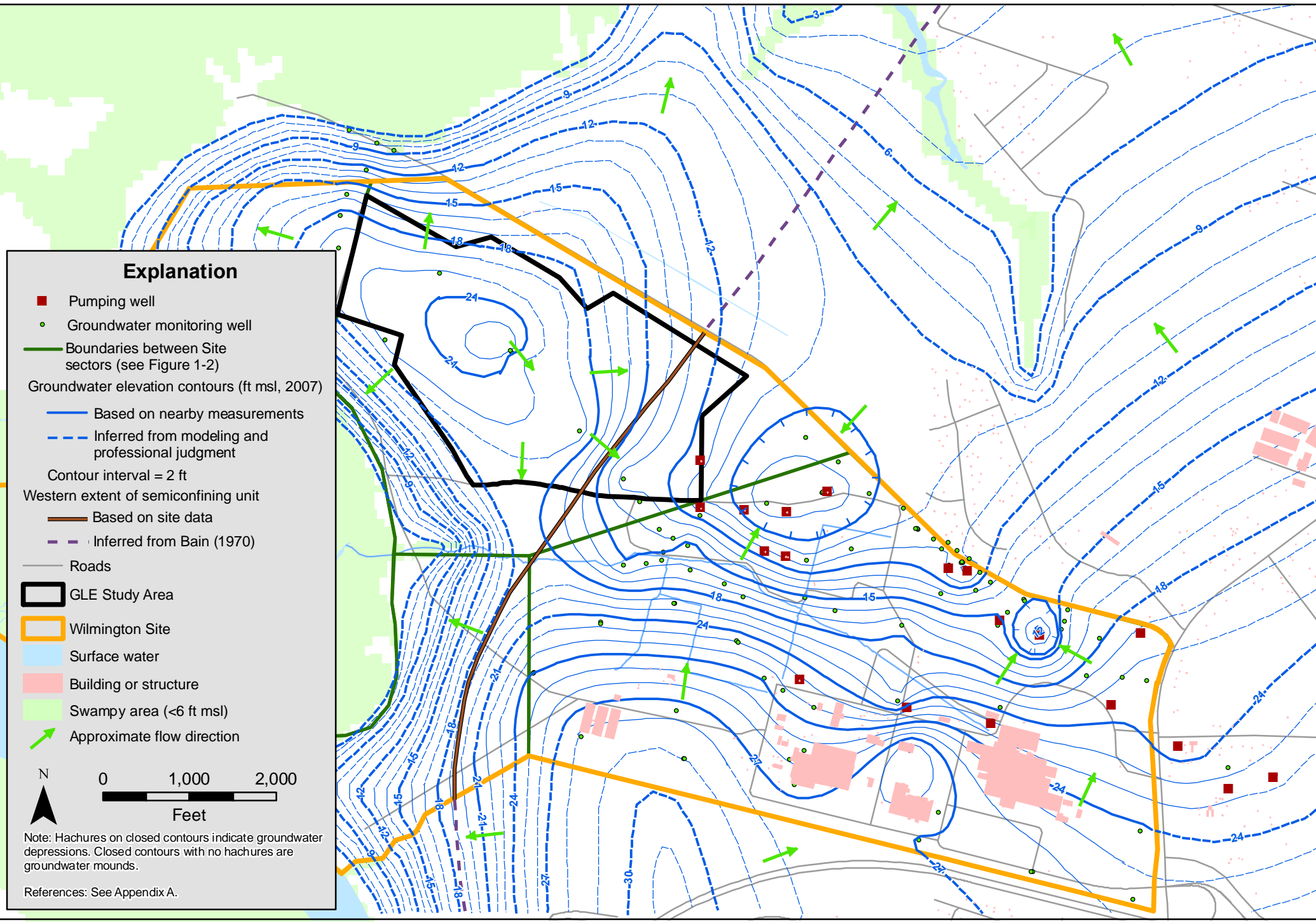
Figure 3.4-10. Principal Aquifer groundwater elevation contours (2007).
