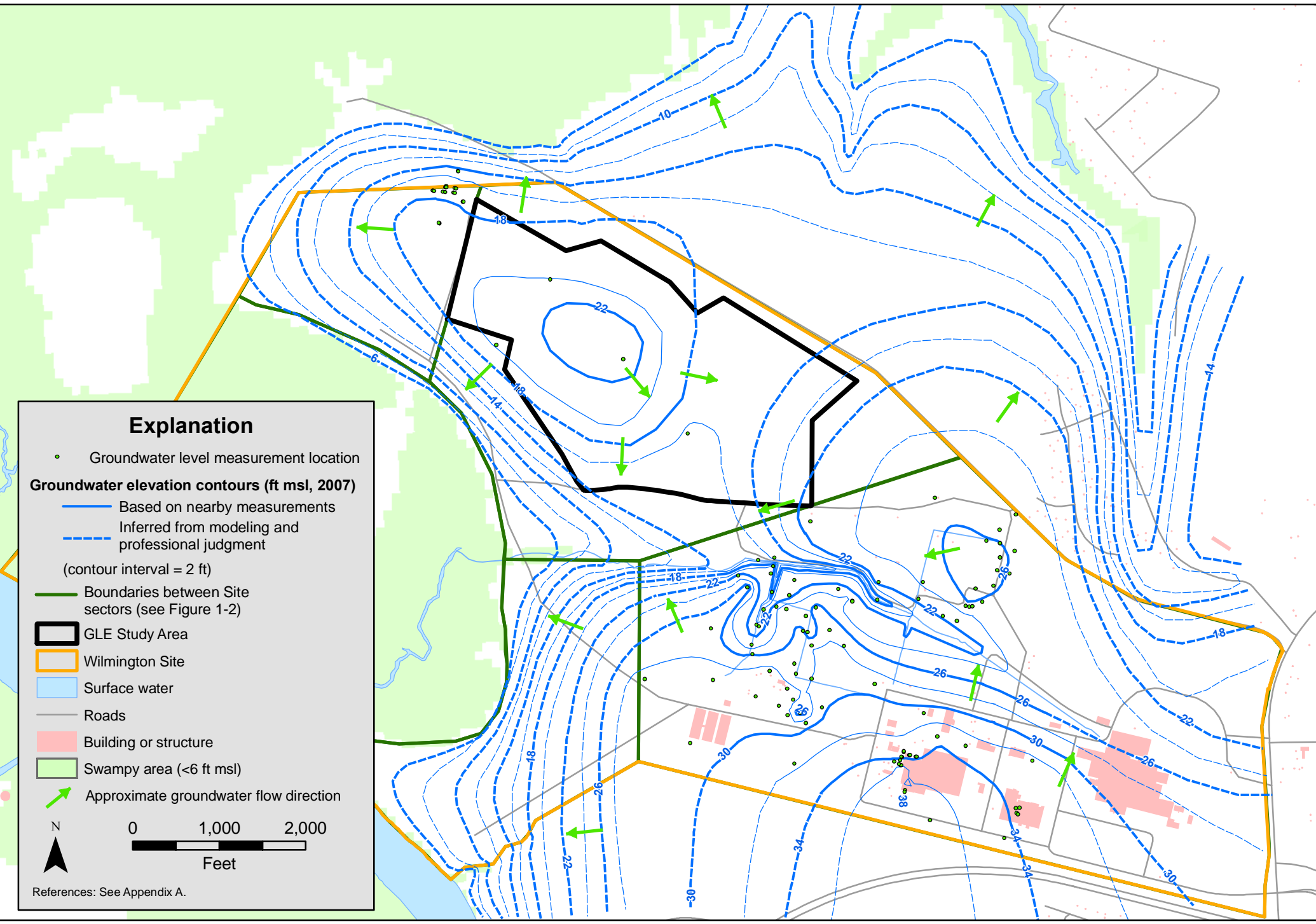
Figure 3.4-7. Surficial Aquifer groundwater elevation contours (2007).
