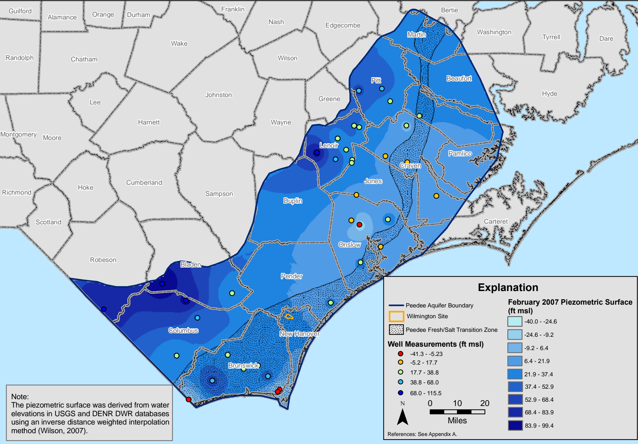
Figure 3.4-28. Peedee Aquifer groundwater elevations, 2007.
