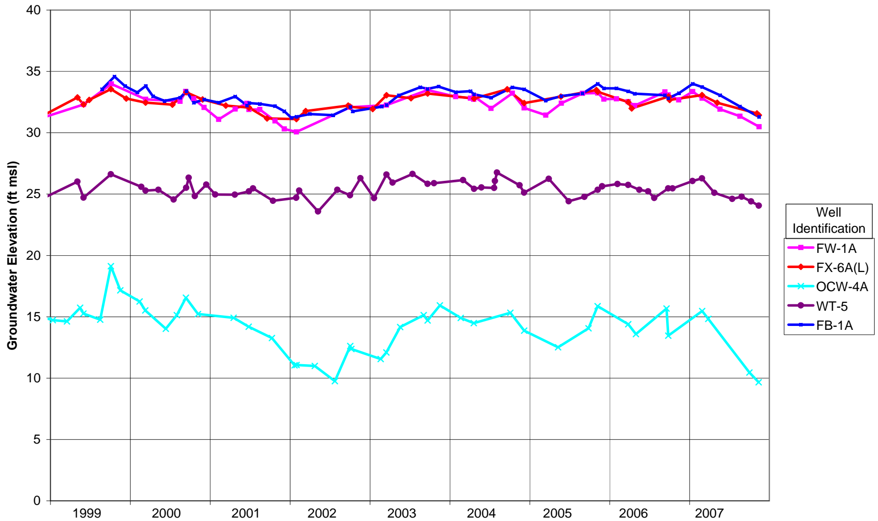
Figure 3.4-8. Example Surficial Aquifer hydrographs.
