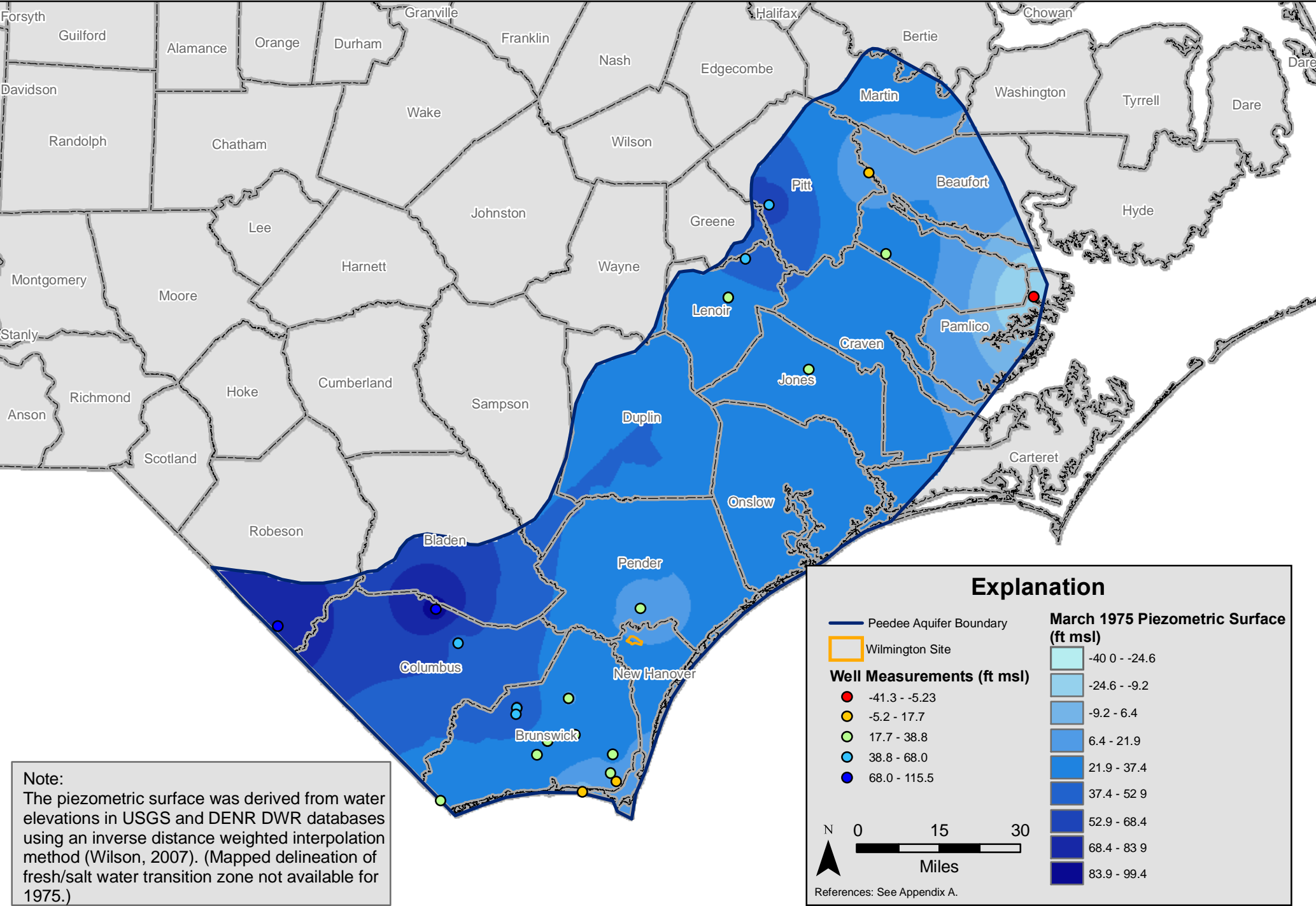
Figure 3.4-27. Peedee Aquifer groundwater elevations, 1975.
