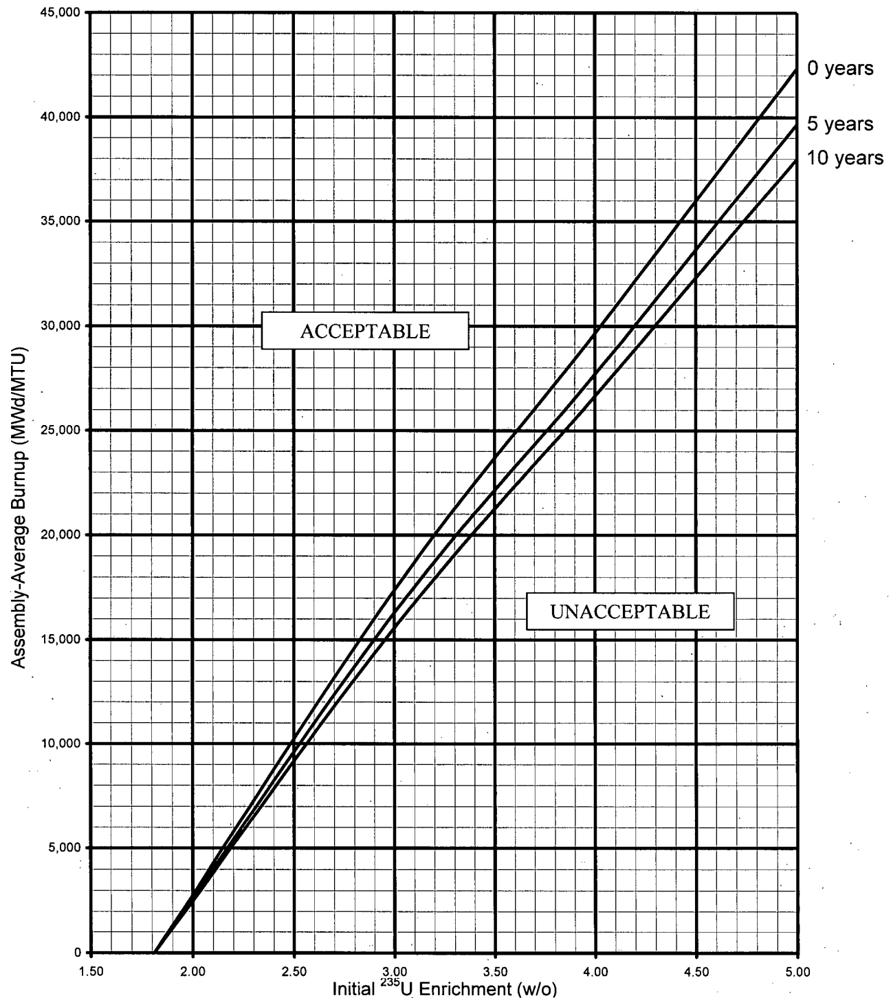
Figure 1: Minimum Fuel Assembly Burnup and Decay Time Versus Nominal Initial Enrichment for Region 2 Storage Configuration
