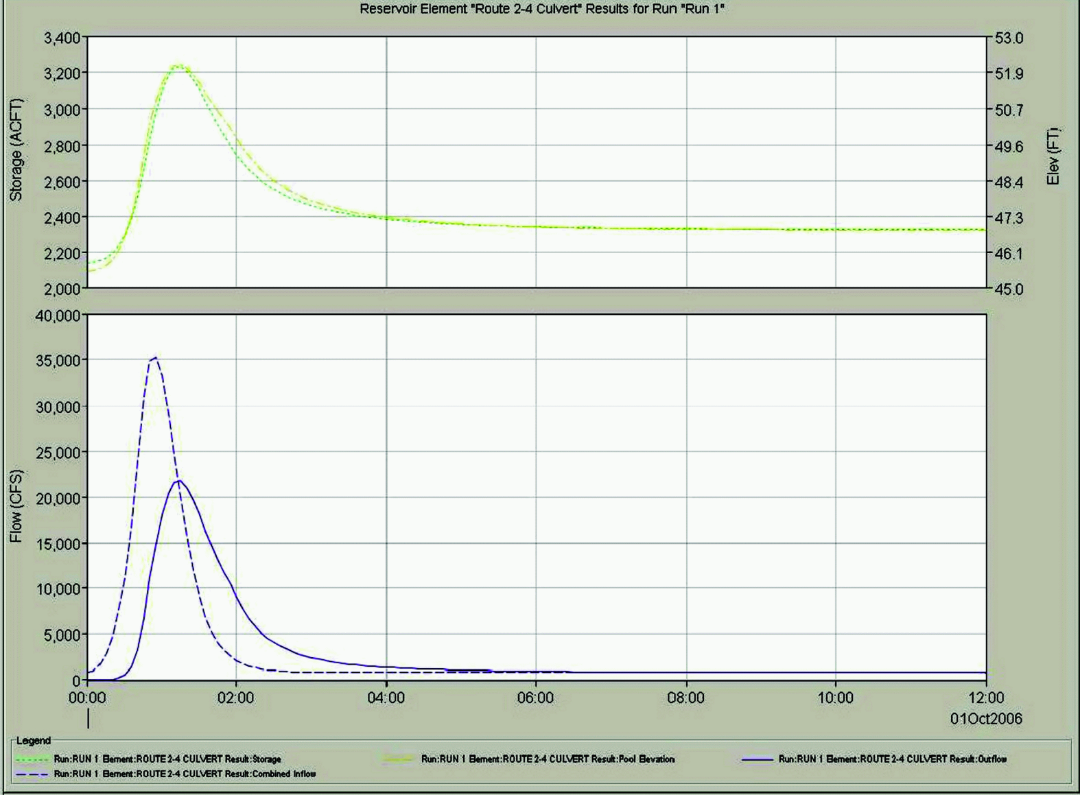
Figure 2.4-13—{Storage And Inflow & Outflow Hydrographs at Maryland Route 2-4 Culvert}
