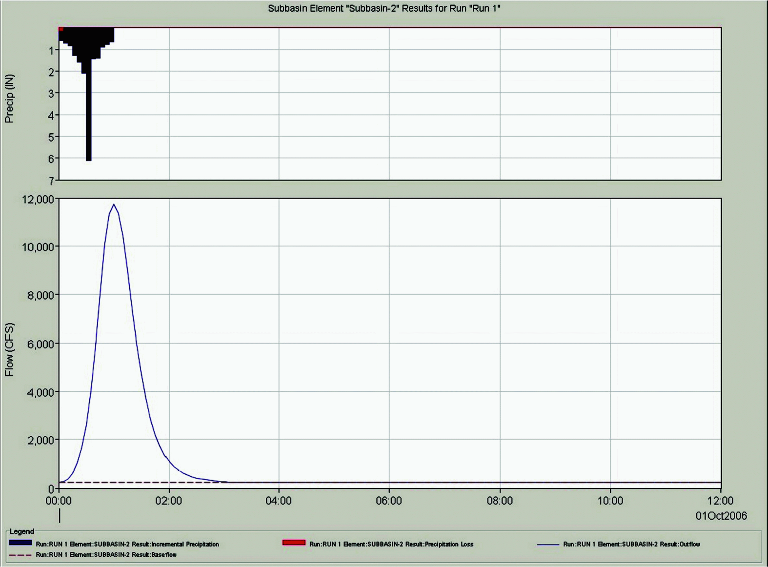
Figure 2.4-15—{Sub-Basin 2 Hydrograph}
