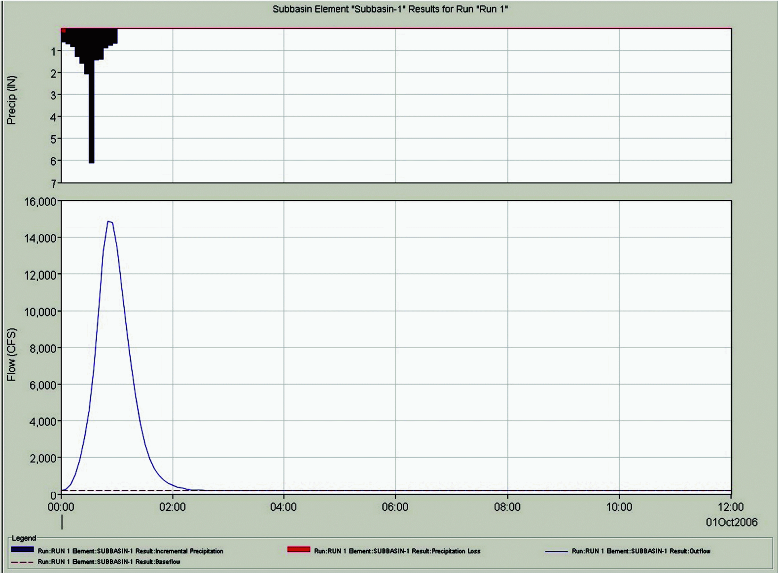
Figure 2.4-14—{Sub-Basin 1 Hydrograph}
