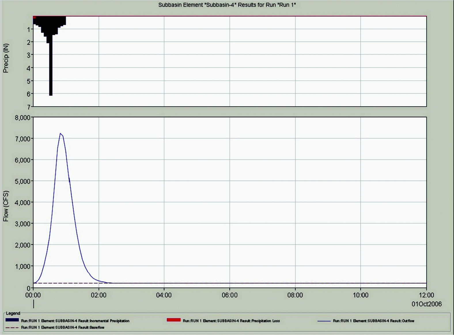
Figure 2.4-17—{Sub-Basin 4 Hydrograph}
