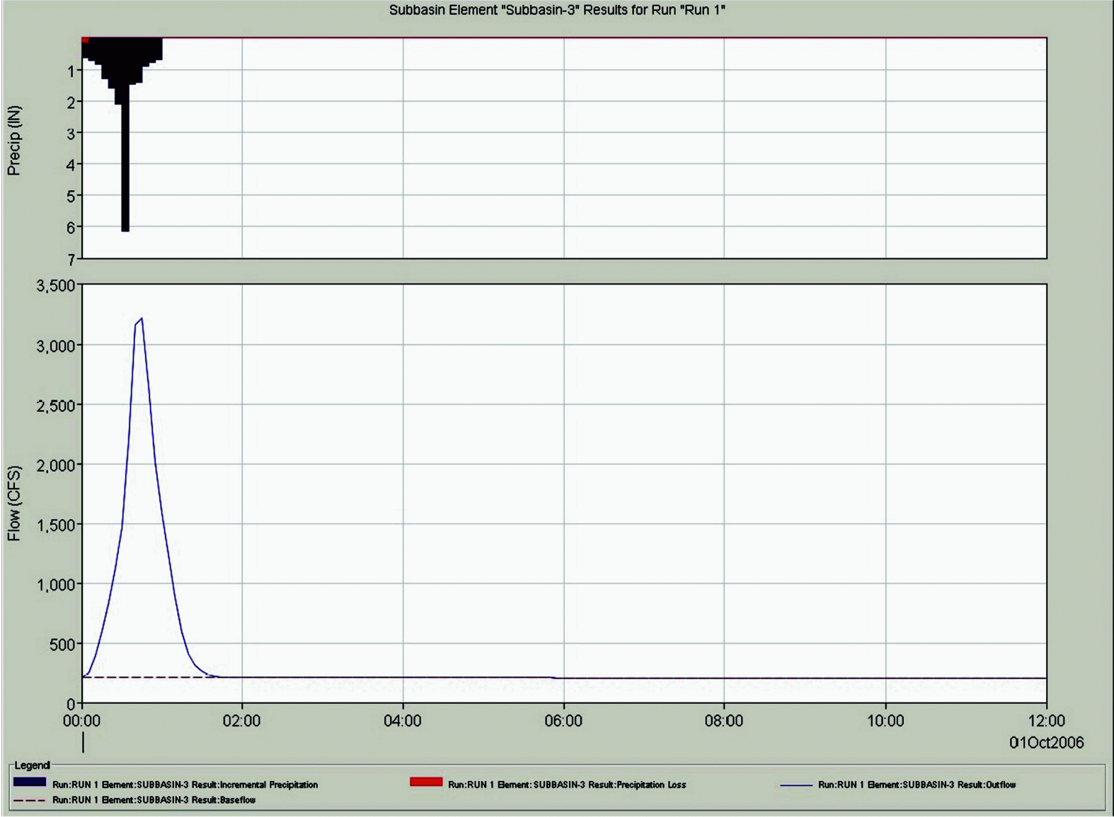
Figure 2.4-16—{Sub-Basin 3 Hydrograph}
