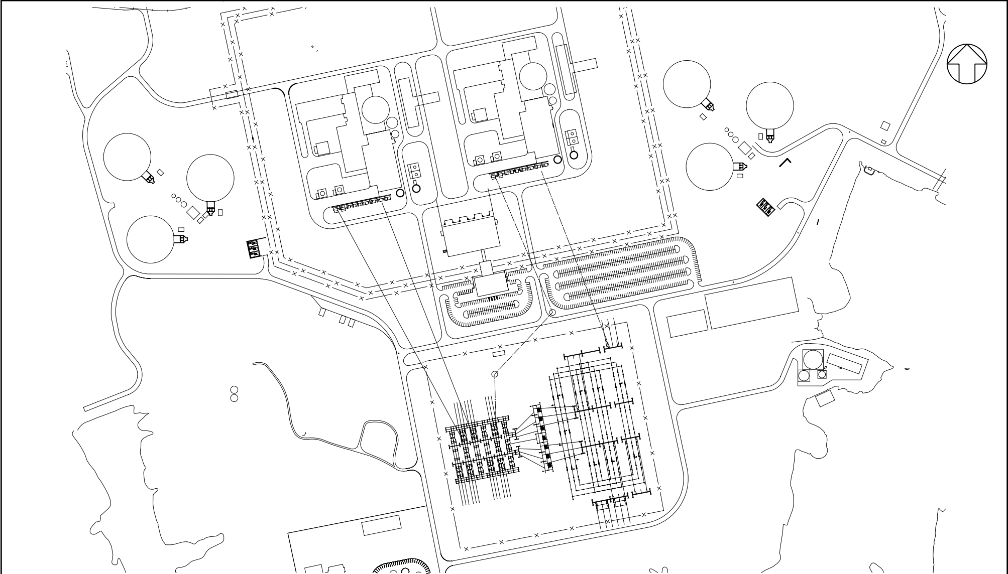
WILLIAM STATES LEE III NUCLEAR STATION UNITS 1 & 2 Switchyard General Arrangement
