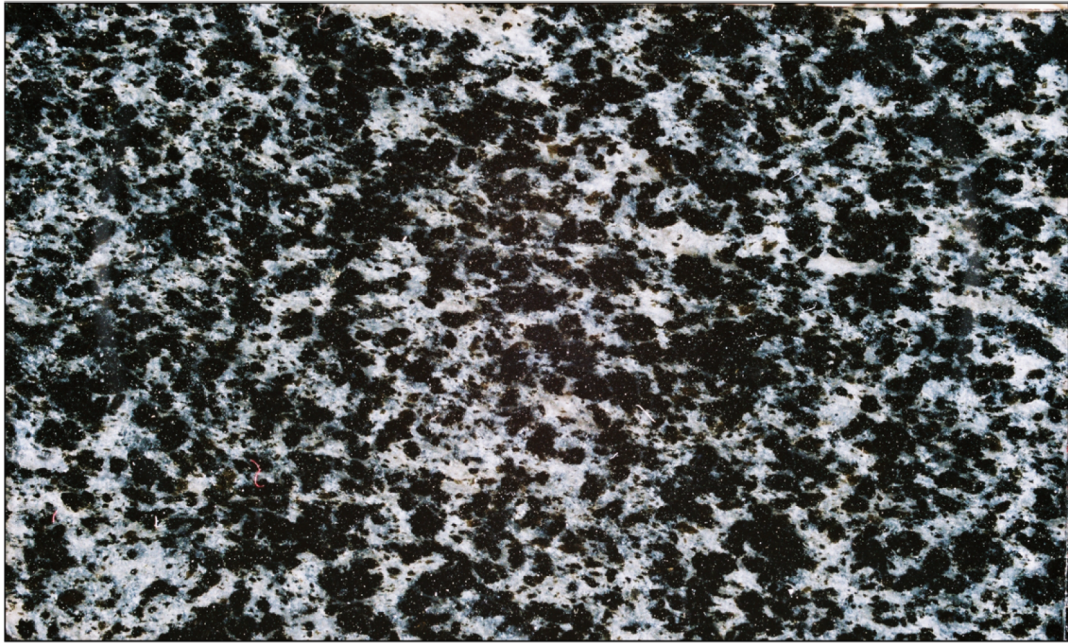
Mica-schist showing typical appearance of hand specimen with abundant biotite porphyroblasts
