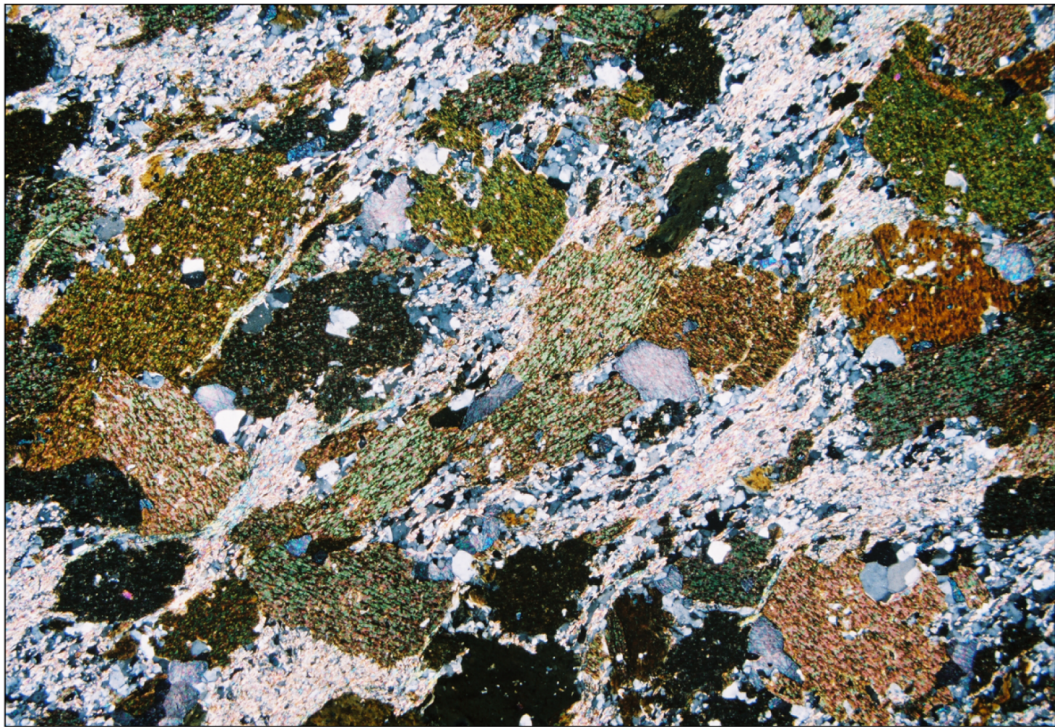
Mica-schist showing typical appearance of biotite porphyroblasts
