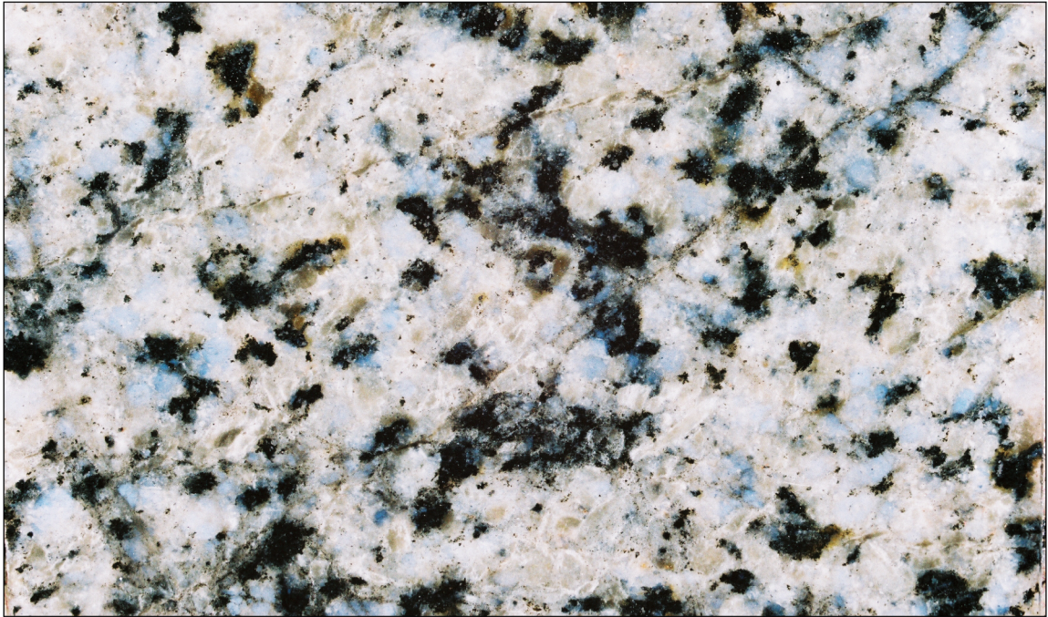
Meta-quartz Diorite showing typical appearance of hand specimen
