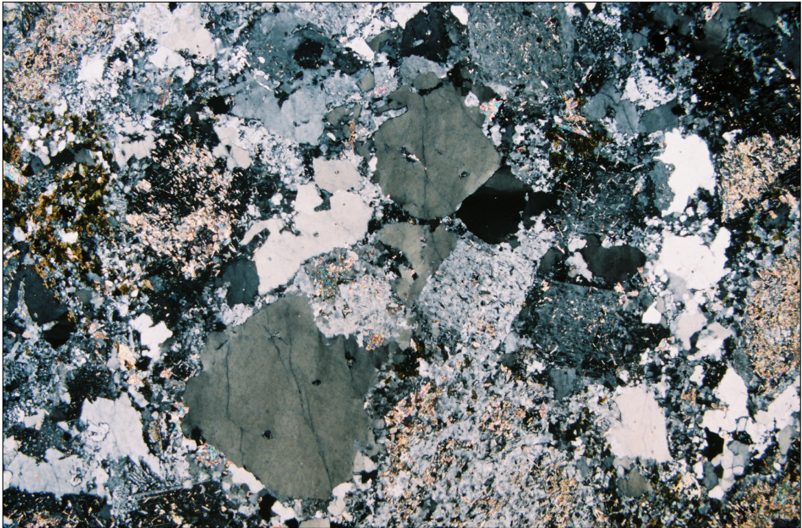
Meta-quartz Diorite showing typical appearance of relict hypidiomorphic texture in thin section
