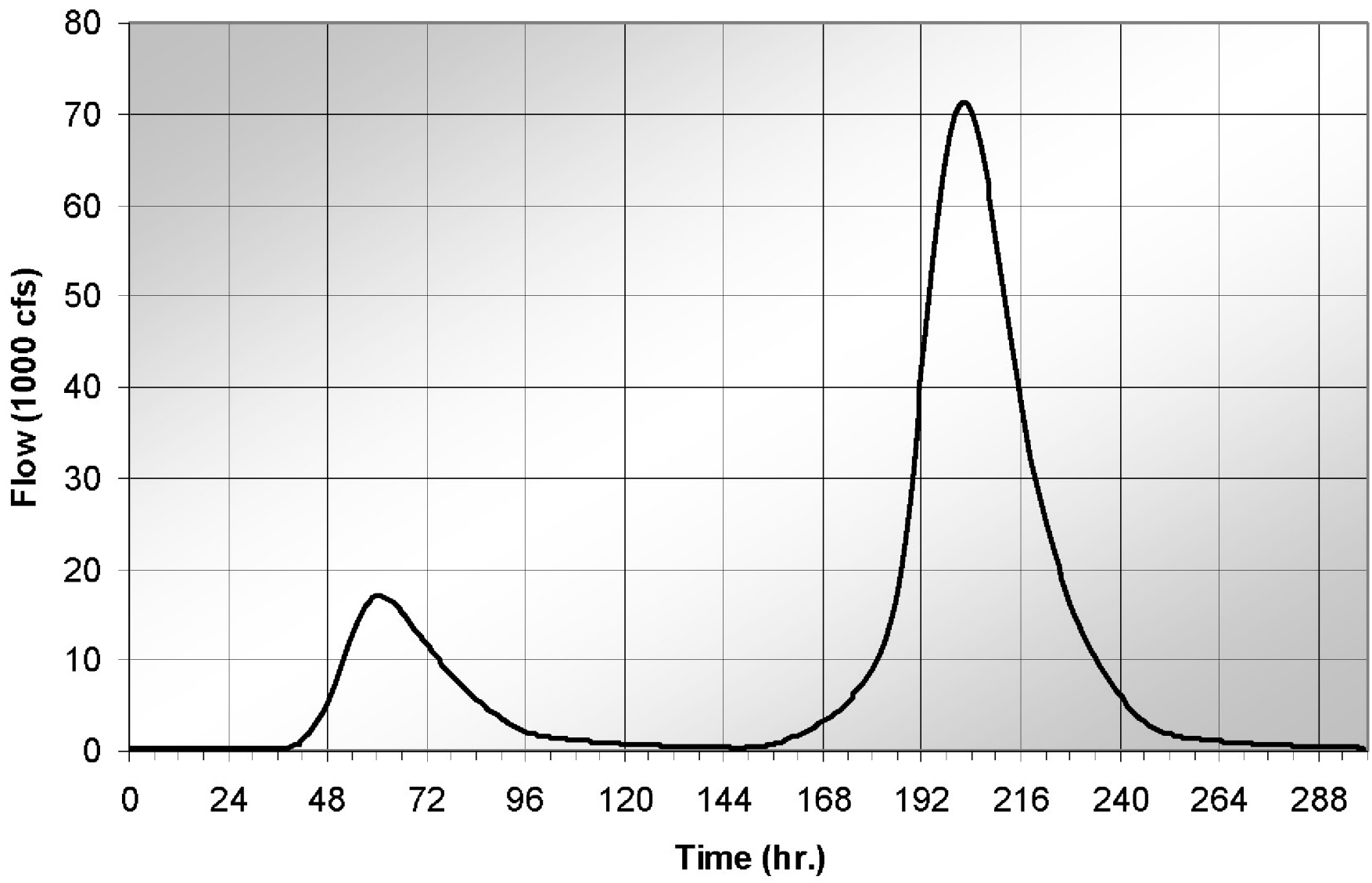
WILLIAM STATES LEE III NUCLEAR STATION UNITS 1 & 2 Subbasin BC-14 and Routed Subbasin KMR-13 PMF Combined Inflow Hydrograph FIGURE 2.4.3-220 Rev 0
