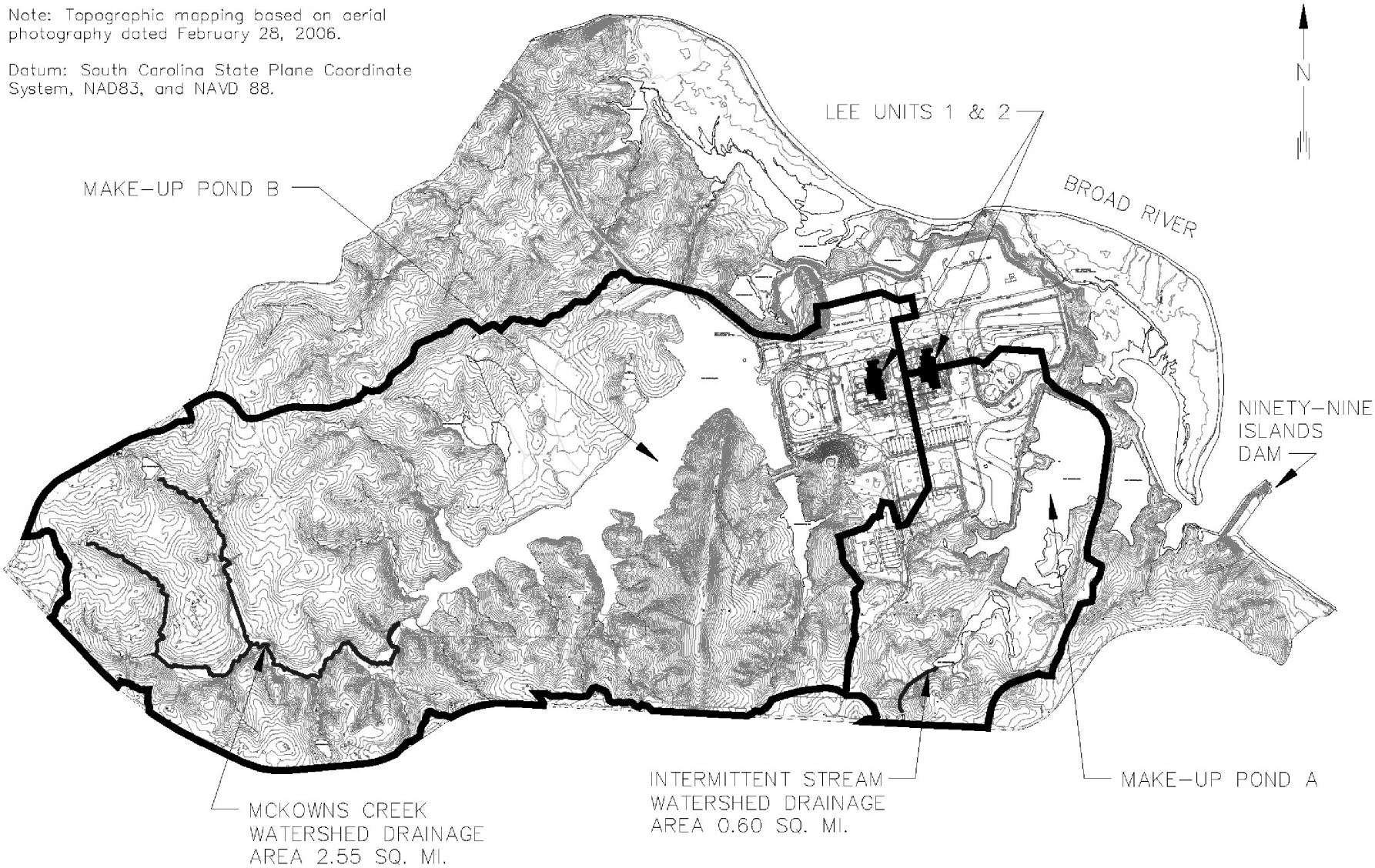
WILLIAM STATES LEE III NUCLEAR STATION UNITS 1 & 2 Make-Up Pond A and Make-Up Pond B Watersheds FIGURE 2.4.3-201 Rev 0
