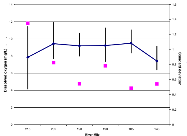
Figure 3. Dissolved oxygen statistics from several river stations within the first 6 months of the study. Vertical bars indicate range of values.
