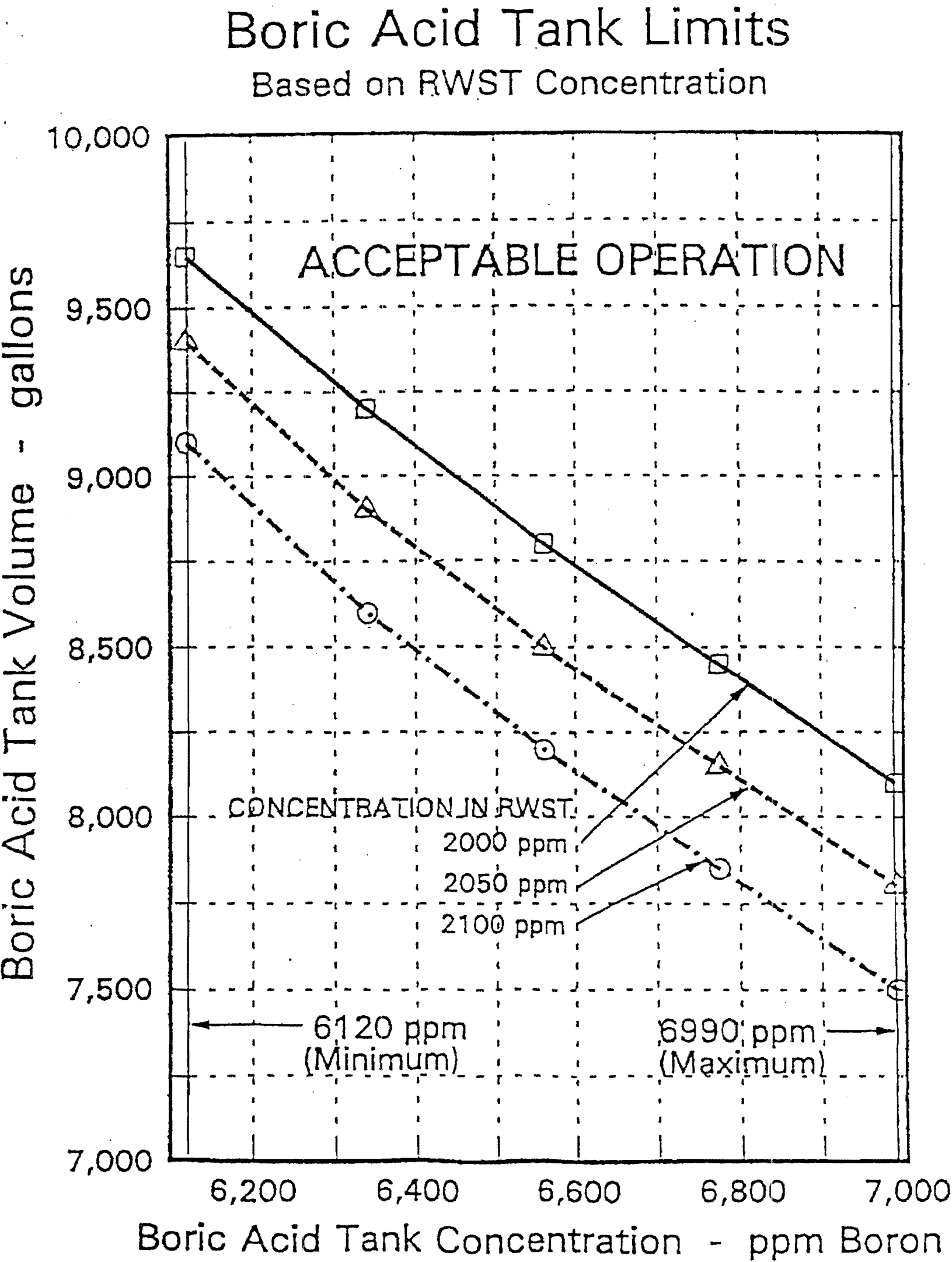
Figure 9.3-21 Watts Bar Nuclear Plant Boric Acid Tank Limits
