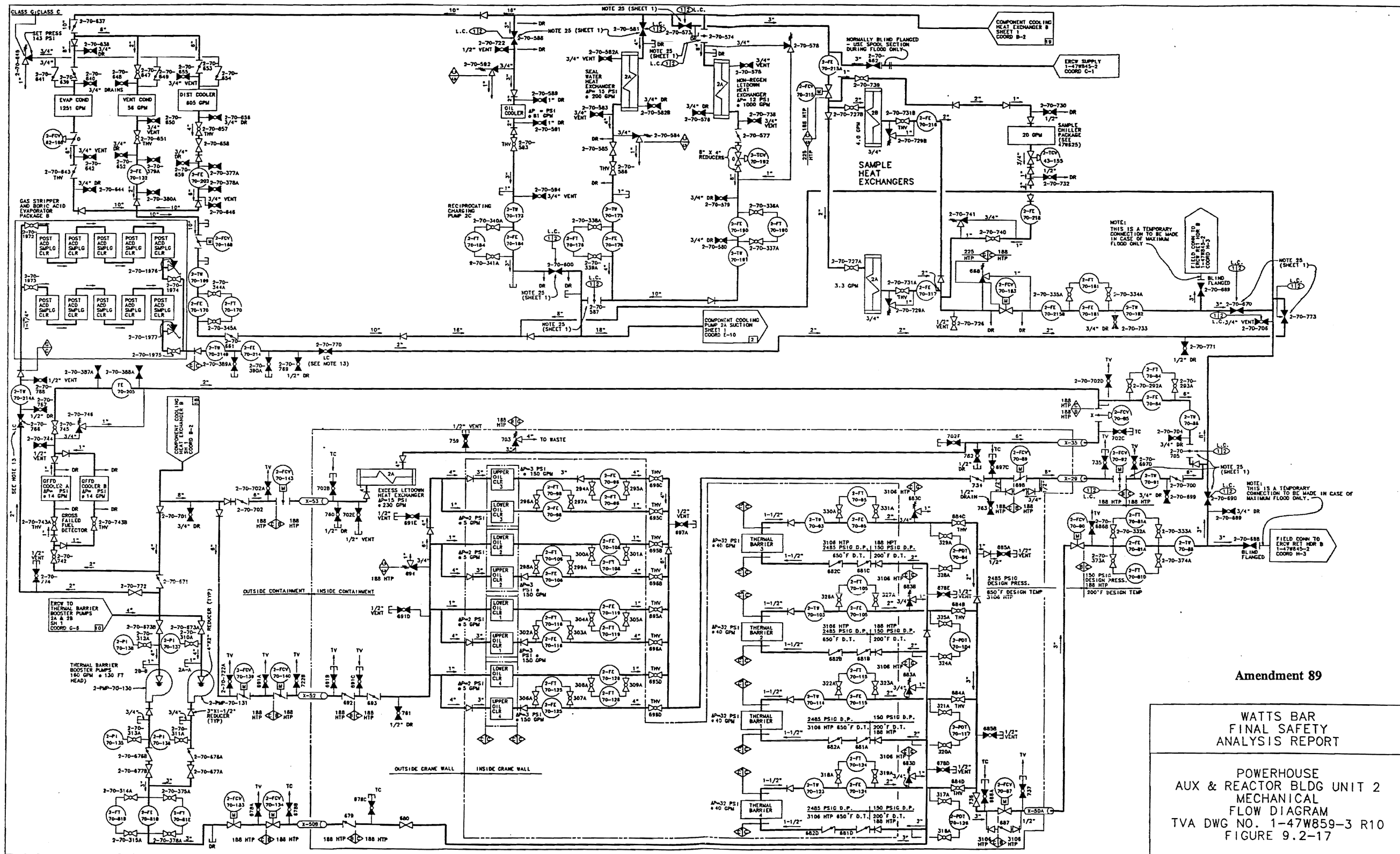
Figure 9.2-17 Powerhouse, Auxiliary and Reactor Building Flow Diagram for Component Cooling System (Unit 2)
