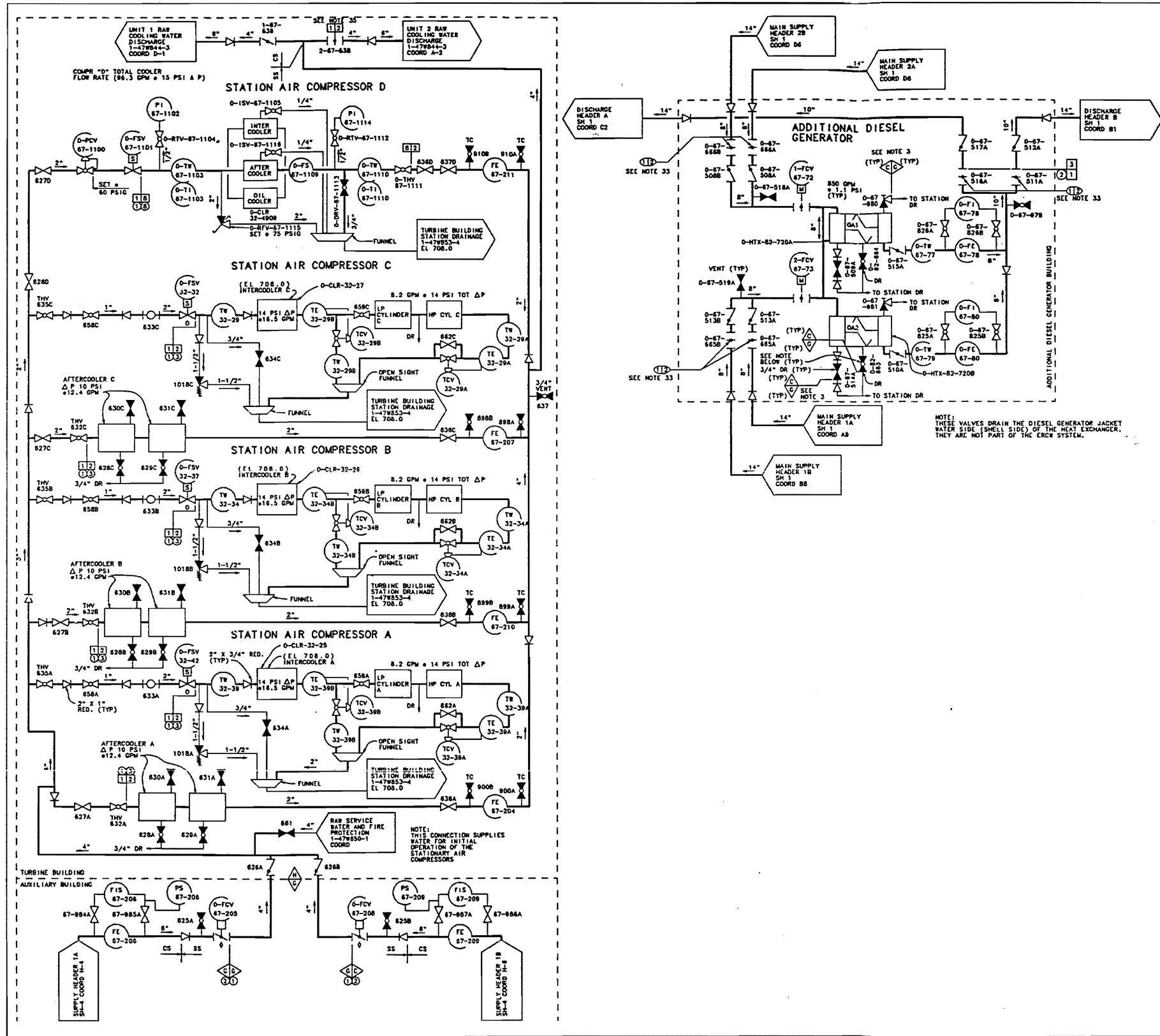
Figure 9.2-4a Powerhouse Turbine Building Units 1 & 2 Flow Diagram for Essential Raw Cooling Water System
