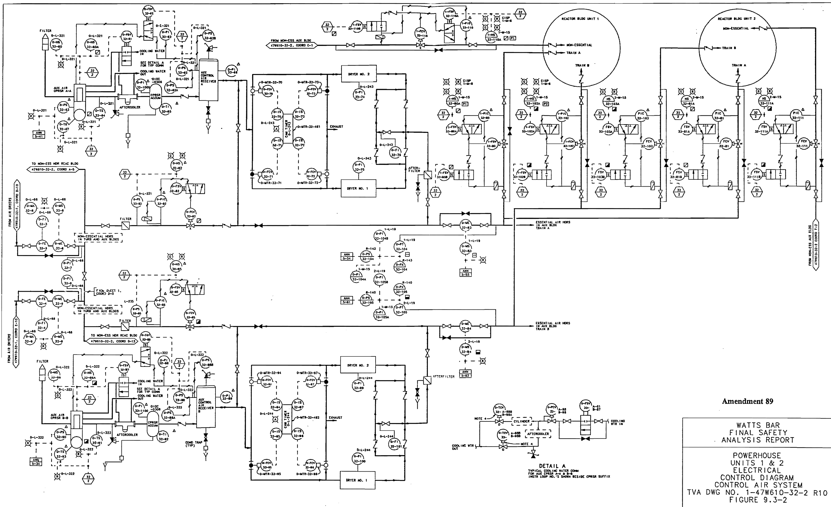
Figure 9.3-2 Electrical Control Diagram for Control Air System
