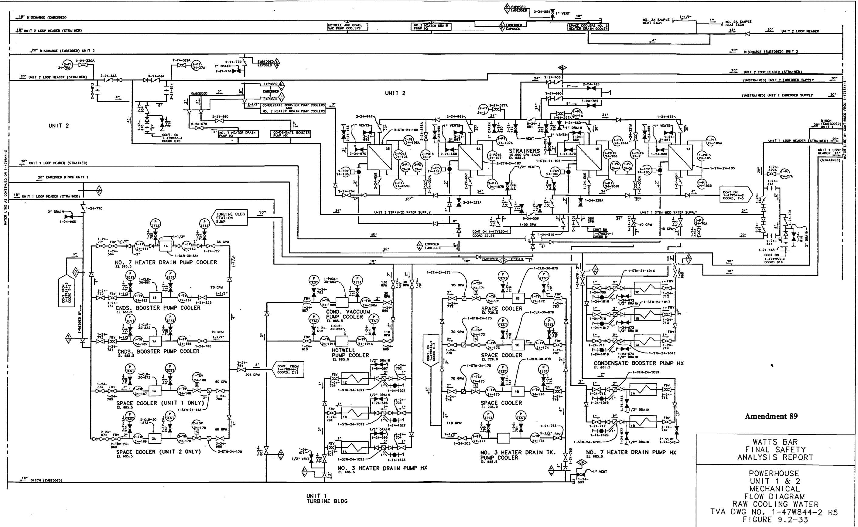
Figure 9.2-33 Powerhouse Flow Diagram for Raw Cooling Water
