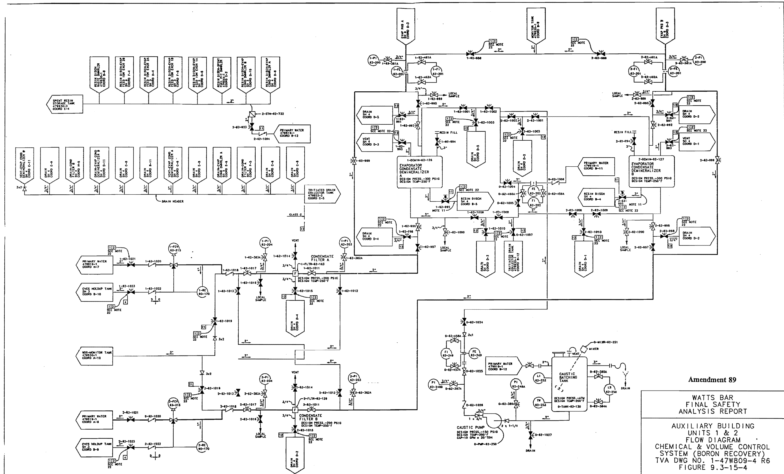
Figure 9.3-15 Auxiliary Building Units 1 &amp; 2 Flow Diagram for Chemical and Volume Control System (Boron Recovery) (Sheet 4)
