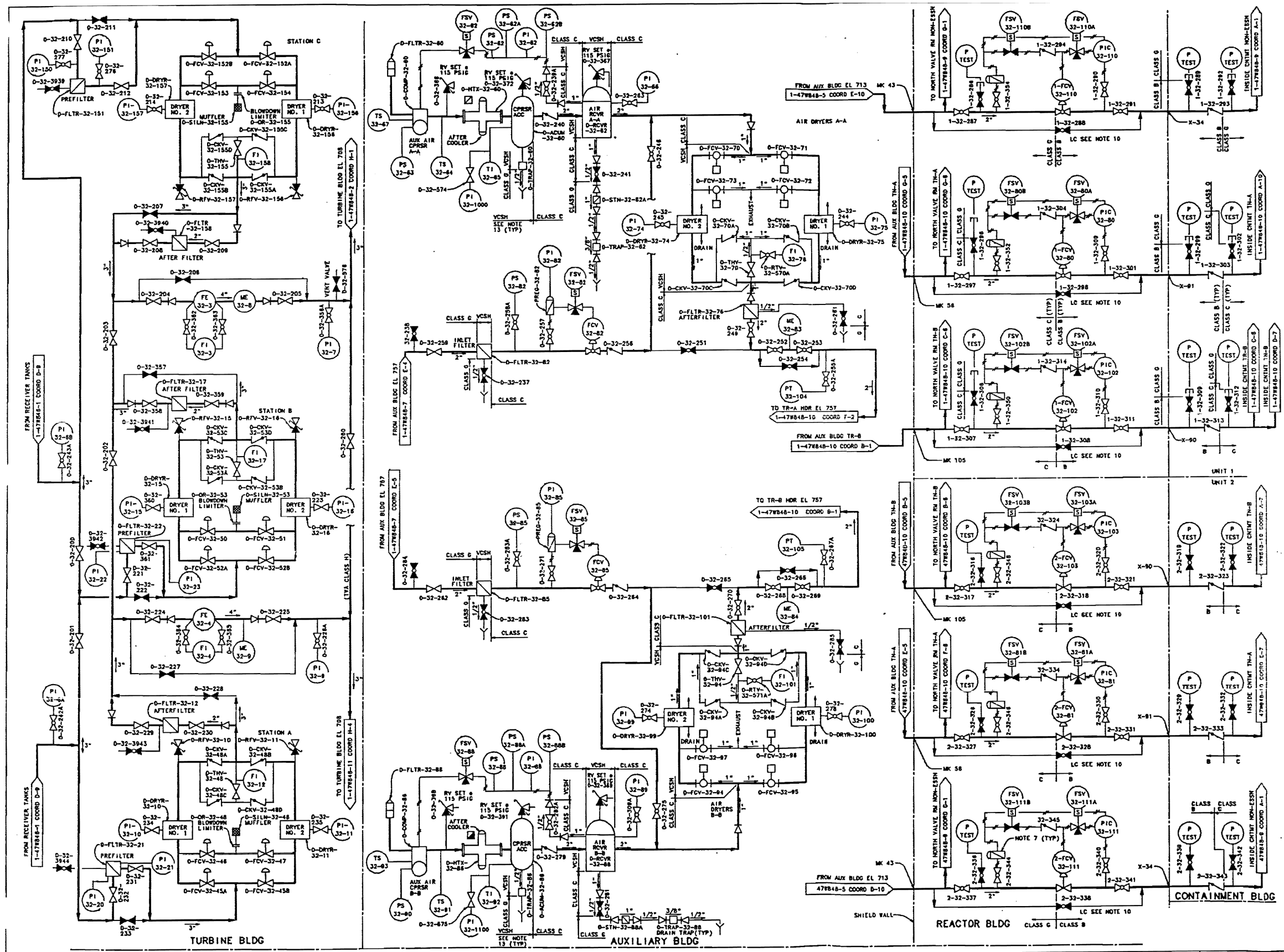
Figure 9.3-6 Powerhouse Units 1 & 2 Mechanical Flow Diagram for Control Air System
