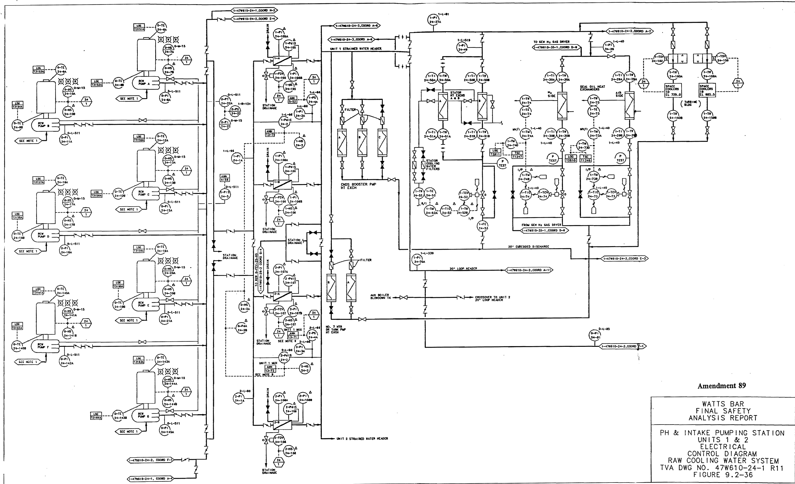
Figure 9.2-36 Powerhouse and Intake Pumping Station Electrical Control Diagram for Raw Cooling Water System
