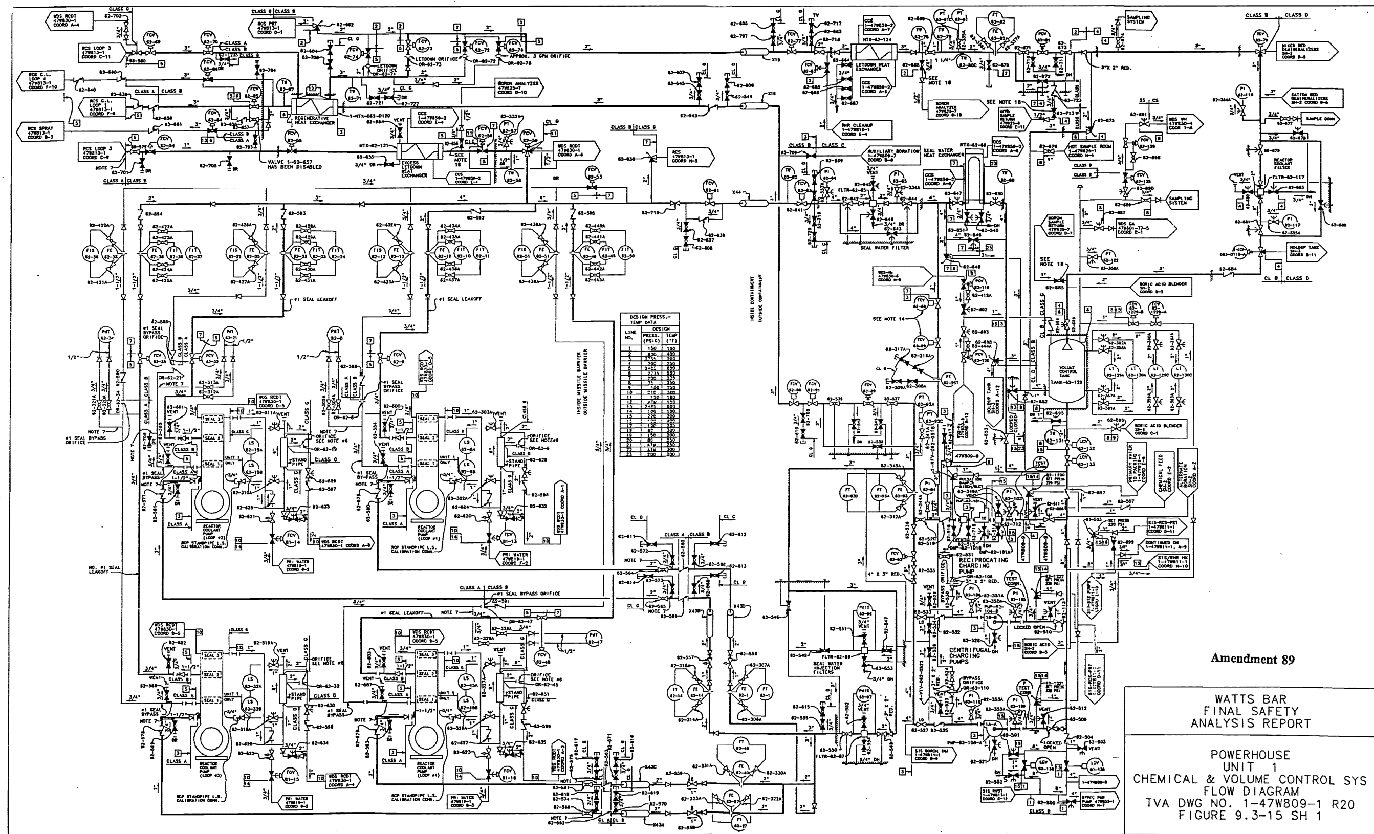
Figure 9.3-15 Powerhouse Unit 1 Chemical and Volume Control System Flow Diagram (Sheet 1)
