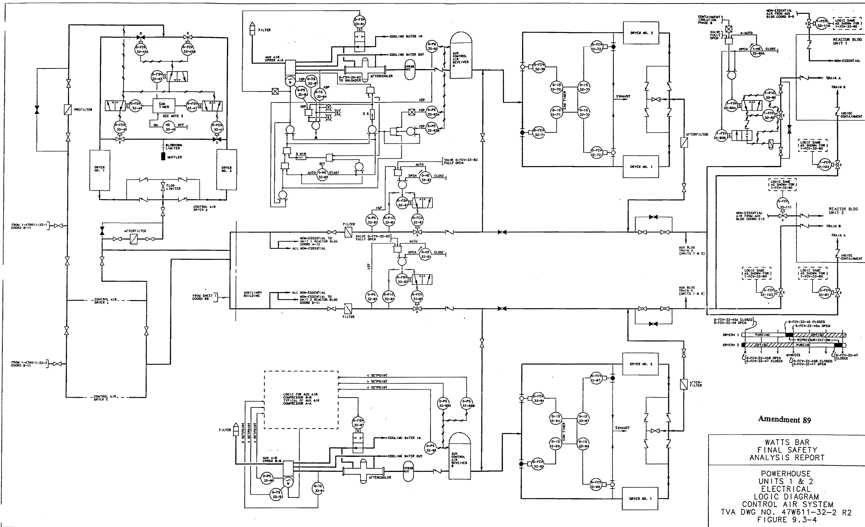
Figure 9.3-4 Powerhouse Units 1 &amp; 2 Electrical Logic Diagram for Control Air System
