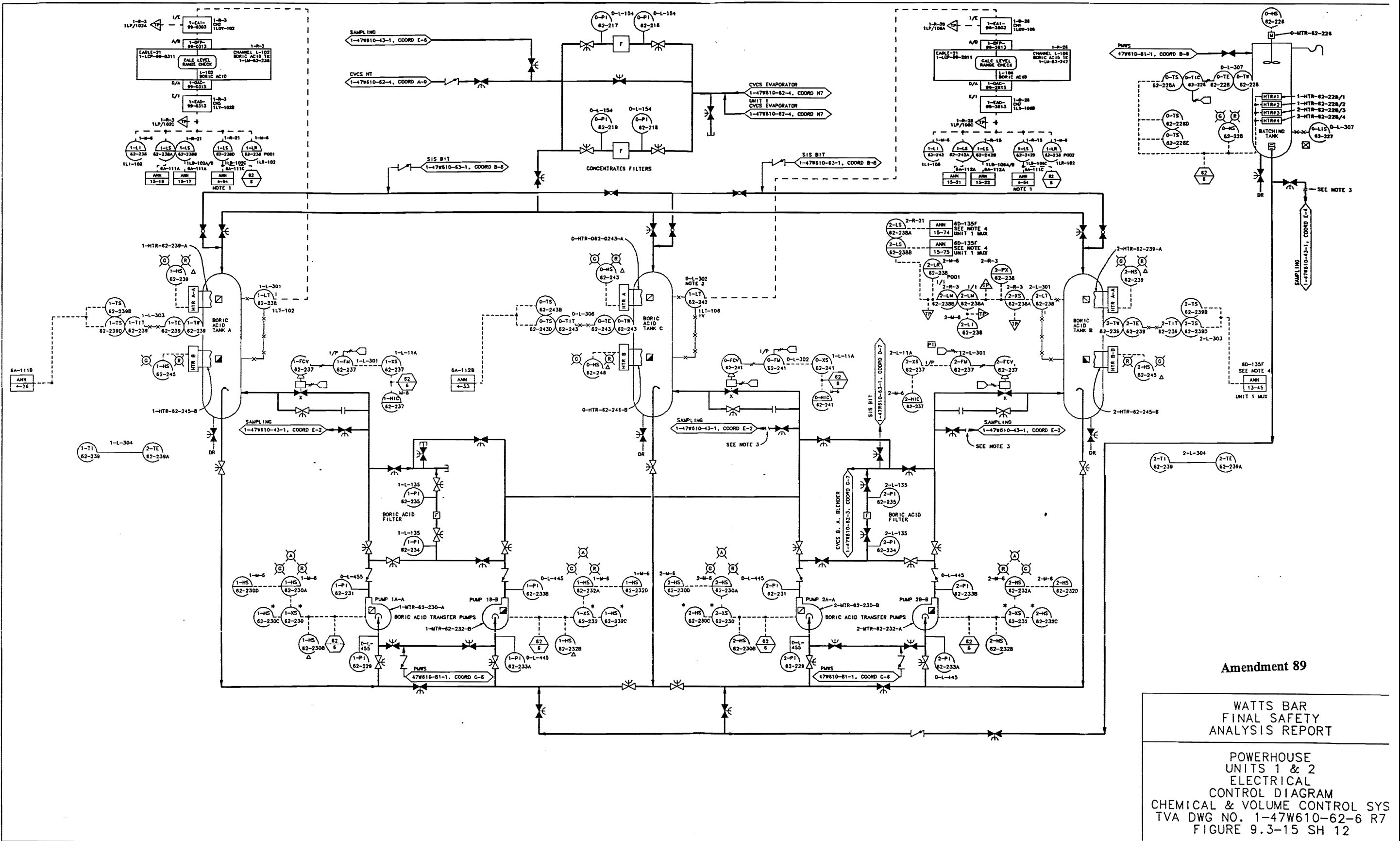
Figure 9.3-15 Powerhouse Units 1 &amp; 2 Electrical Control Diagram Chemical &amp; Volume Control Sys (Sheet 12)
