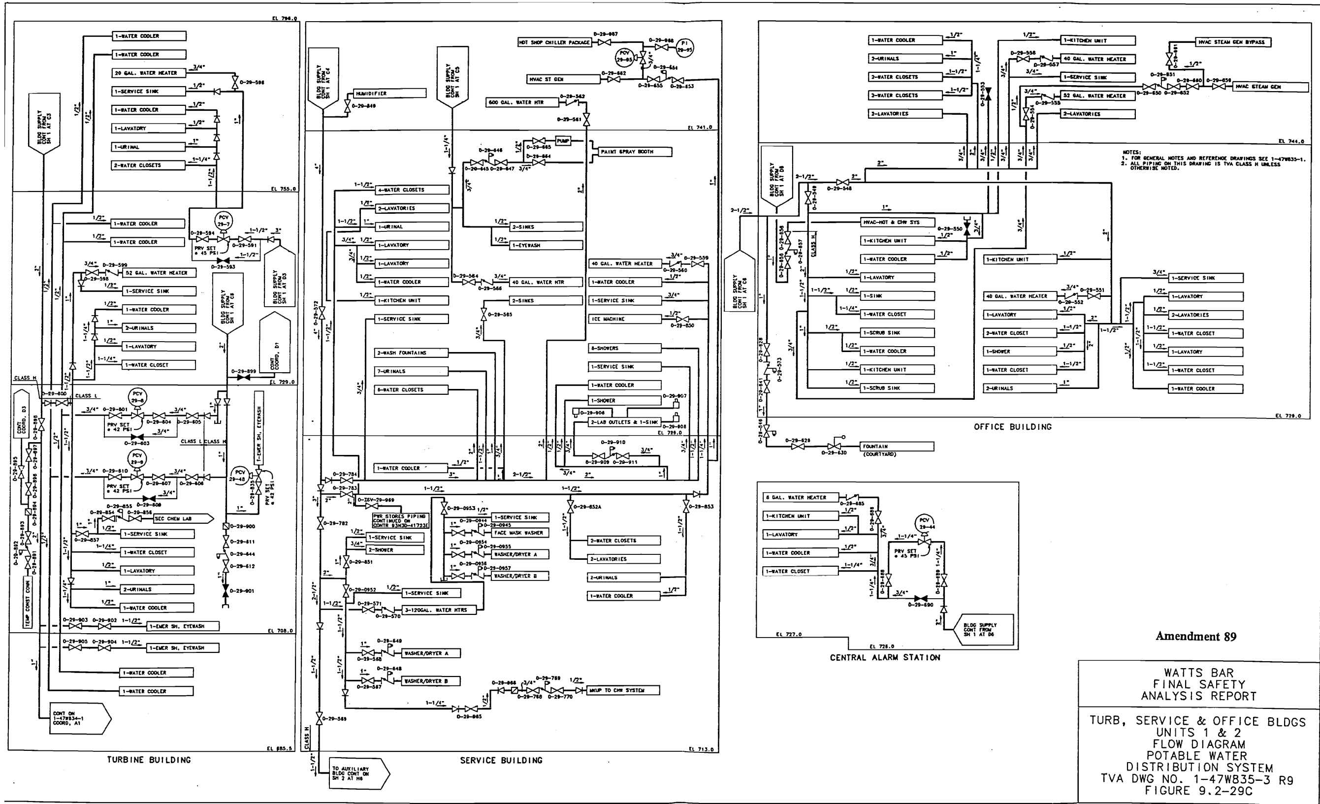
Figure 9.2-29c Turb, Service & Office Bldgs. Units 1 & 2 Flow Diagram for Potable Water Distribution System
