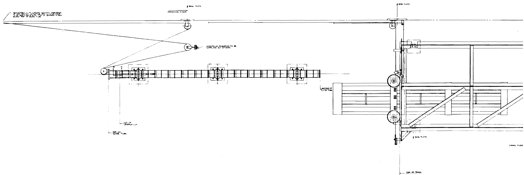
Figure 9.1-10 Rod Cluster Control Changing Fixture
