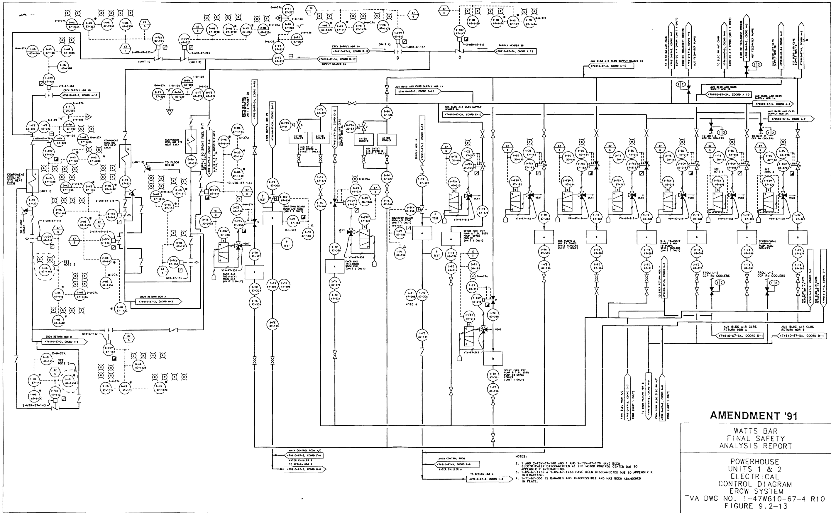
Figure 9.2-13 Powerhouse Electrical Control Diagram for Essential Raw Cooling Water System
