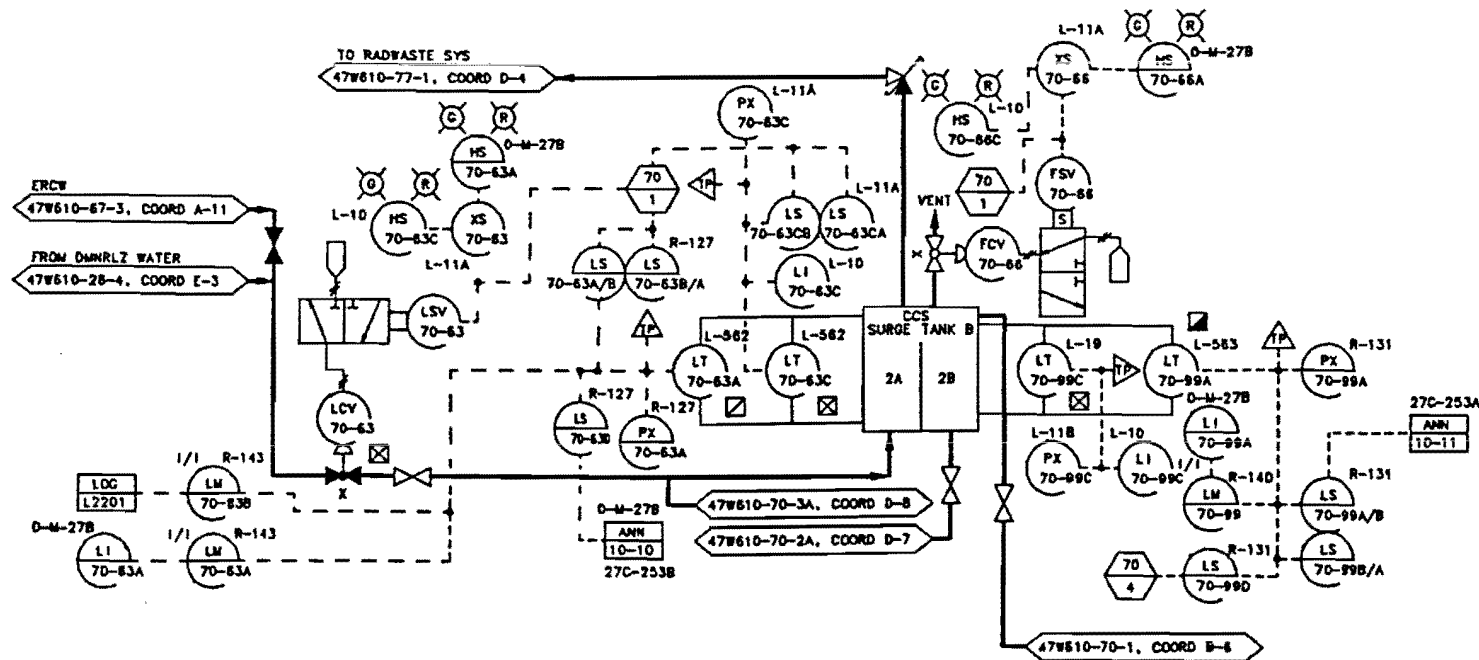
Figure 9.2-20a Powerhouse Unit 2 Electrical Control Diagram
