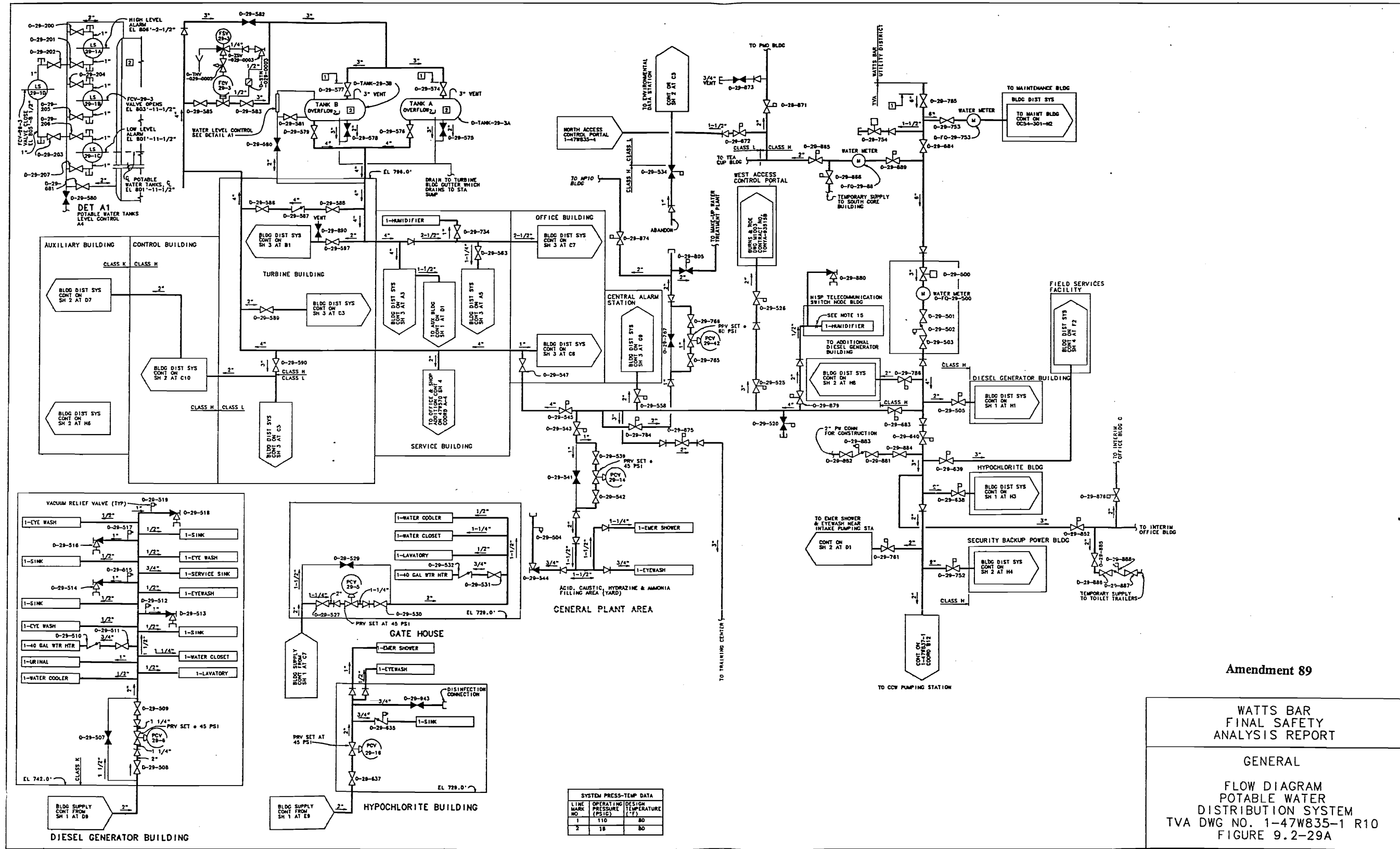
Figure 9.2-29a General Flow Diagram for Potable Water Distribution System
