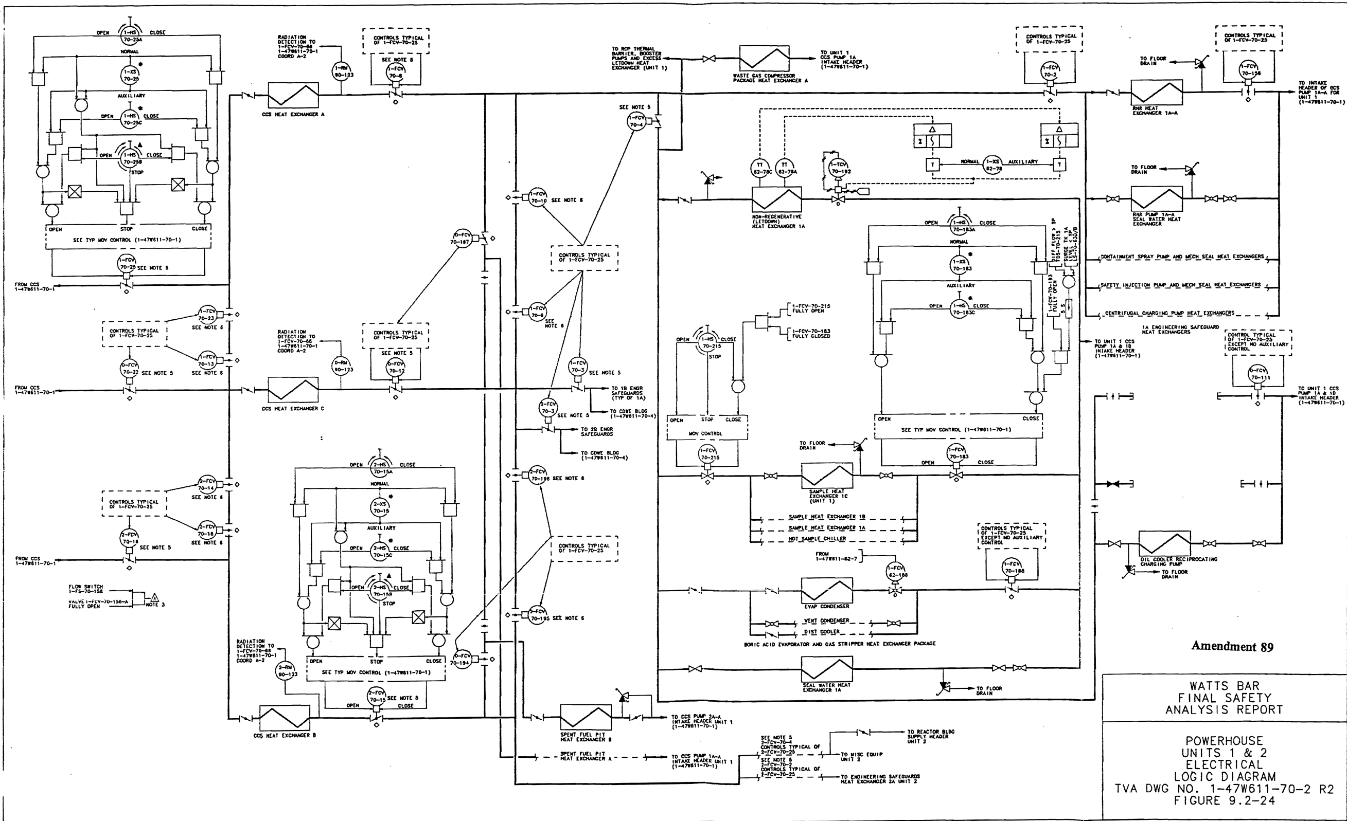
Figure 9.2-24 Powerhouse Units 1 & 2 Electrical Logic Diagram for Component Cooling Water System
