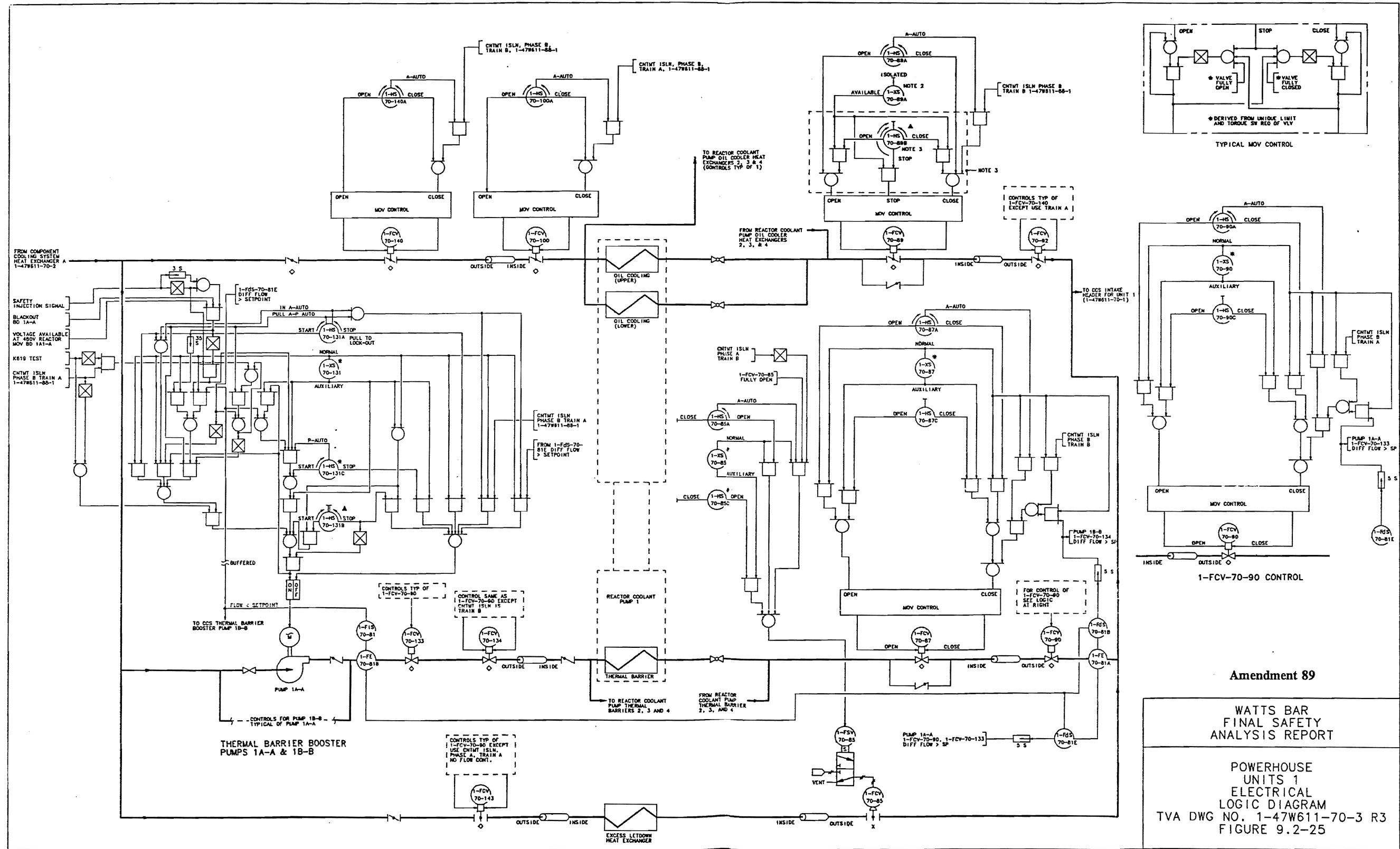
Figure 9.2-25 Powerhouse Unit 1 Electrical Logic Diagram
