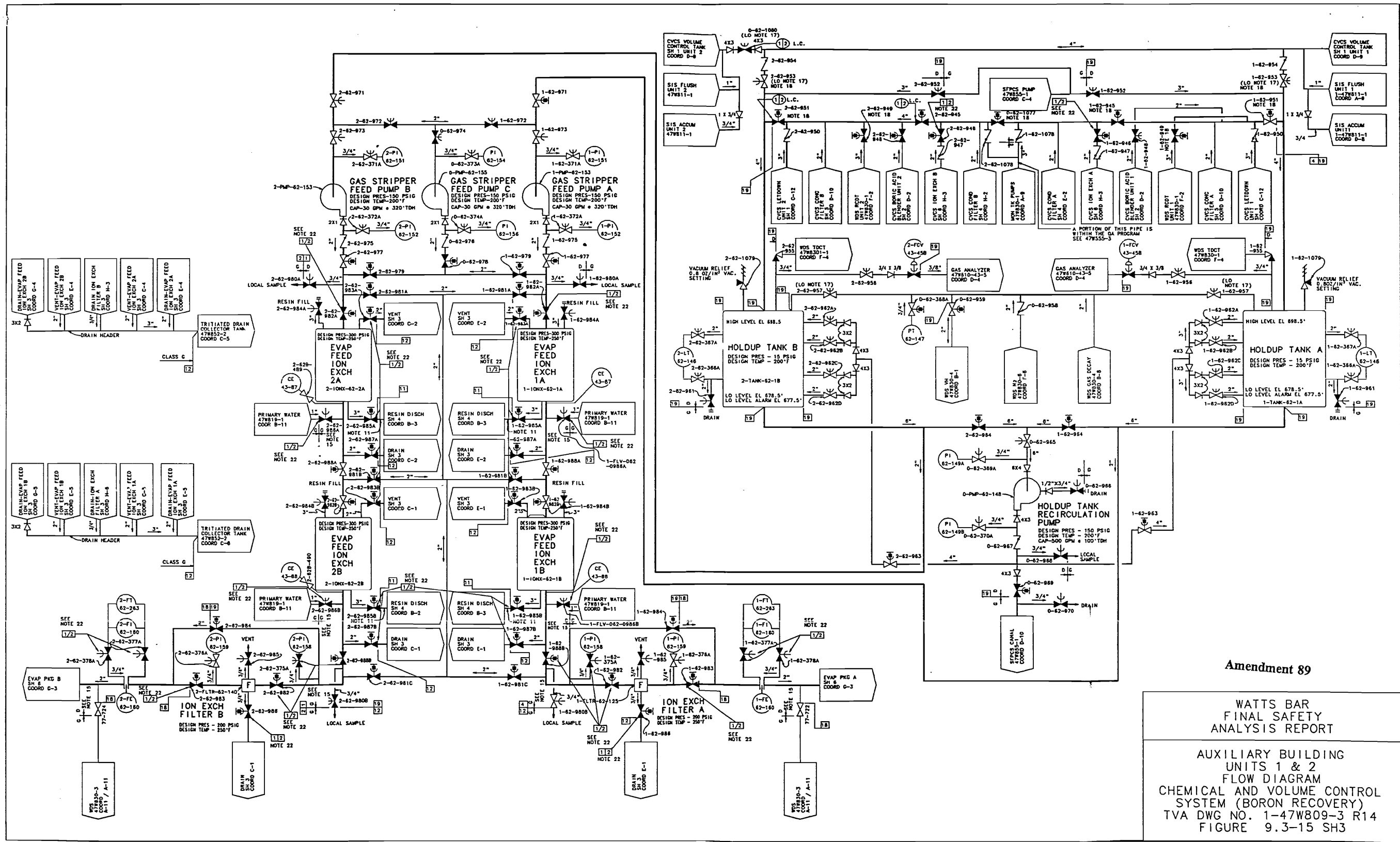
Figure 9.3-15 Auxiliary Building Units 1 & 2 Flow Diagram for Chemical and Volume Control System (Boron Recovery) (Sheet 3)
