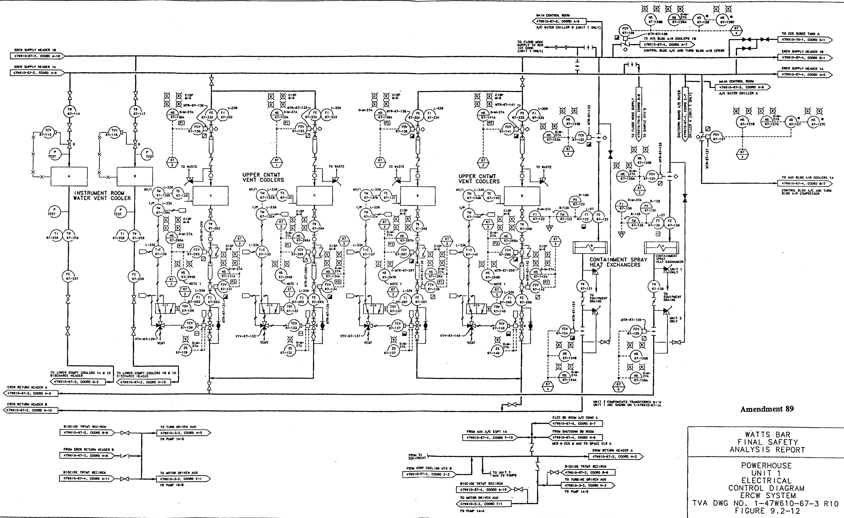
Figure 9.2-12 Electrical Control Diagram for Essential Raw Cooling Water System (Unit 1)
