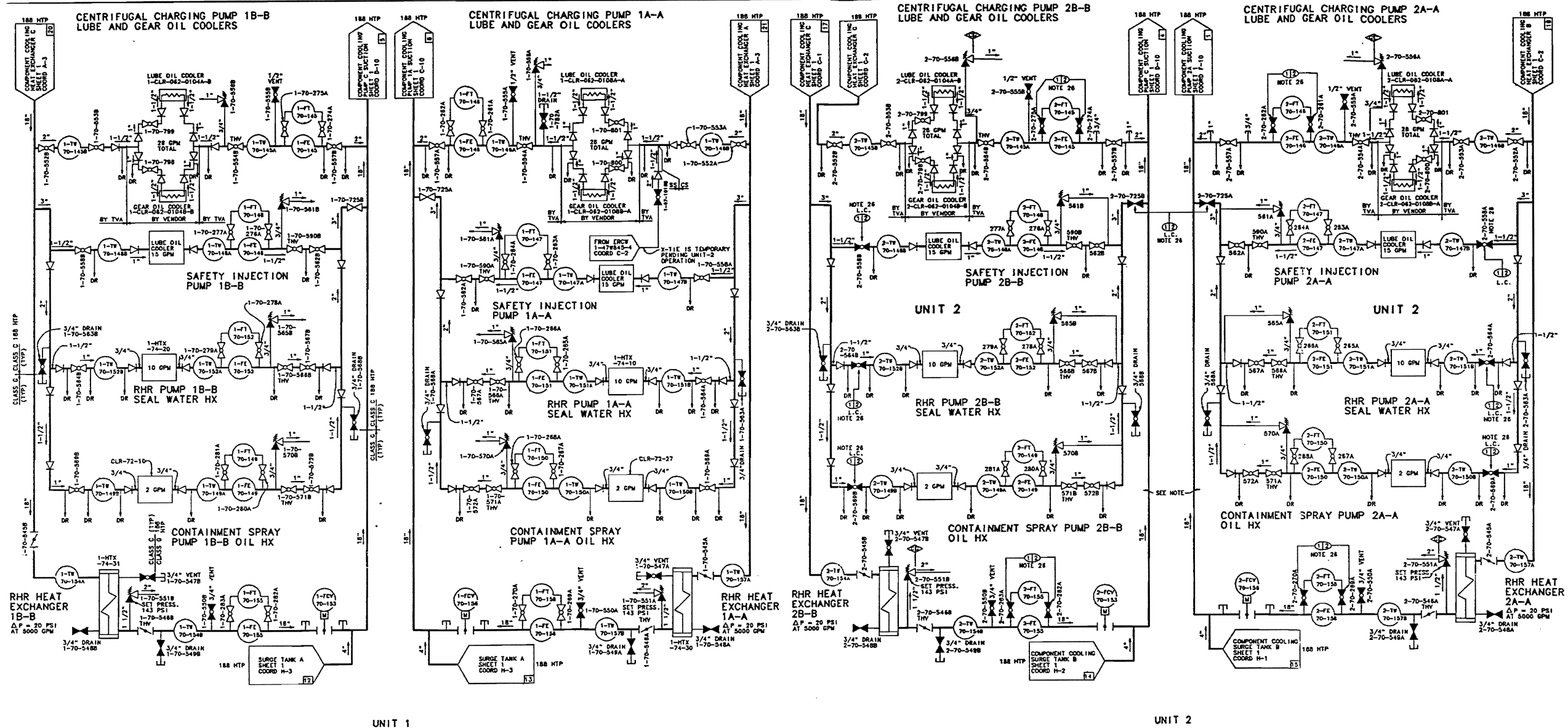
Figure 9.2-16 Powerhouse, Auxiliary Building Flow Diagram for Component Cooling Water System
