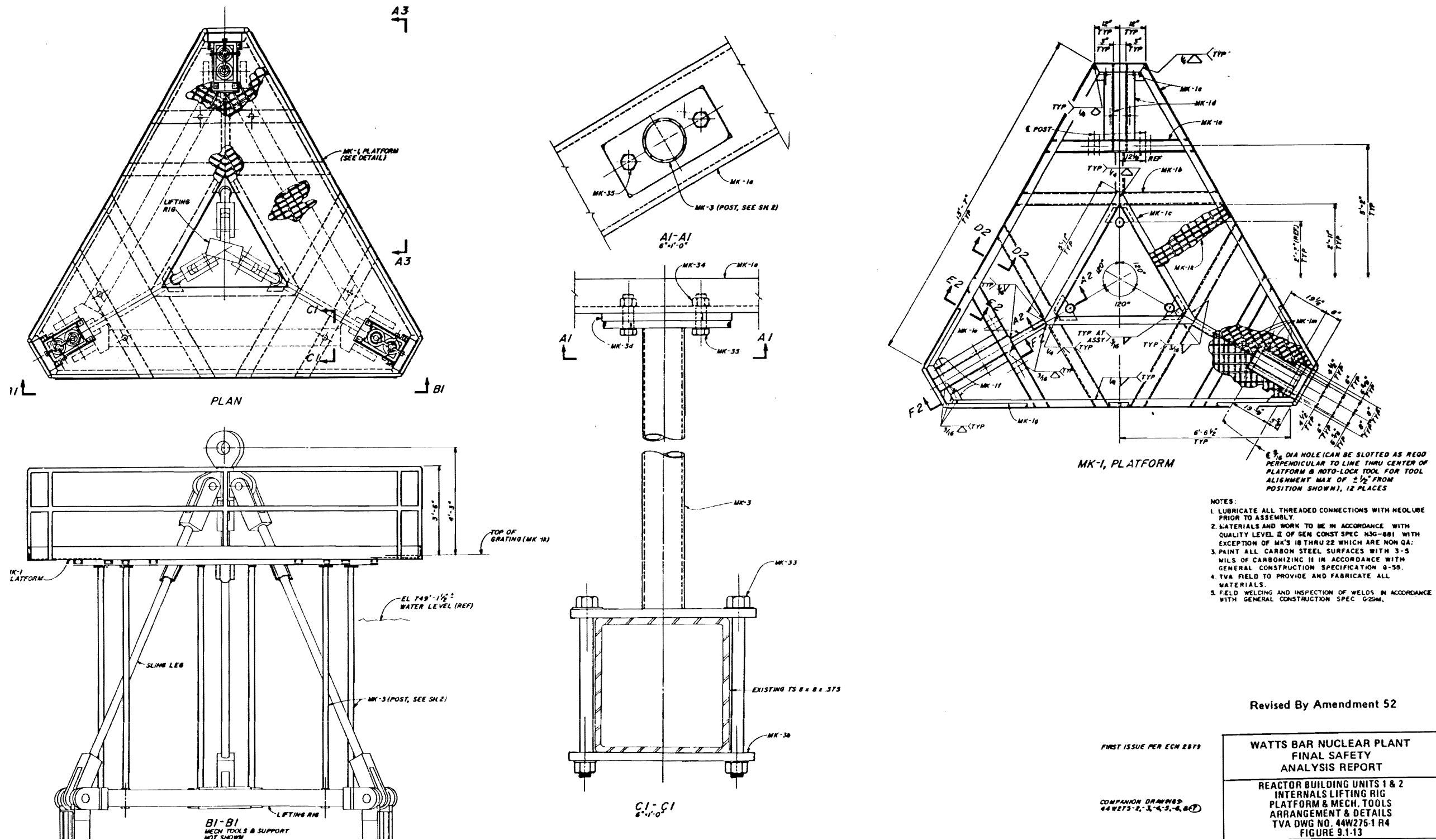
Figure 9.1-13 Reactor Building Internals Lifting Rig Platform and Mech. Tools Arrangement and Details
