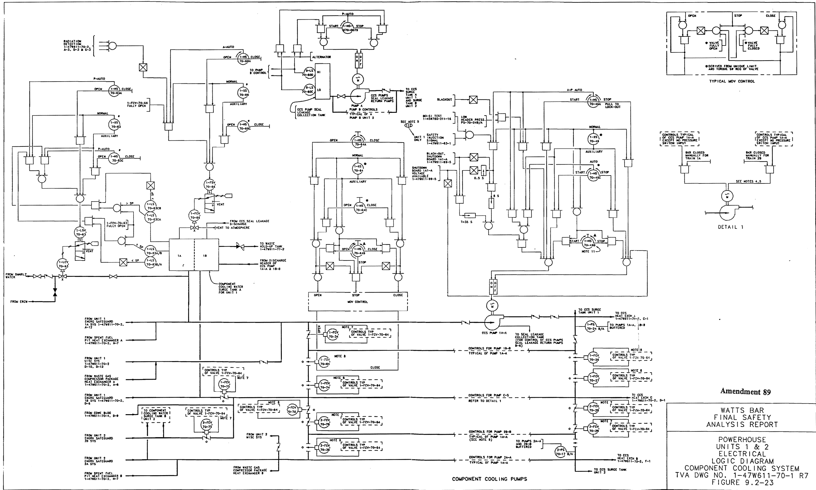
Figure 9.2-23 Powerhouse Units 1 & 2 Electrical Logic Diagram for Component Cooling System
