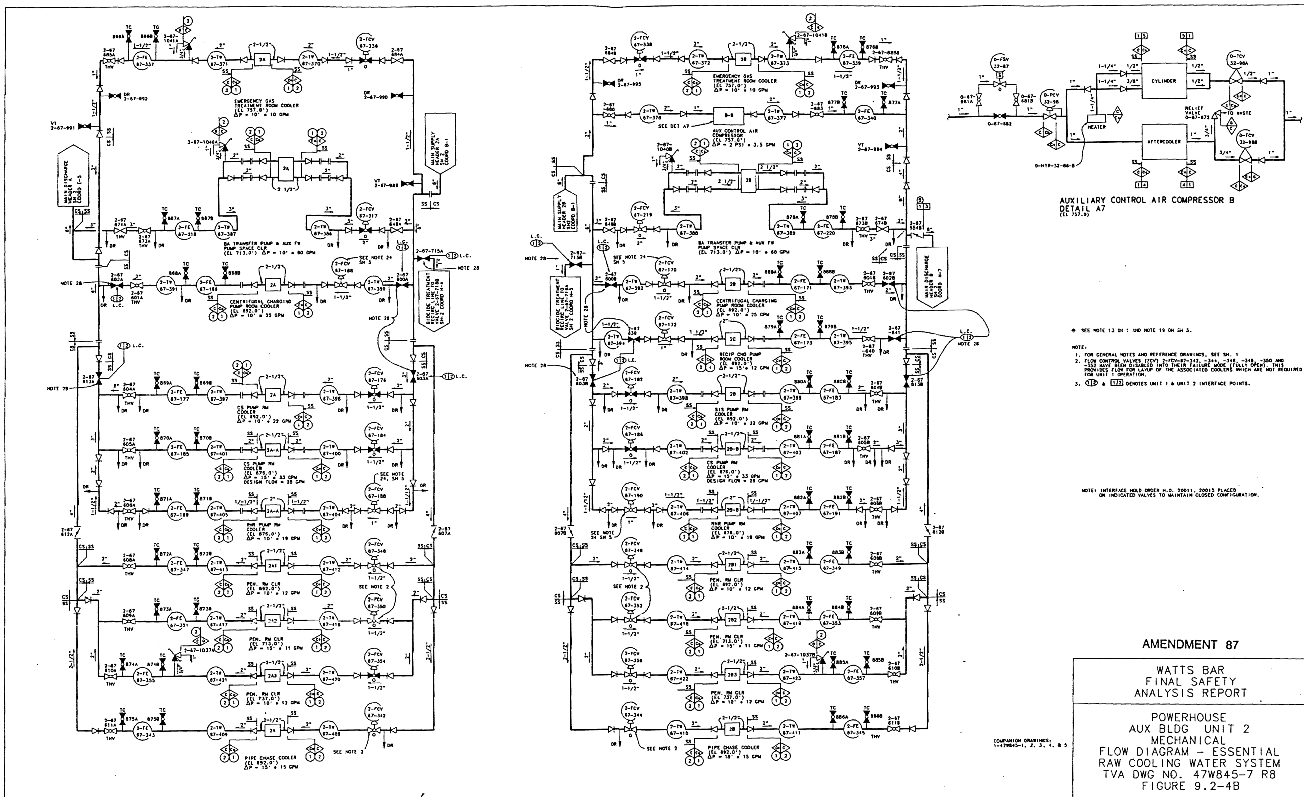
Figure 9.2-4b Powerhouse Auxiliary Building Flow Diagram for Essential Raw Cooling Water System (Unit 2)
