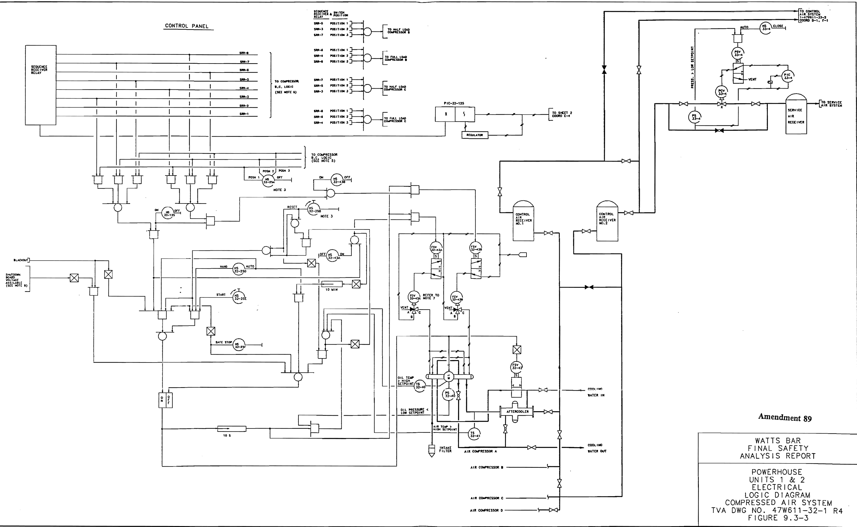
Figure 9.3-3 Powerhouse Units 1 & 2 Electrical Logic Diagram for Compressed Air System
