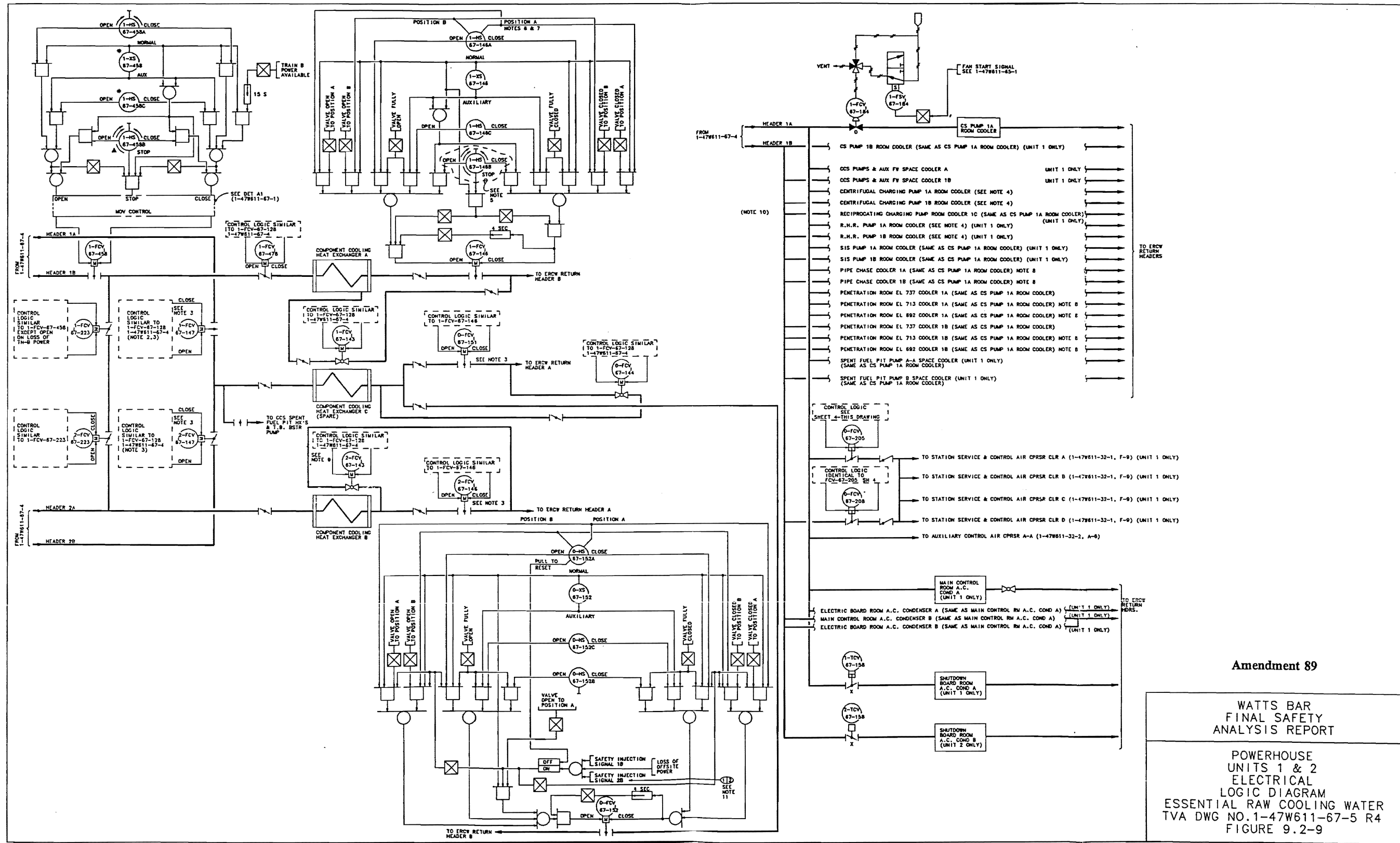
Figure 9.2-9 Powerhouse Units 1 & 2 Electrical Logic Diagram for Essential Raw Cooling Water System
