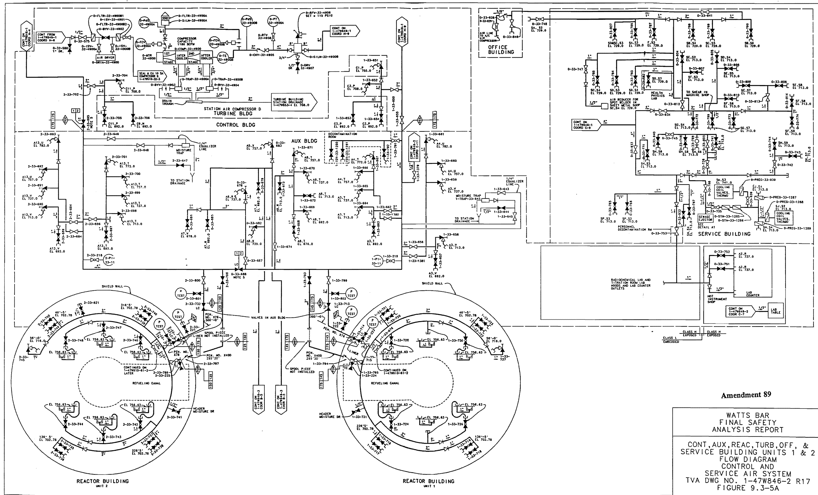
Figure 9.3-5a Control, Auxiliary, Reactor, Turbine, Office and Service Building Units 1 &amp; 2 Flow Diagram for Control and Service Air System
