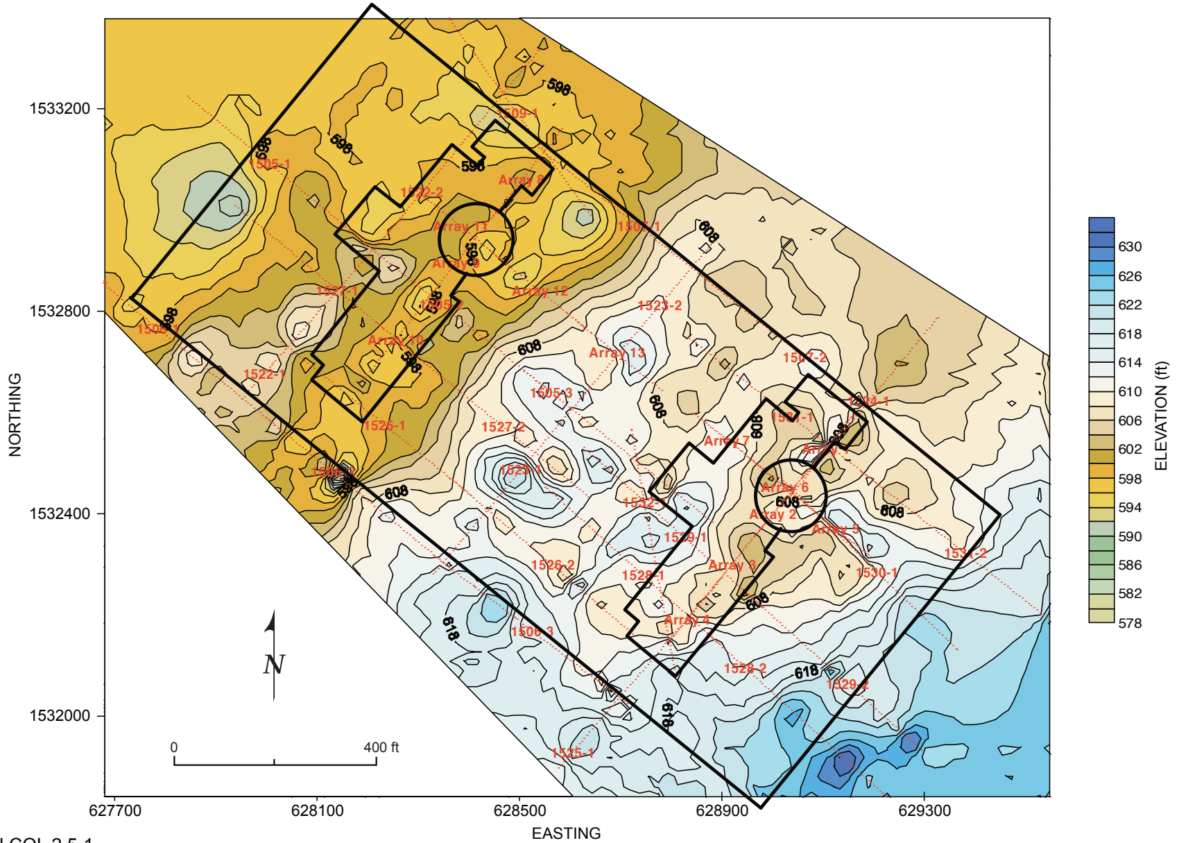
FIGURE 2.5-312 Seismic 3D Model: Top of 6,000 fps Vp Layer
