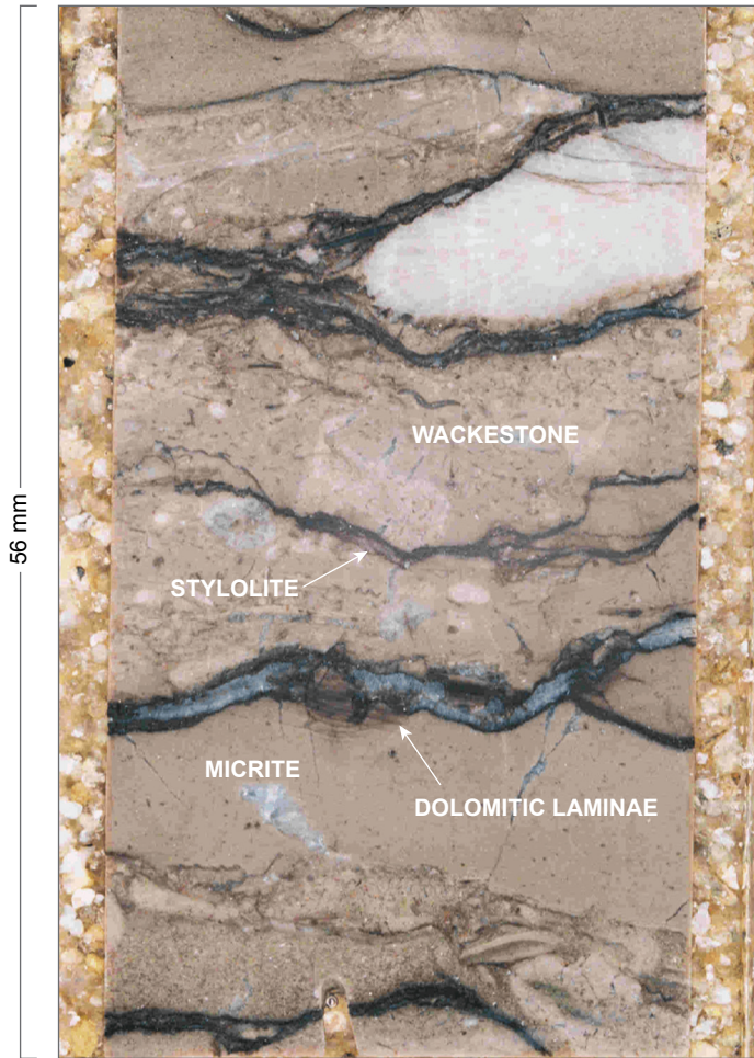
BLN-4 Limestone (micrite and wackestone) with wavy dolomitic laminae and stylolites
