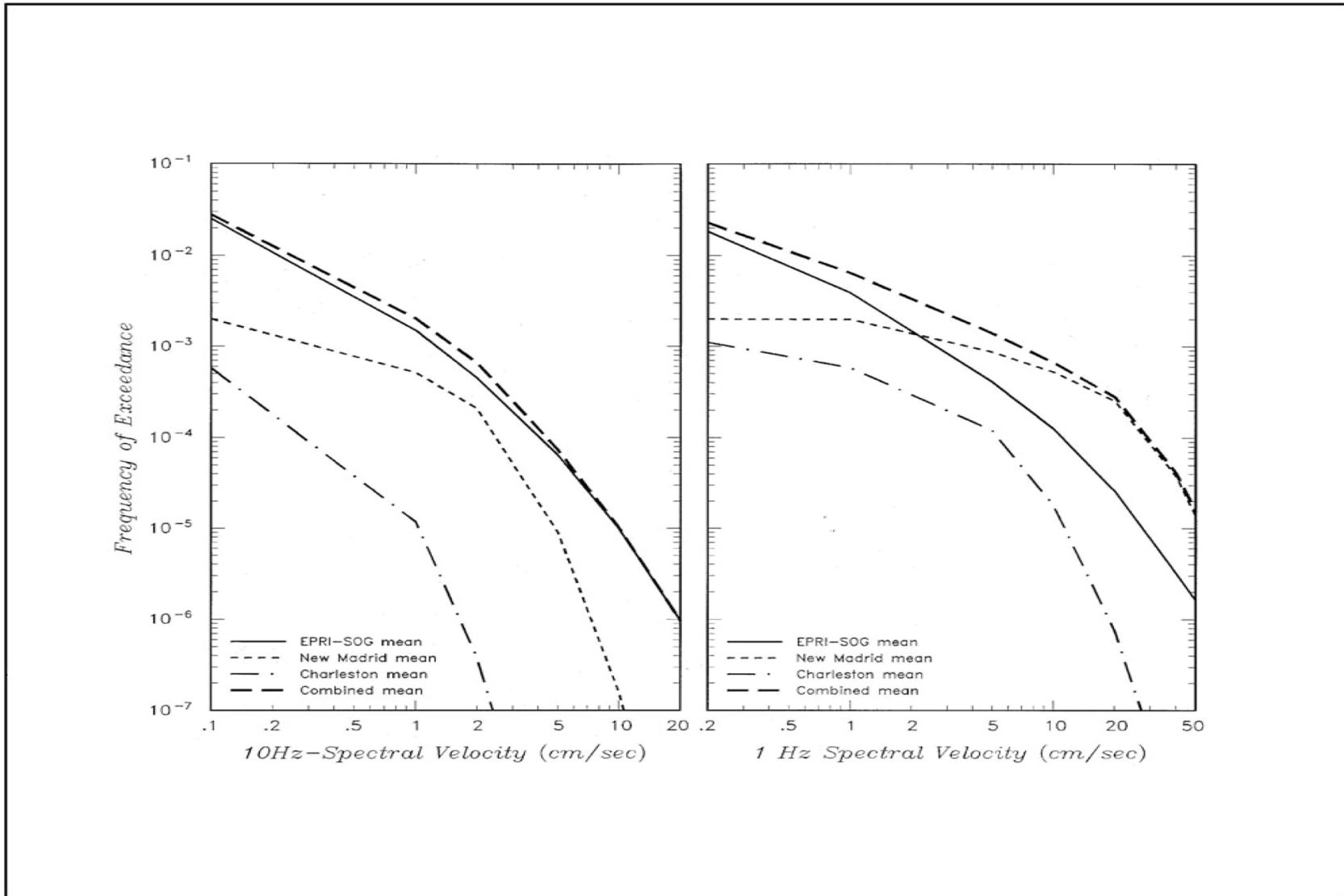
FIGURE 2.5-259 Effect of Adding Sources of Repeating Large Magnitude New Madrid and Charleston Earthquakes on the Site Hazard
