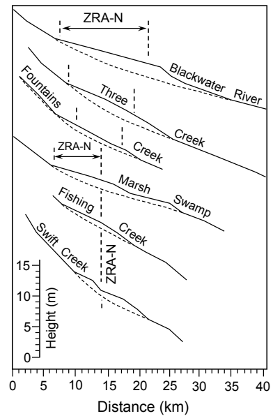
Longitudinal profiles along river flood plains that traverse the northern zone of river anomalies (ZRA-N; between vertical dashed lines along Blackwater River and Three and Fountains Creeks). The part of Marsh Swamp that parallels the ZRA-N is between the vertical dashed lines.
