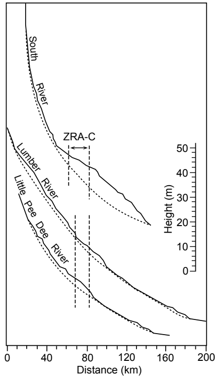
Longitudinal profiles of flood plains of South, Lumber, and Little Pee Dee Rivers. Central zone of river anomalies (ZRA-C) denoted by dashed vertical lines.
