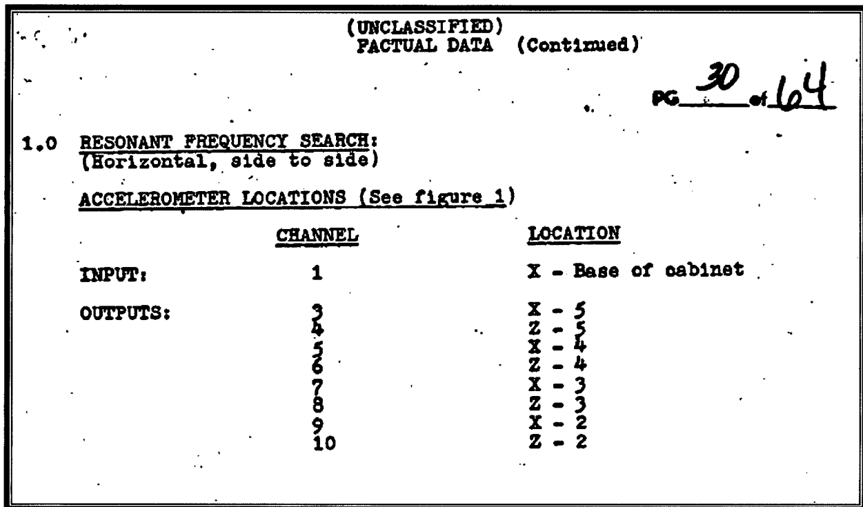
Figure 3-5. Channel assignments for Accelerometers MSFIS Cabinet (Reference 1).
