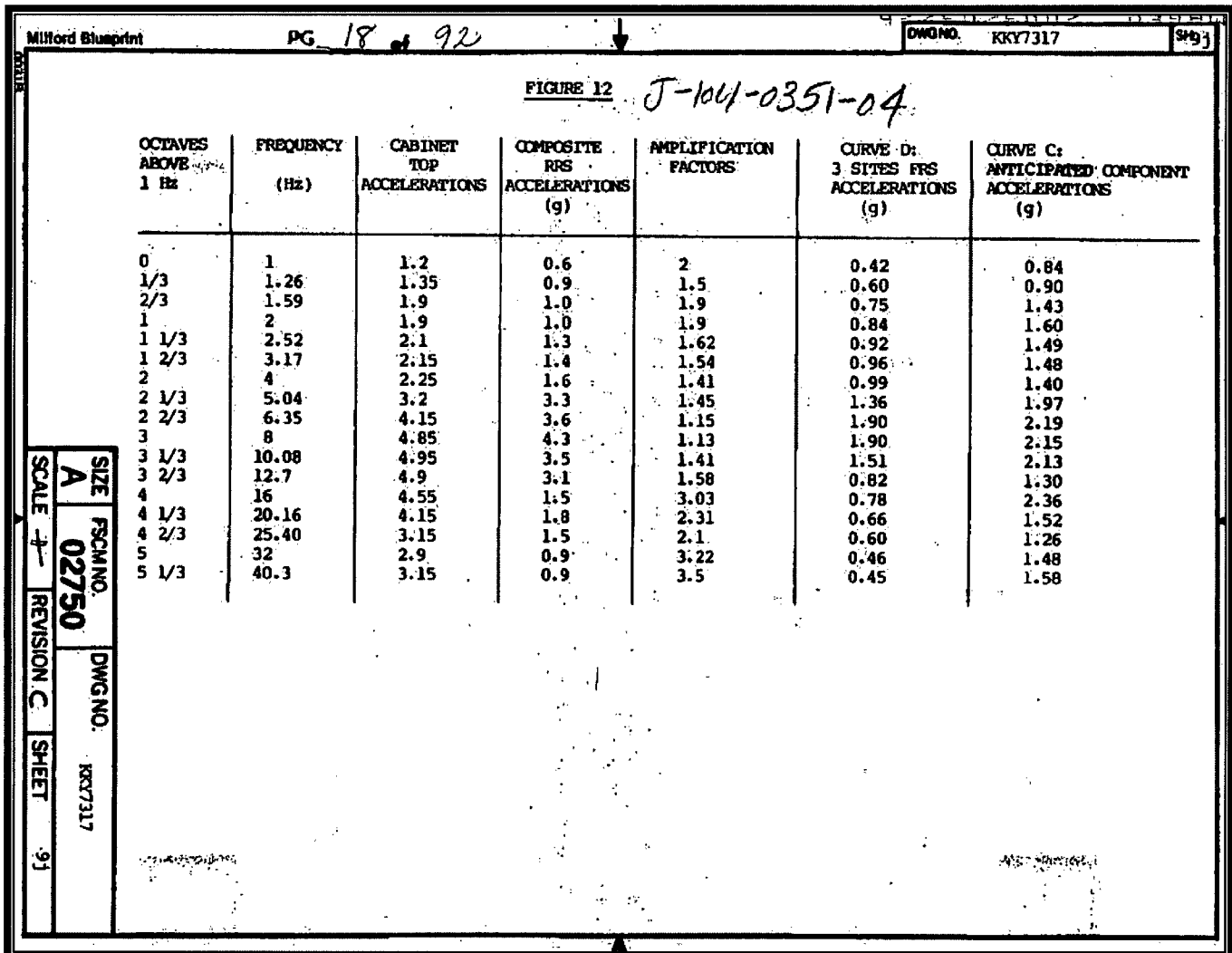
Figure 3-7. Calculated Amplification Factors from Reference 2.
