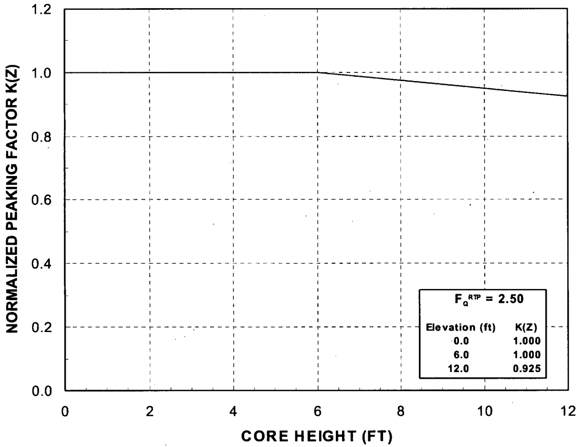
Figure 2.6 K(Z) - Normalized Peaking Factor Vs. Core Height
