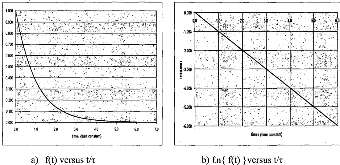
Figure 3: Plot of Exponential Function
