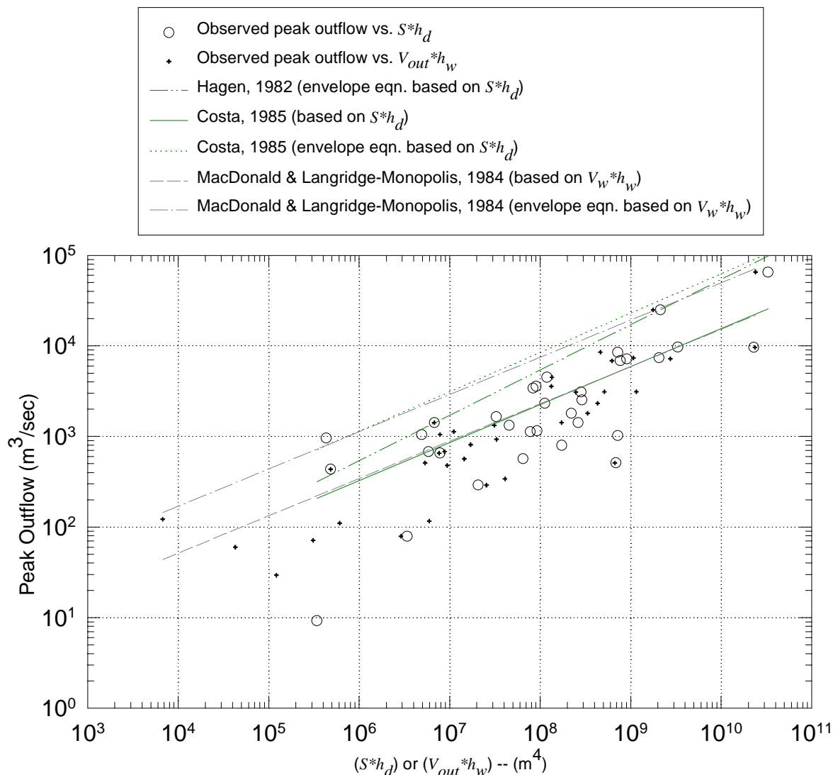
Figure 15. — Comparison of case study data and proposed relations for peak outflow as a function of the product of height and storage parameters.
