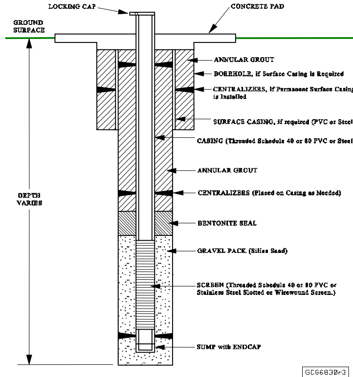
Attachment 2 Figure 1, Piezometer and Monitoring Well Construction Diagram
