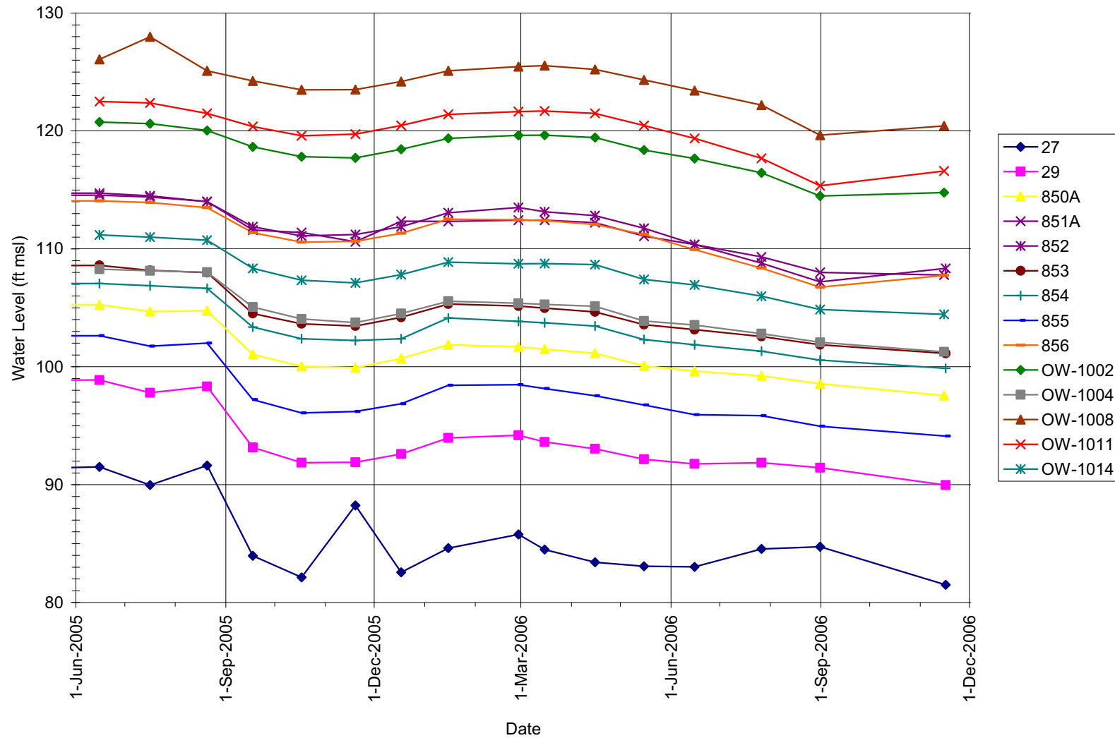
Figure 2.3.1-34 Tertiary Aquifer: June 2005 - November 2006 Hydrographs
