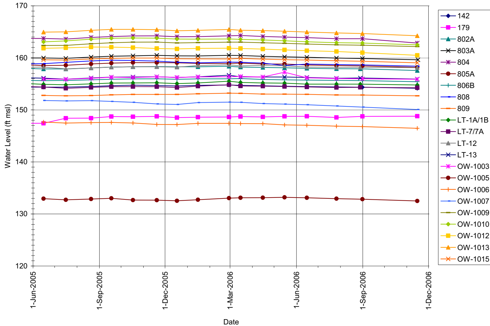
Figure 2.3.1-32 Water Table Aquifer: June 2005 – November 2006 Hydrographs
