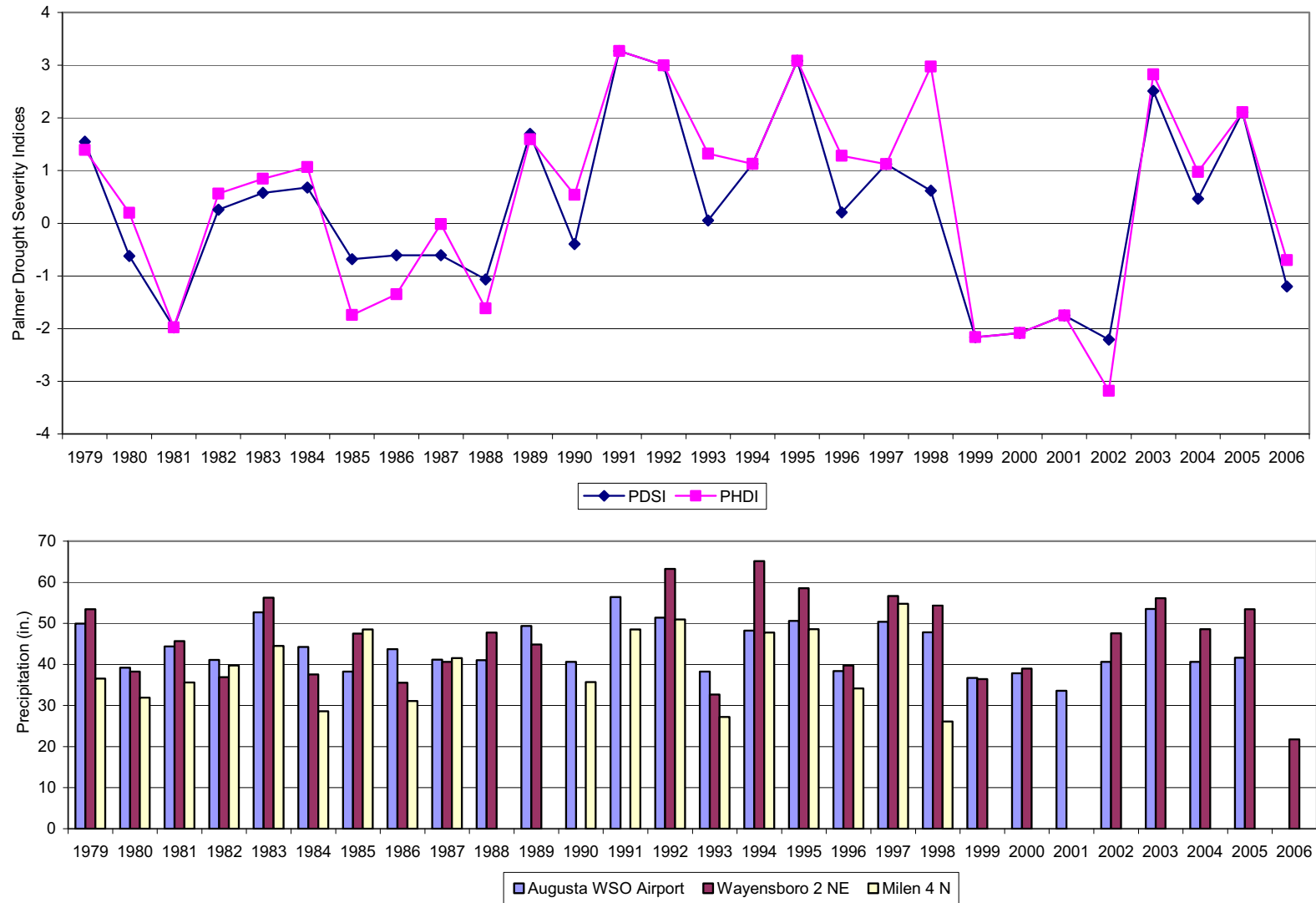
Figure 2.3.1-31 Average Annual PDSI and PHDI for Georgia and Total Annual Precipitation for the Period 1979–2006
