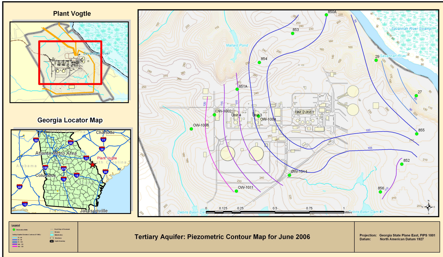
Figure 2.3.1-27 Tertiary Aquifer: Piezometric Contour Map for June 2006
