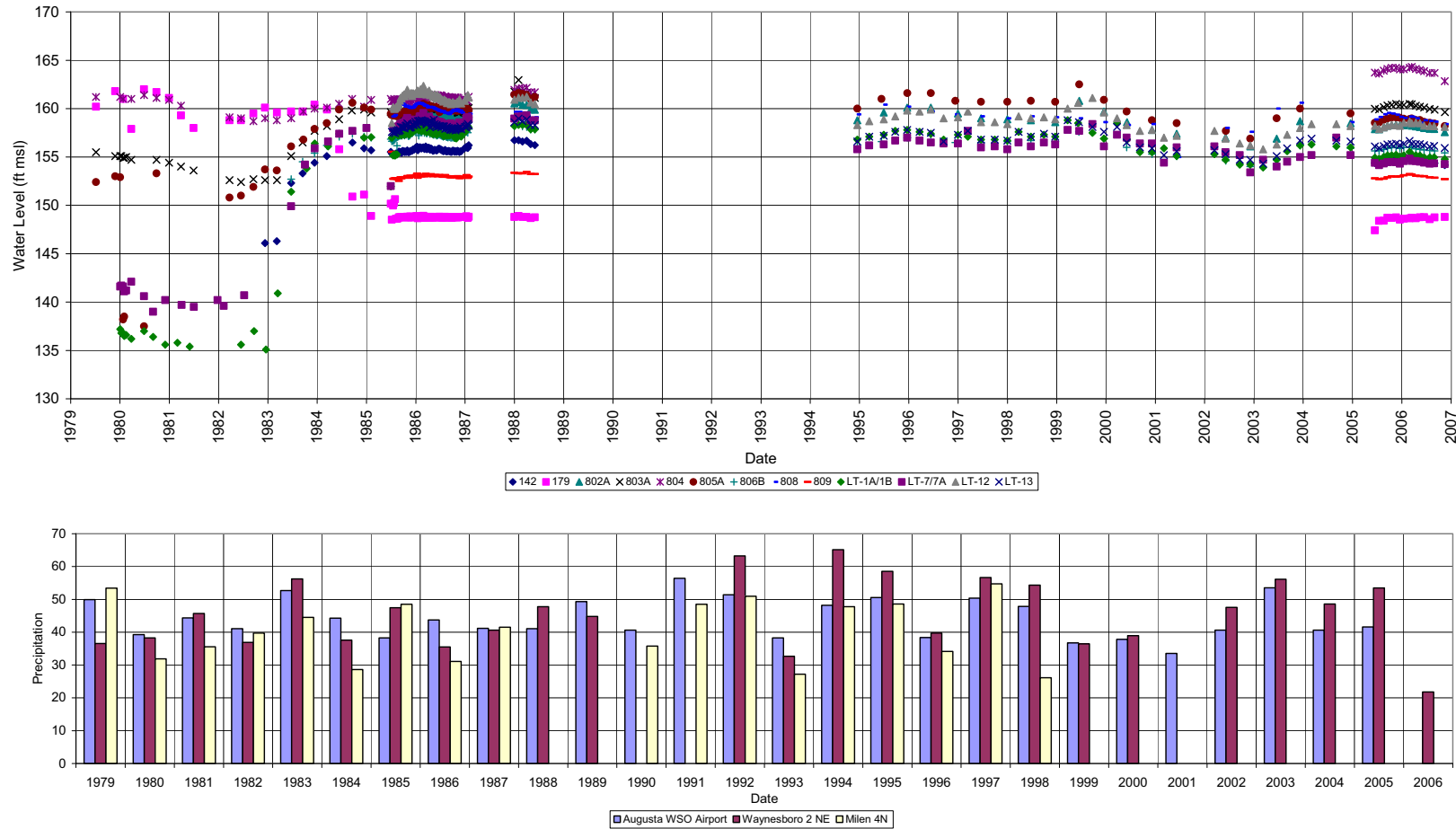
Figure 2.3.1-30 Water Table Aquifer: 1979-2006 Hydrographs
