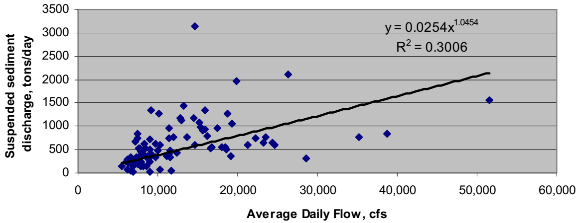
Figure 2.3.1-28 Average Daily Suspended Sediment Load For Savannah River at Clio, Georgia (USGS Gage No. 2198500)
