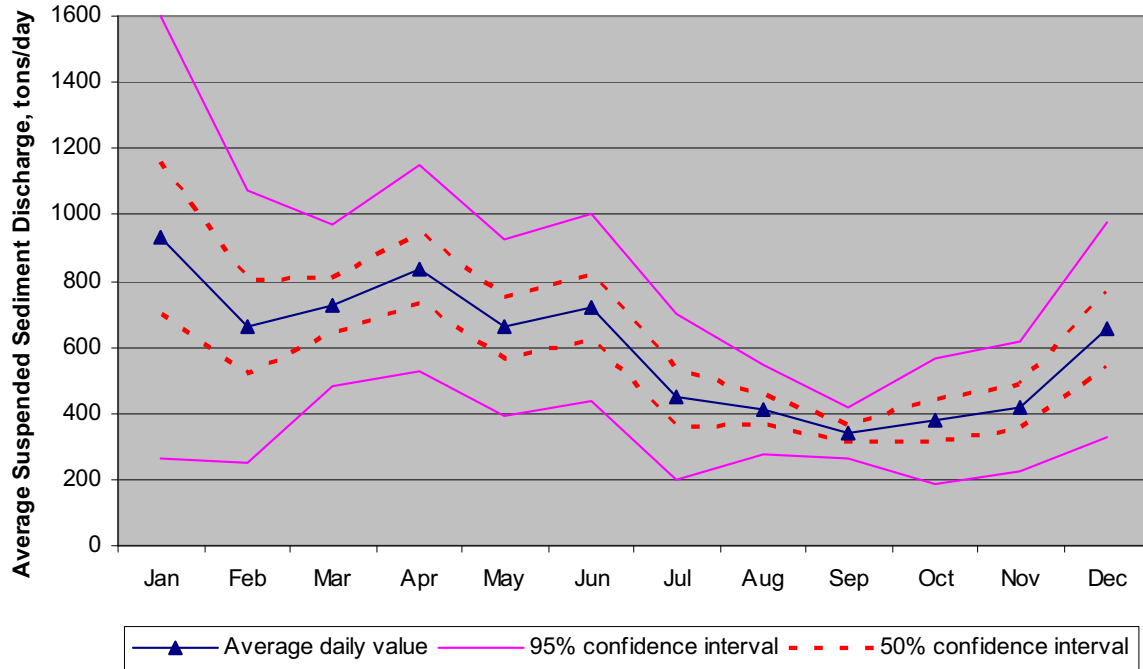
Figure 2.3.1-29 Average Monthly Suspended Sediment Discharge Measured on the Savannah River at Clio, Georgia (USGS Gage No. 2198500)
