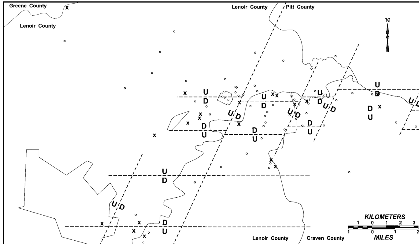
Northeast-southwest trend overprints the Paleocene east-west fault trend. U is upthrown, D is downthrown.
