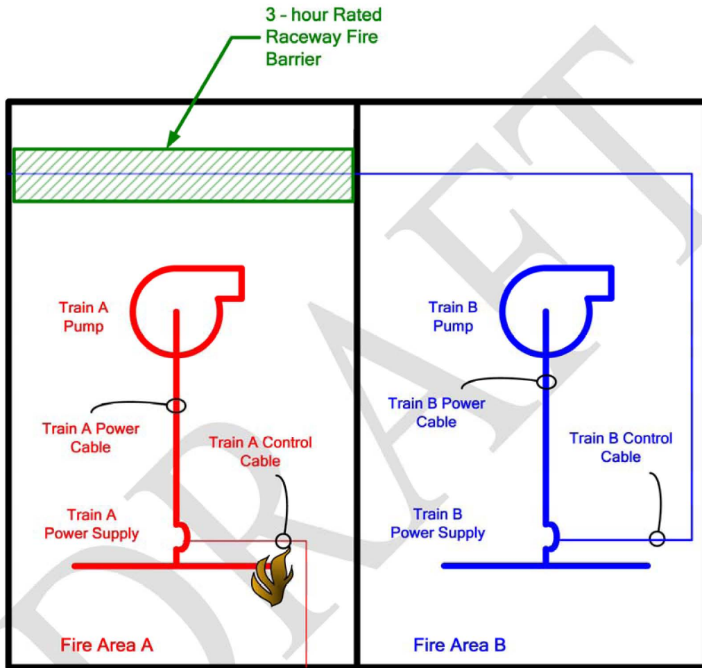
Figure E-3 Allowed Operator Manual Action in Fire Area Meeting 10 CFR 50, Appendix R,
