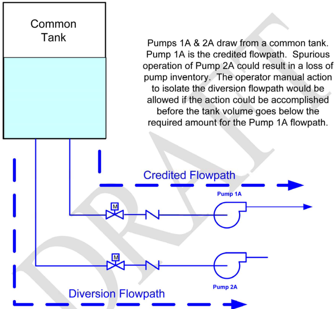
Figure E-4 Allowed Operator Manual Action – In Credited Success Path – Common Tank Suction
