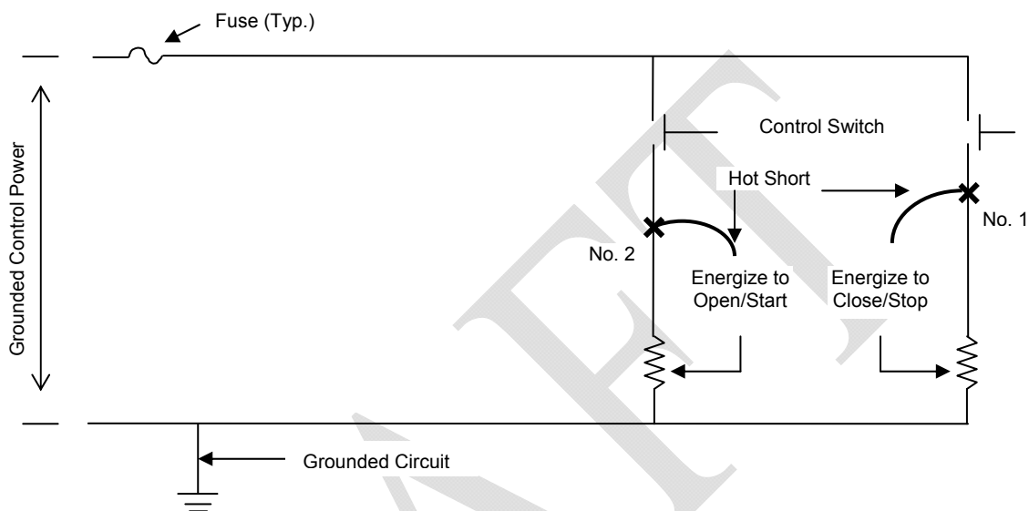
Figure 3.5.2-4 Hot Short (Grounded Control Circuit)
