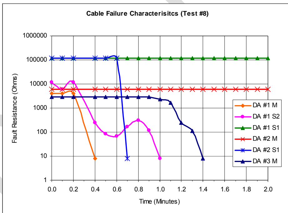
Figure B.1-4 Fault Resistance for Fire-Induced Cable Failure
