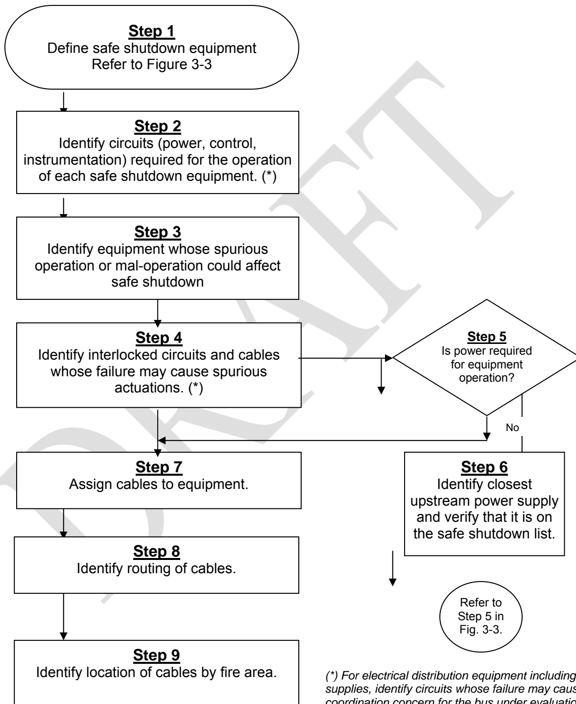
Figure 3-4 Safe Shutdown Cable Selection
