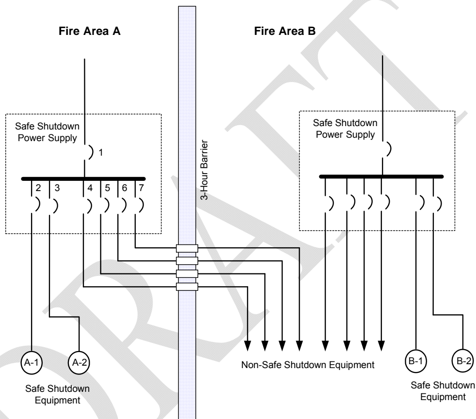
Figure B.1-1 Example MHIF Sequence
