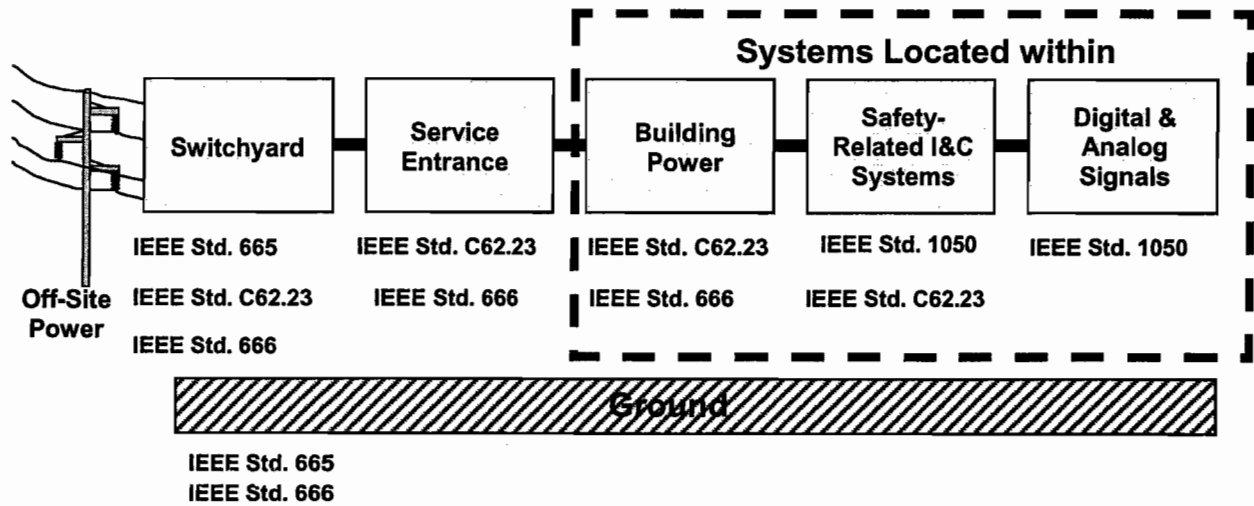
Figure 10. Overview of lightning protection standards for generating stations.
