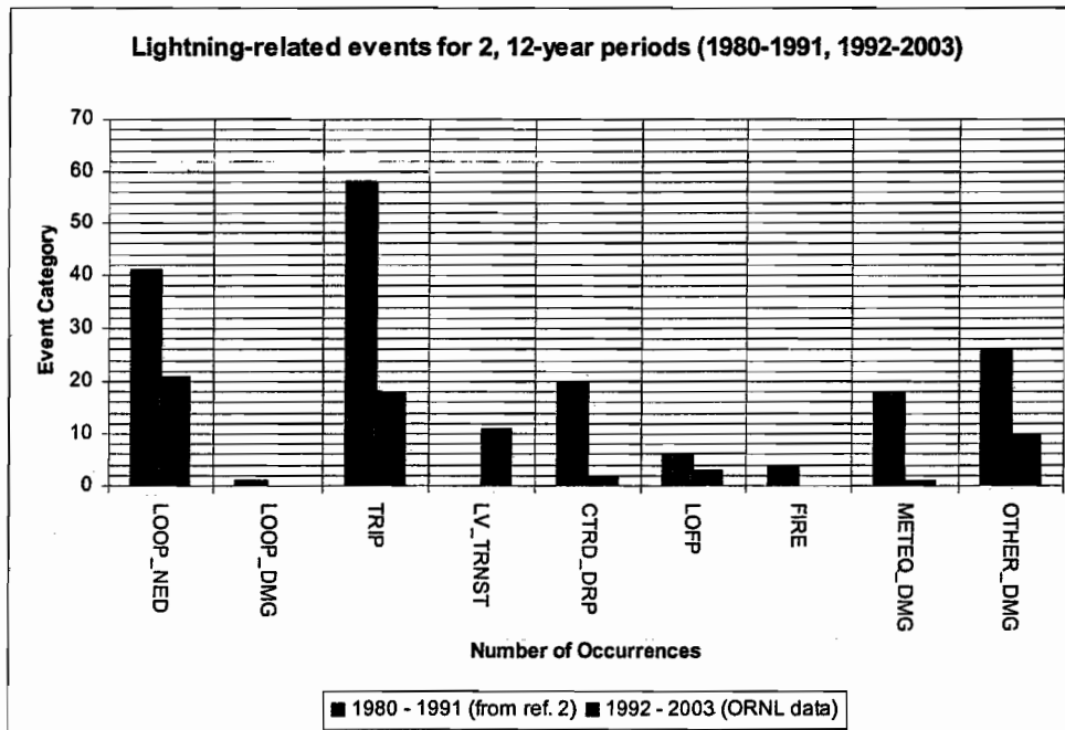
Figure 4. Lightning-related events for two 12-year periods (1980–1991, 1992–2003)
