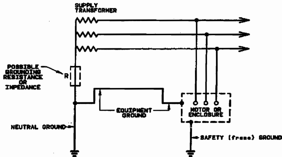
Figure 11. Three types of grounding covered by IEEE Std 665.
