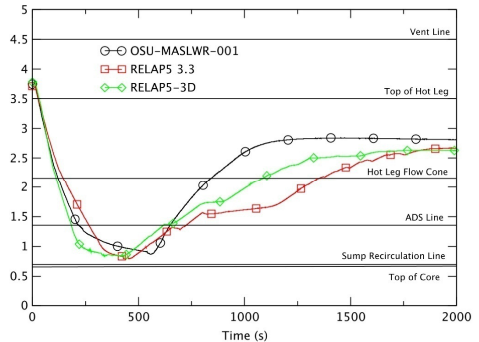
COLLAPSED DOWNCOMER LIQUID LEVEL
