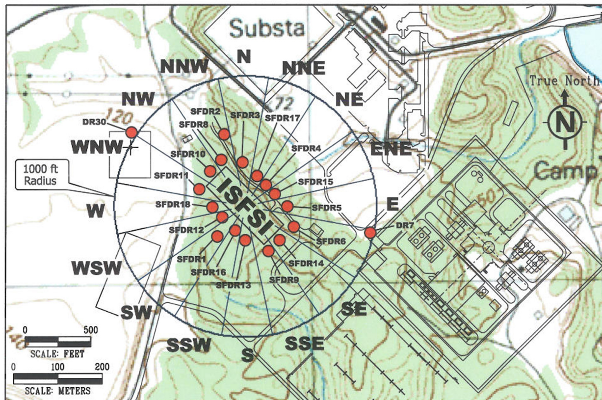
Figure 4.5-9—ISFSI TLD Locations
