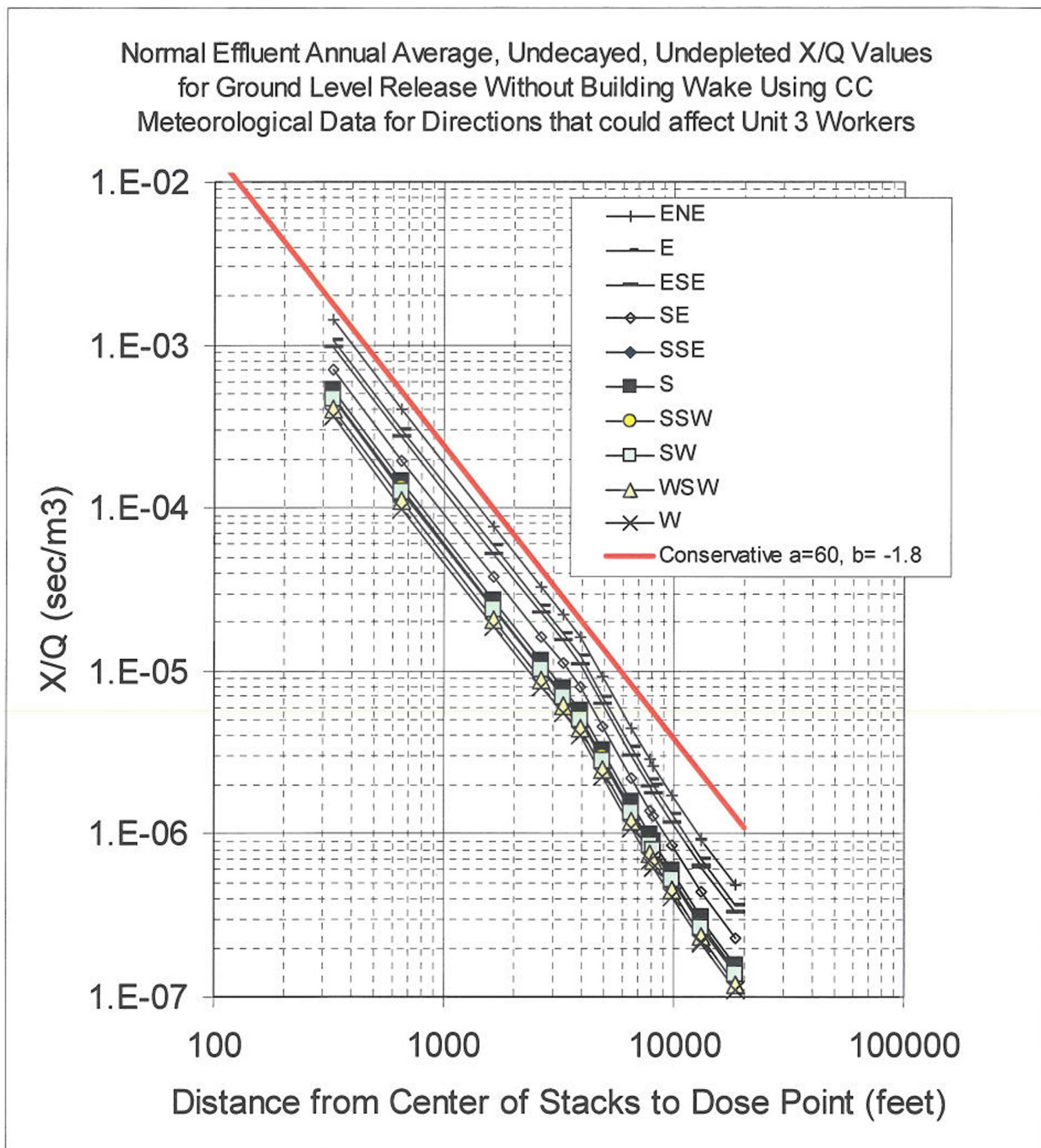
Figure 4.5-8—{Bounding Annual Average X/Q in CCNPP Unit 3 Direction}
