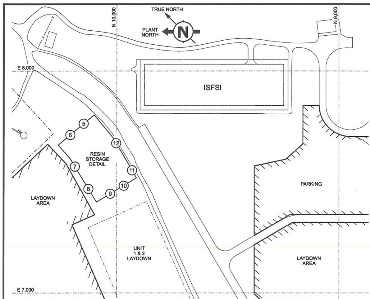
Figure 4.5-11— {Resin Area TLD Locations}
