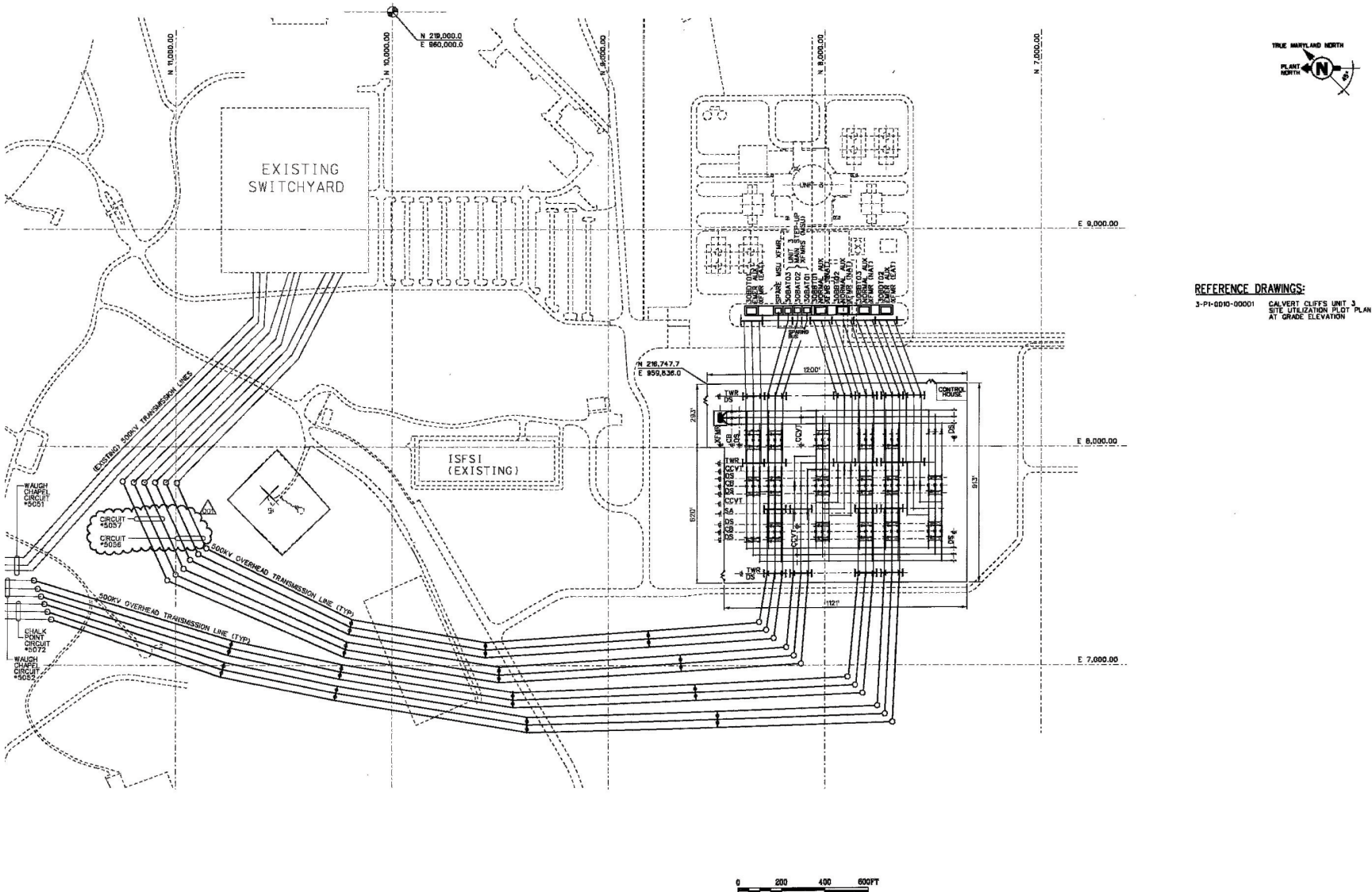
Figure 8.2-1—{CCNPP Unit 3 500kV Switchyard and Transmission Line Layout}
