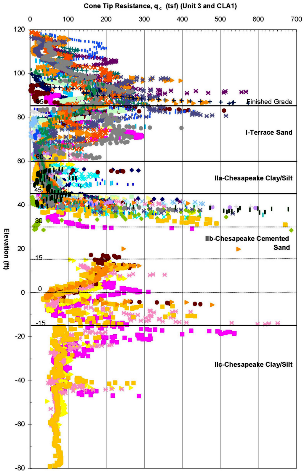
Figure 2.5-113—{Measured CPT TIP Resistance Values}
