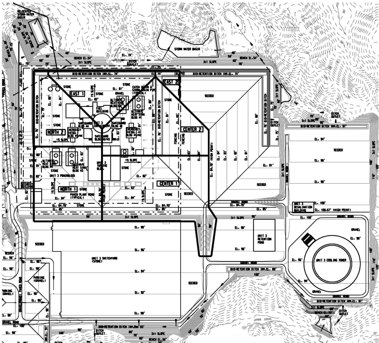
Figure 2.4-7—{CCNP UNIT 3 Sub-Basin Drainage Boundaries}
