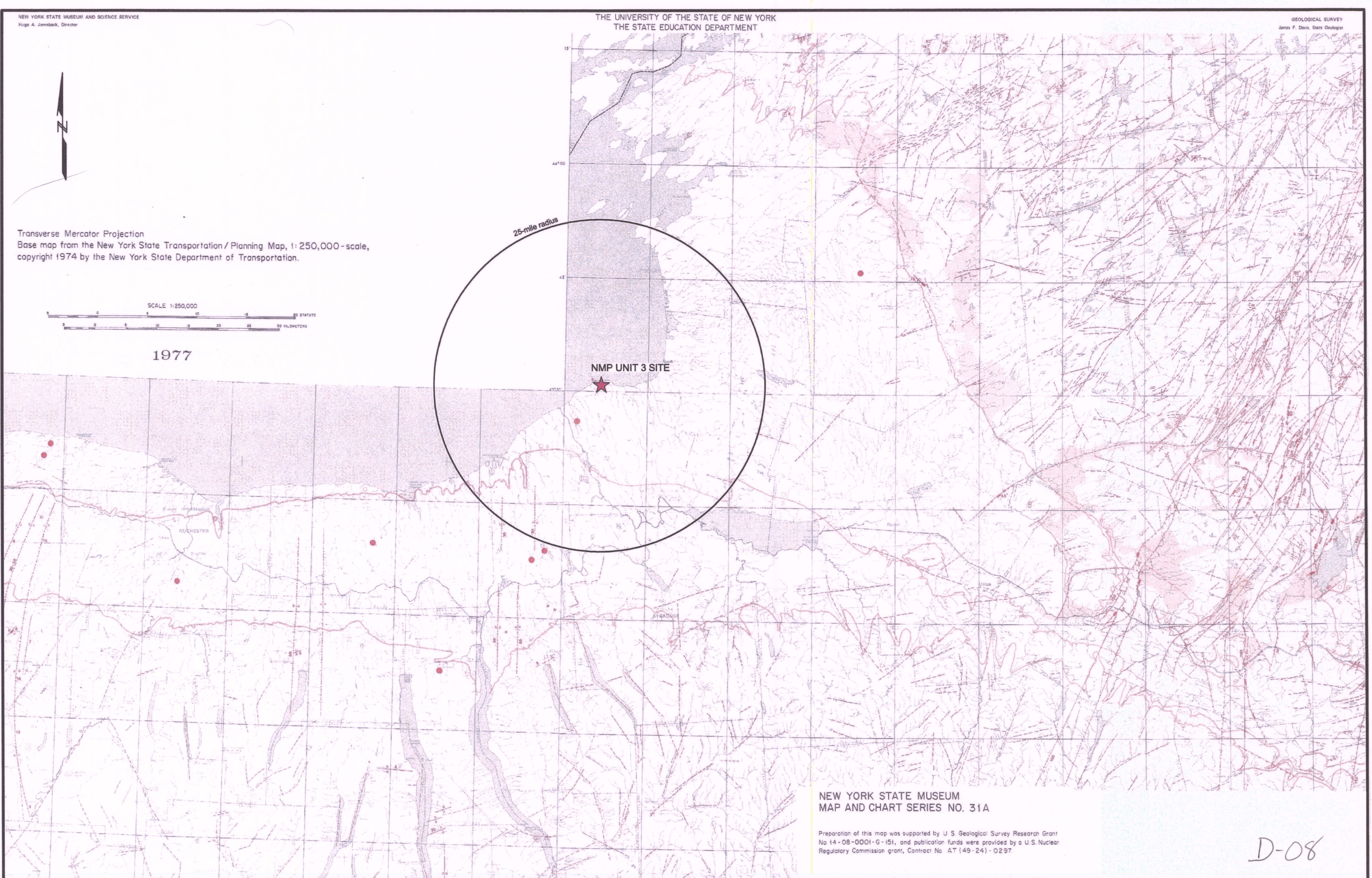
Figure 2.5-36—{Preliminary Brittle Structures Map of NY}
