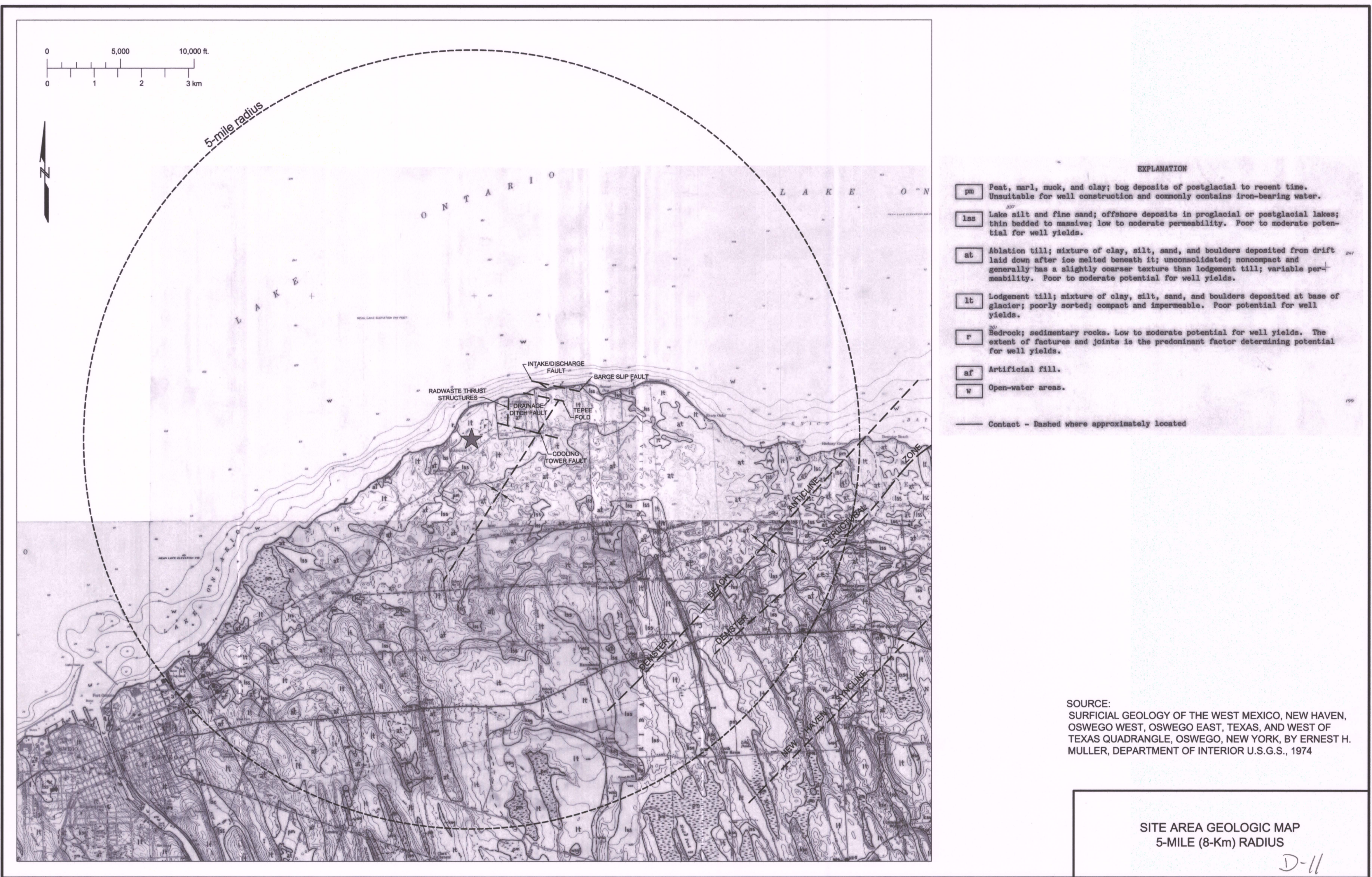
Figure 2.5-55—{Site Area Geologic Map 5-Mile (8-Km) Radius}
