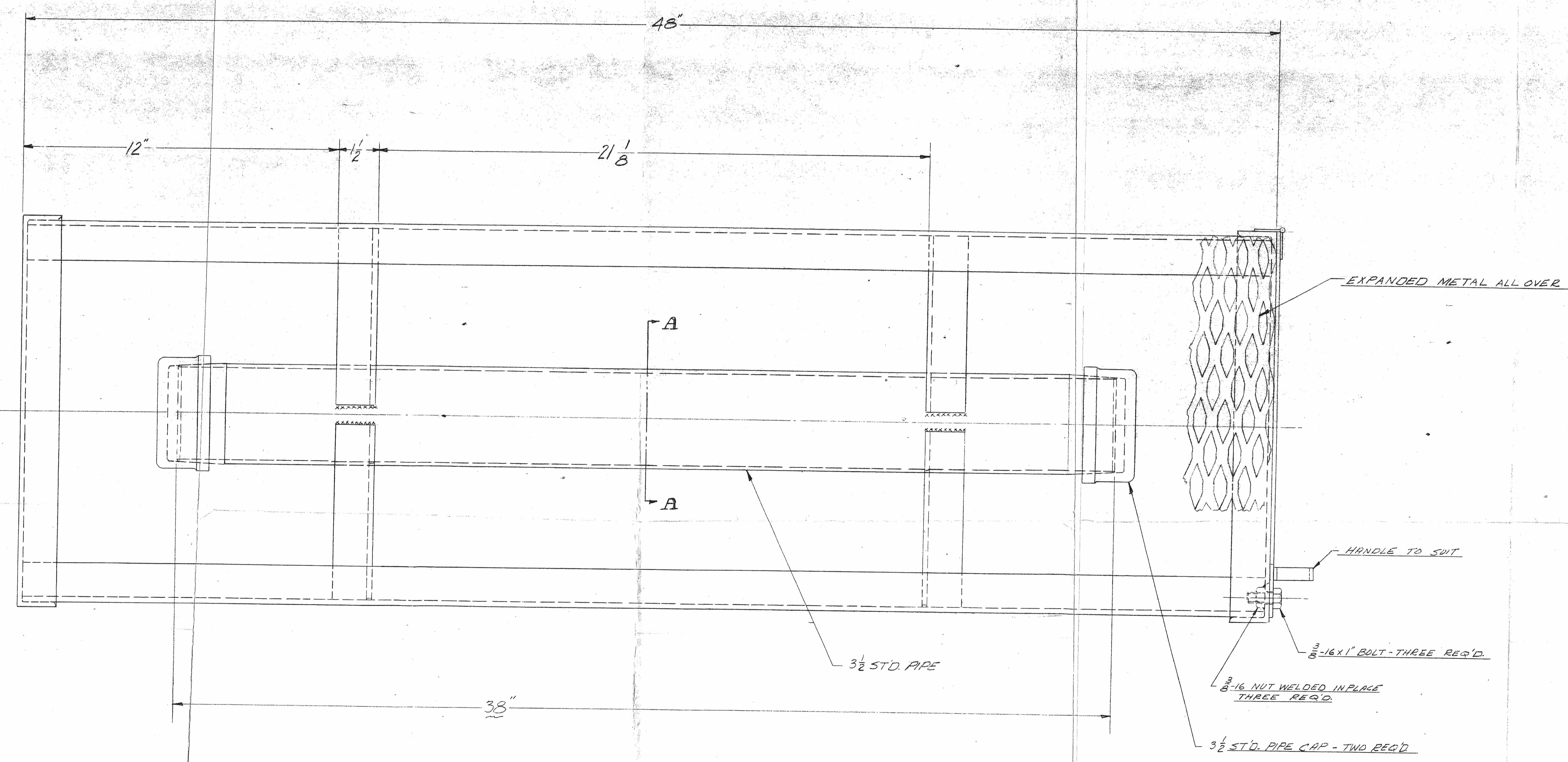
WELDED CONSTRUCTION - ANGLE 1 1/2 x 1 1/2 x 3/16 HALF SIZE
