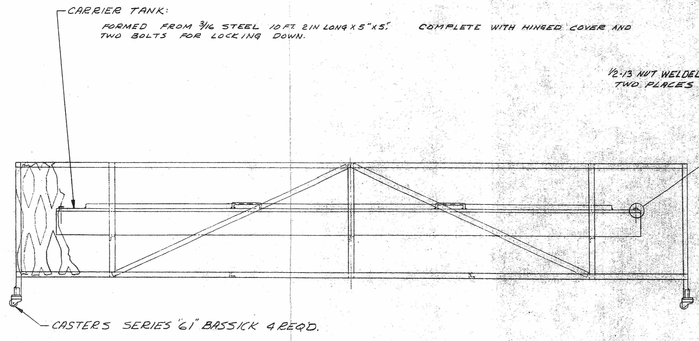
WELDED CONSTRUCTION - SCALE: 1 IN = 1 FT
