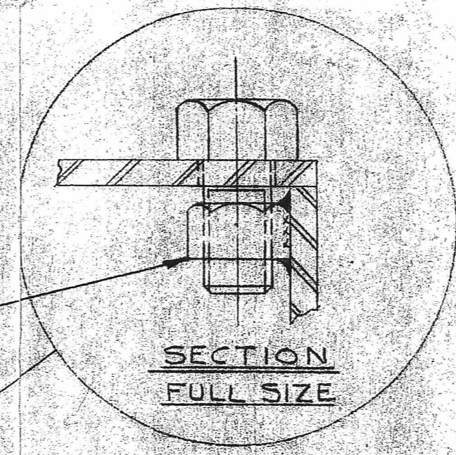
1/2-13 NUT WELDED IN PLACE TWO PLACES
