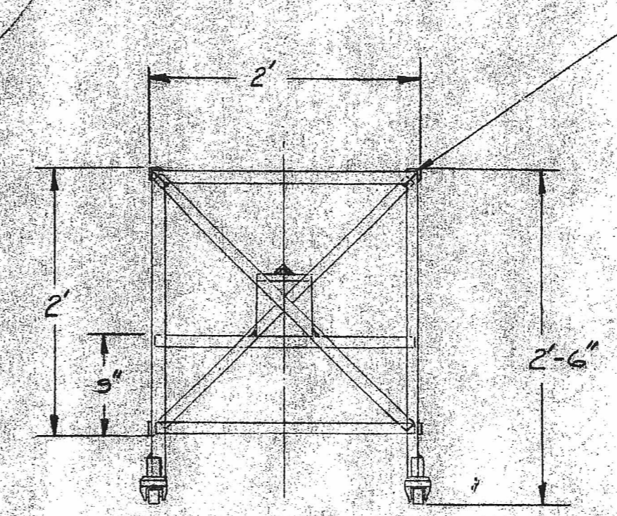
ALL STRUCTURAL MEMBERS ARE 3/4 x 2 x 2 ANGLE IRON
