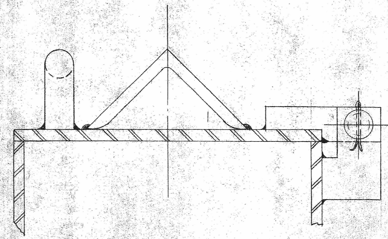
SECTION A-A FULL SIZE
