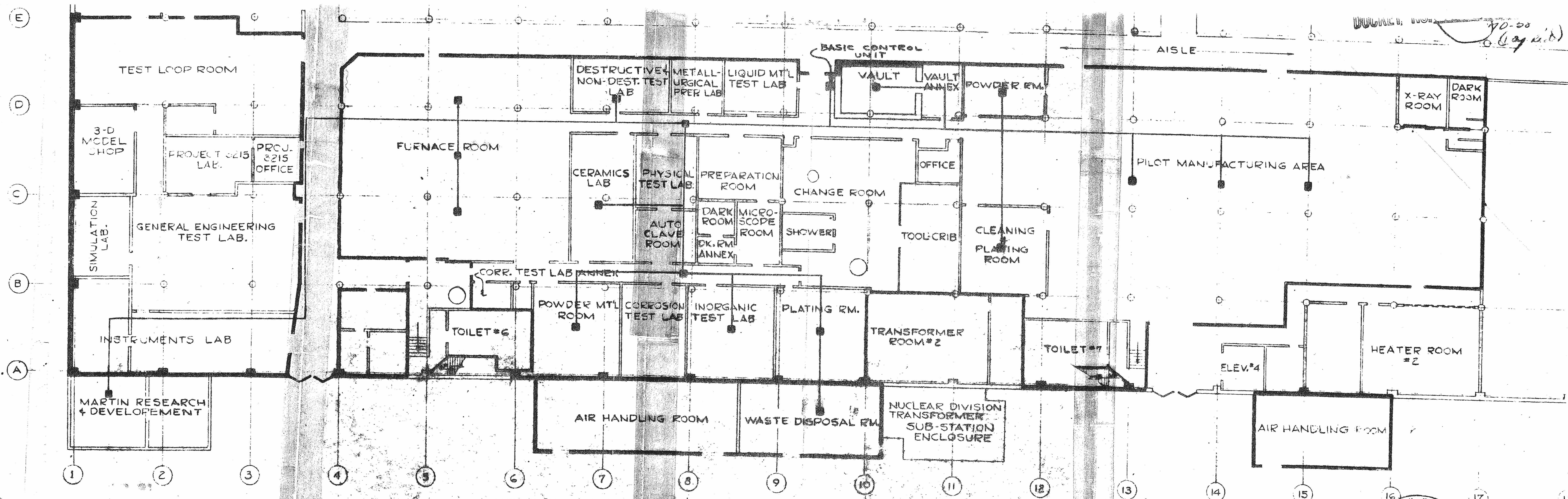
CONDUIT LAYOUT & DETECTOR LOCATION FOR RADIATION MONITOR SYSTEM NUCLEAR AREAS
