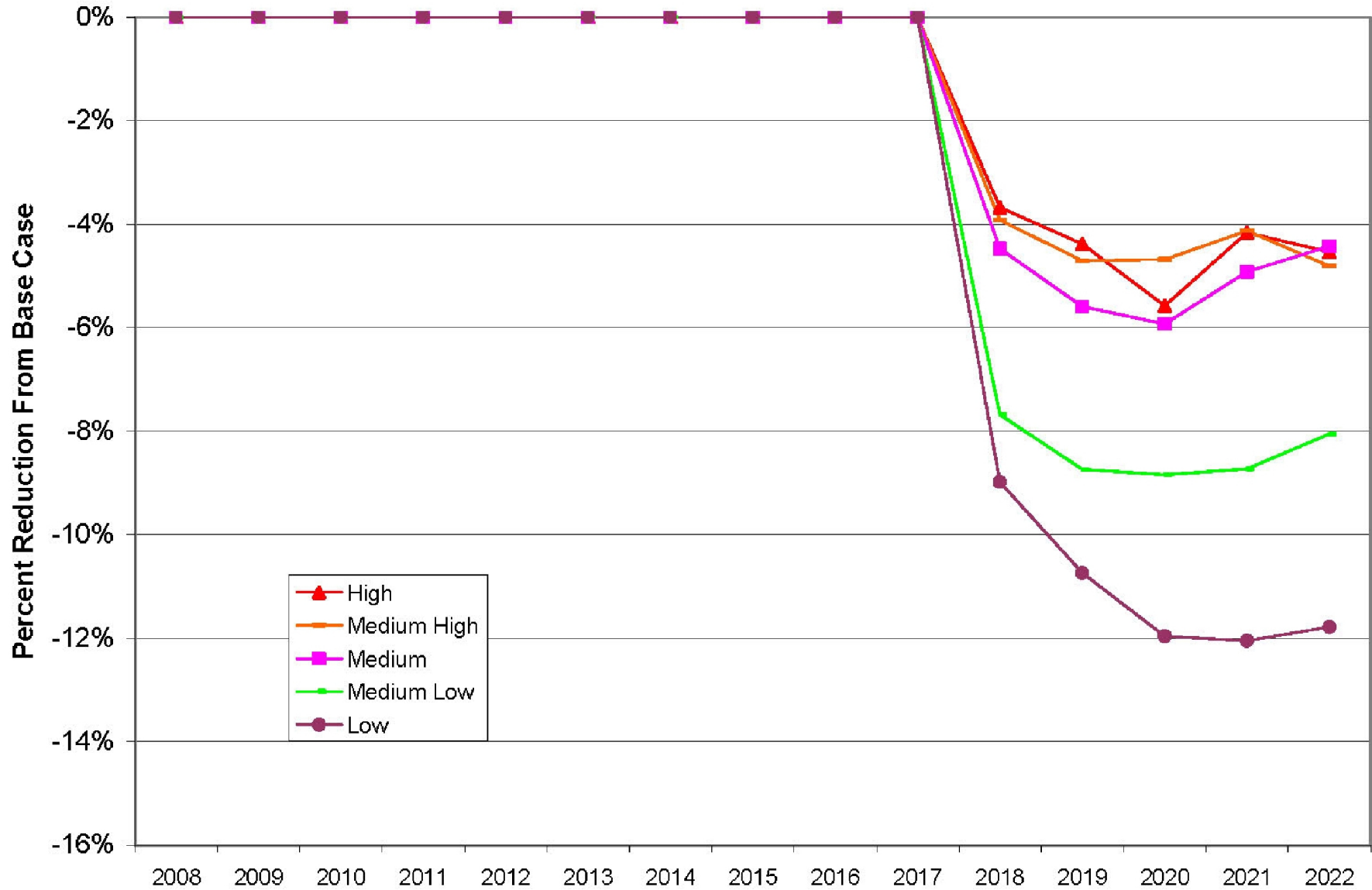
FIGURE 8.4-10 Percent Reduction in TVA SO 2 Emissions due to BLN Unit 3 (2018) and BLN Unit 4 (2019)
