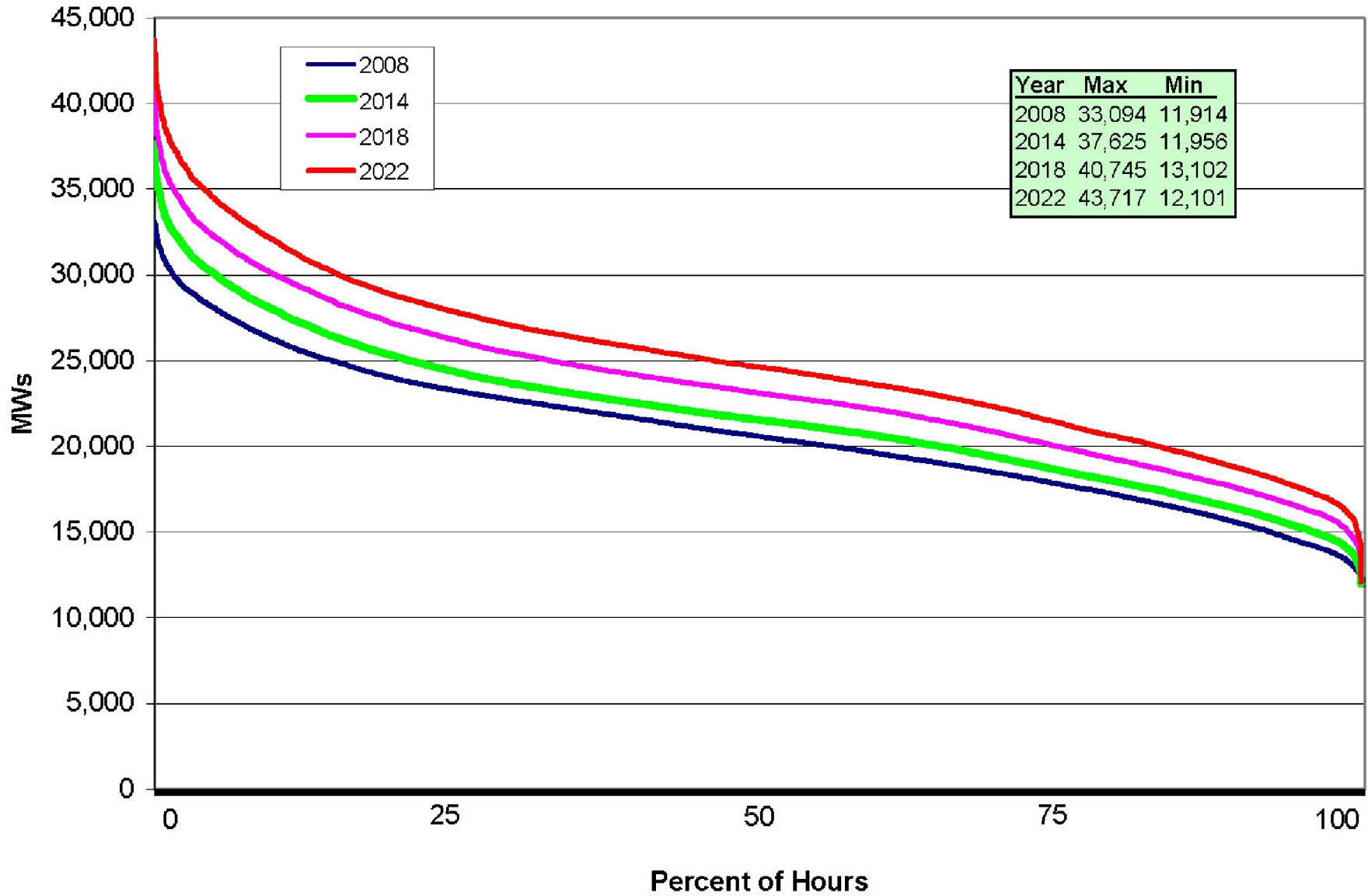
FIGURE 8.2-8 Load Duration Curves for Medium Load Forecast
