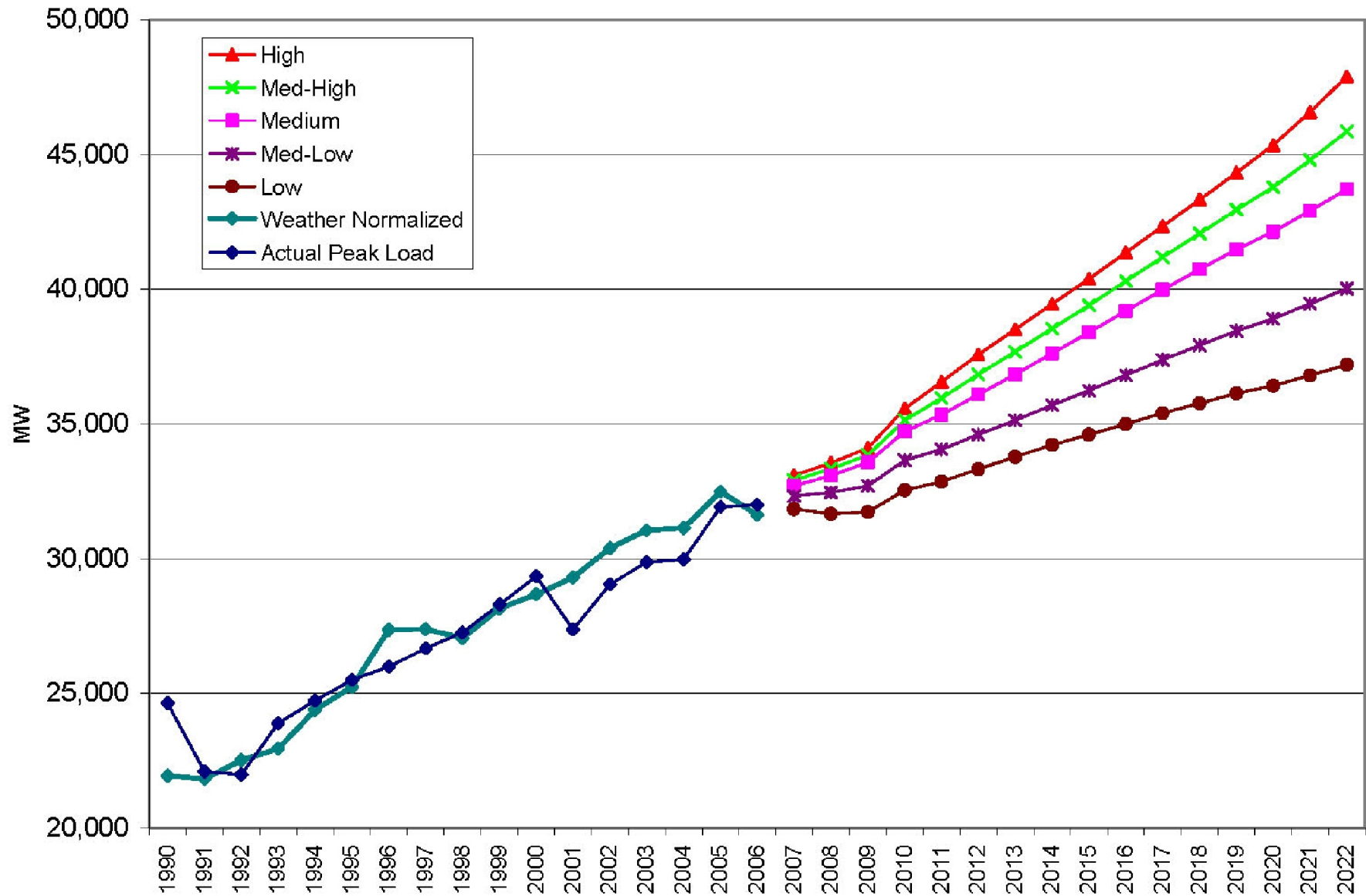
FIGURE 8.2-6 Actual and Forecast Summer Peak Load
