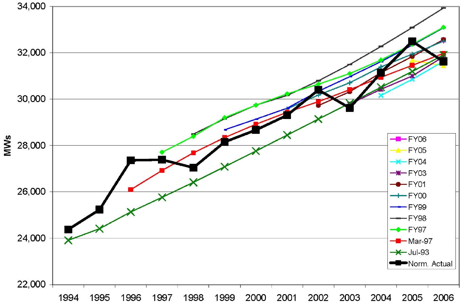
FIGURE 8.2-2 Comparison of Forecast and Actual Summer Peak Loads
